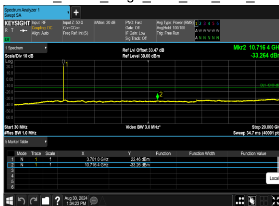
N77(10M)_DFT-s-OFDM_BPSK_Edge_1RB_Left_Low_CH
