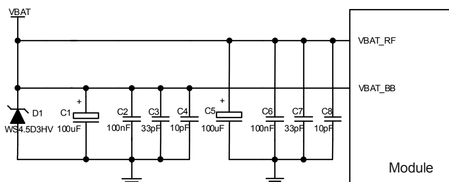
Figure 8: Star Structure of the Power Supply
