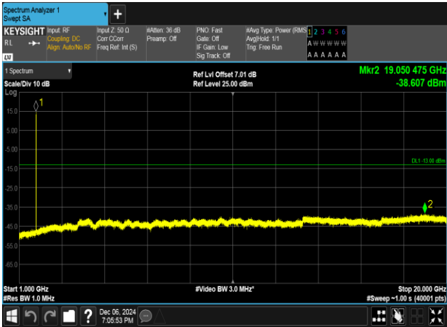
Band4-1513-2-1000~20000MHz-PASS
