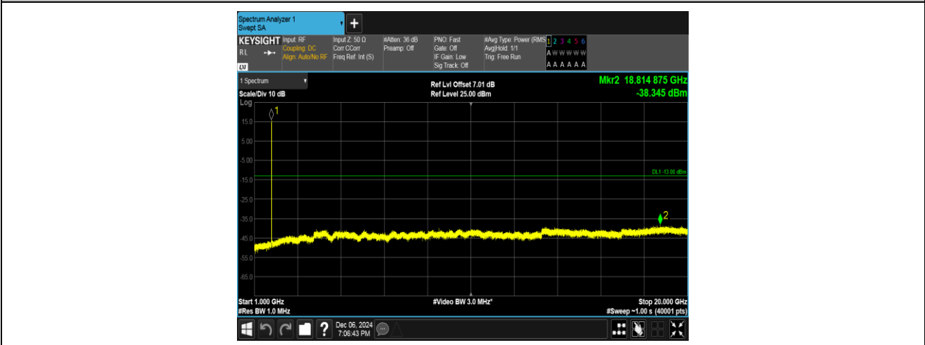
Band4-1312-3-1000~20000MHz-PASS
