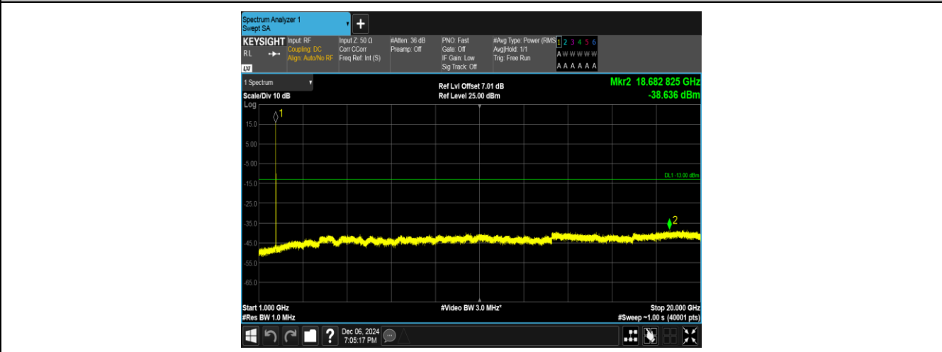
Band4-1413-2-1000~20000MHz-PASS
