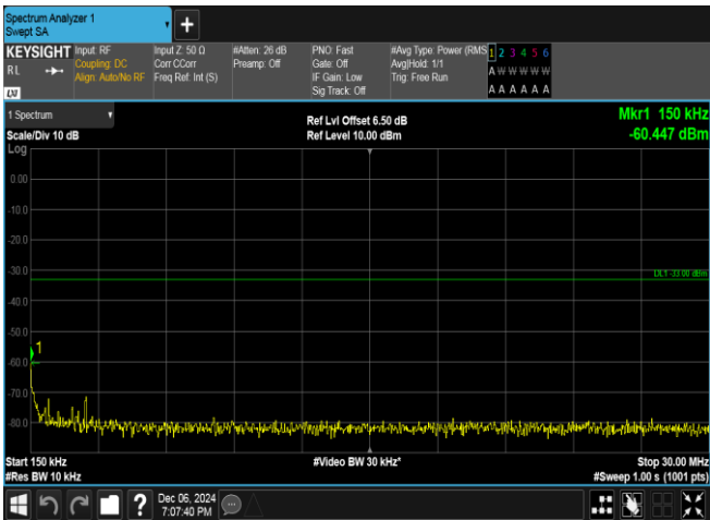
Band4-1513-3-0.15~30MHz-PASS
