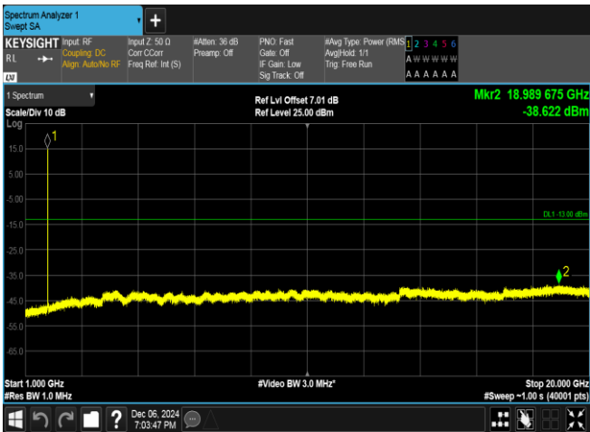
Band4-1513-1-1000~20000MHz-PASS
