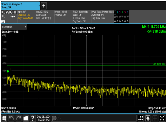
Band4-1513-3-0.009~0.15MHz-PASS
