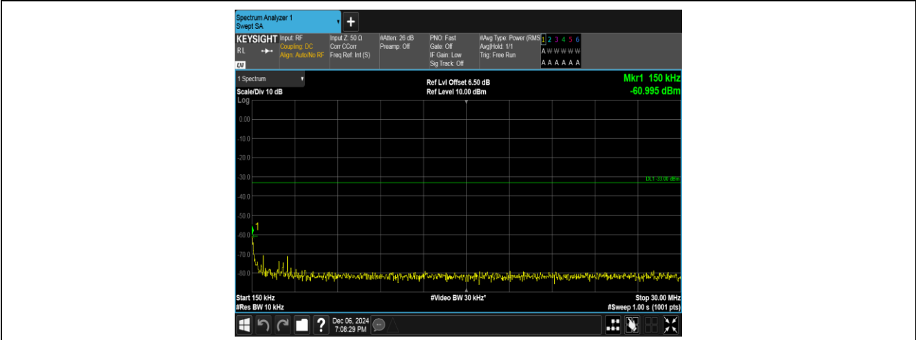
Band4-1312-4-0.15~30MHz-PASS
