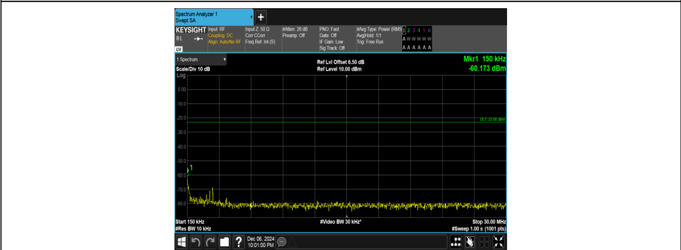
Band5-4182-1-0.15~30MHz-PASS
