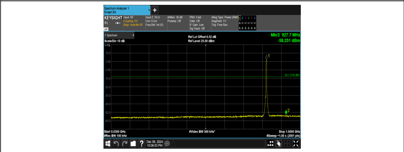
Band5-4132-4-30~1000MHz-PASS
