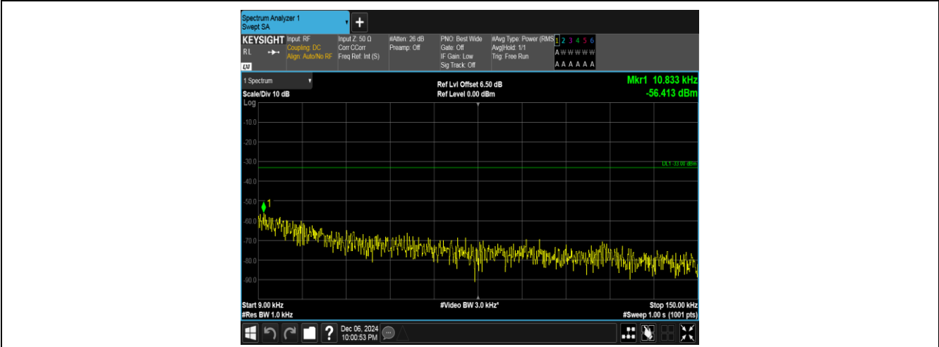
Band5-4182-1-0.009~0.15MHz-PASS
