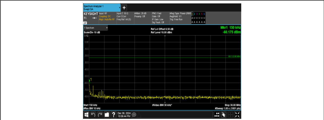
Band5-4132-4-0.15~30MHz-PASS
