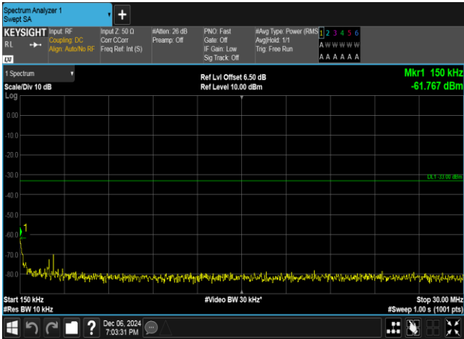
Band4-1513-1-0.15~30MHz-PASS
