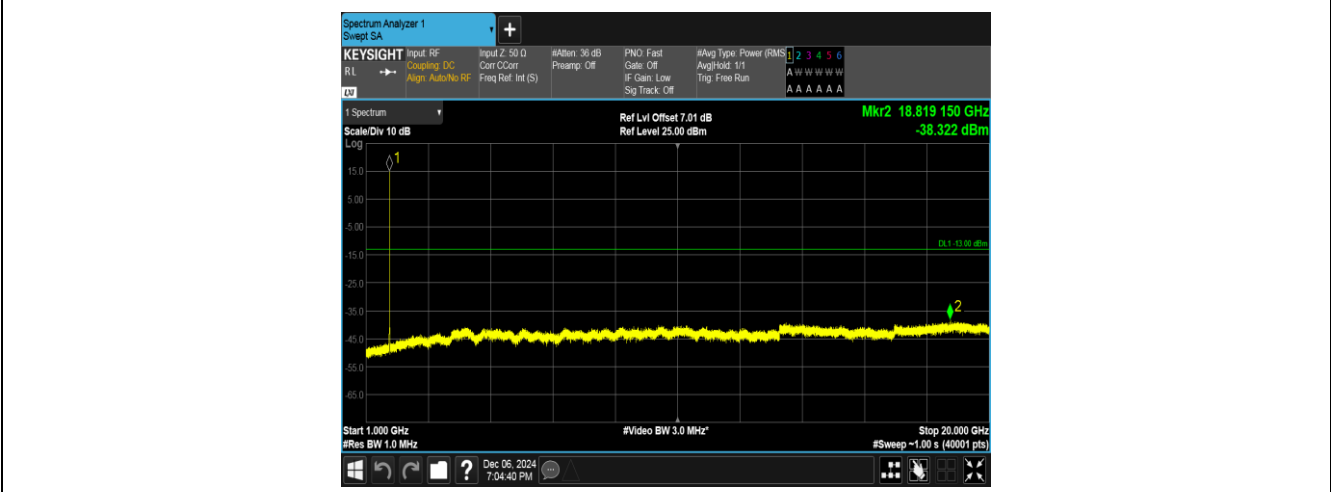
Band4-1312-2-1000~20000MHz-PASS
