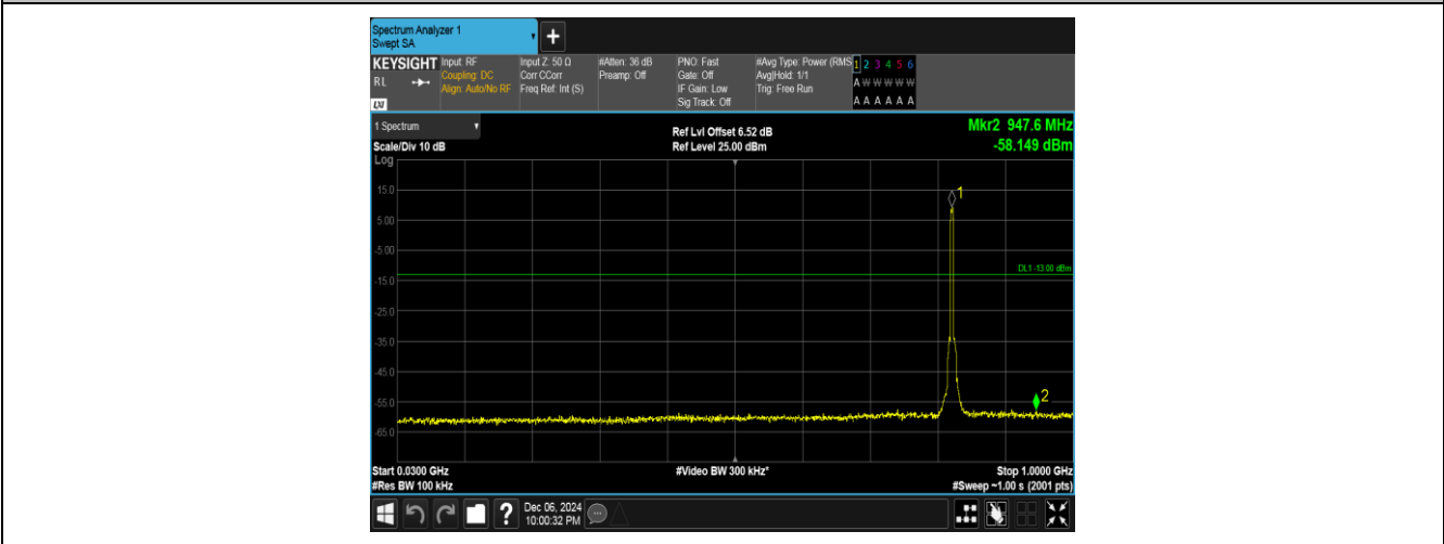
Band5-4132-1-30~1000MHz-PASS
