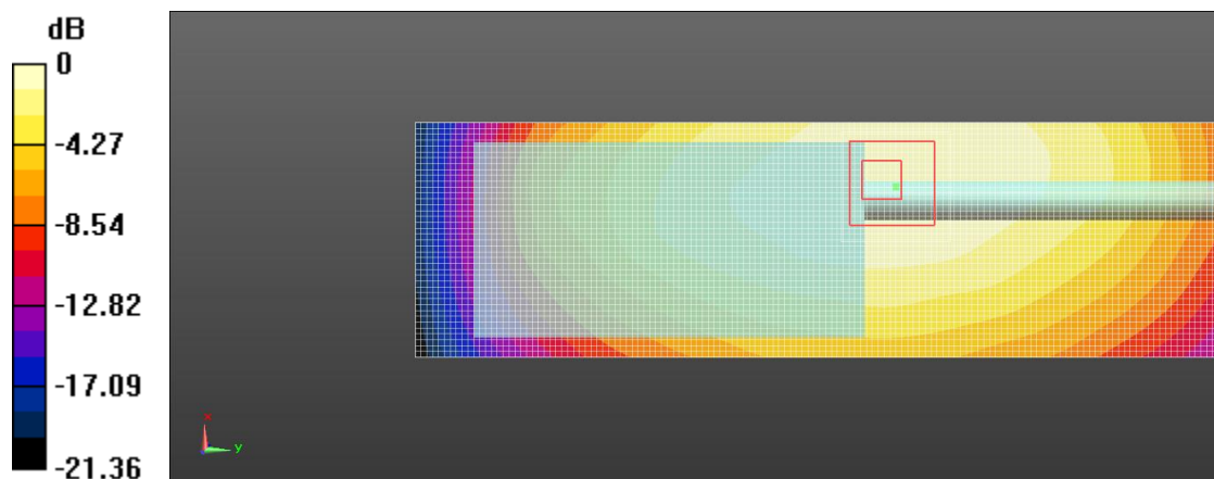
Figure 2: PMR_FM12.5KHz_ Body Worn_0mm
