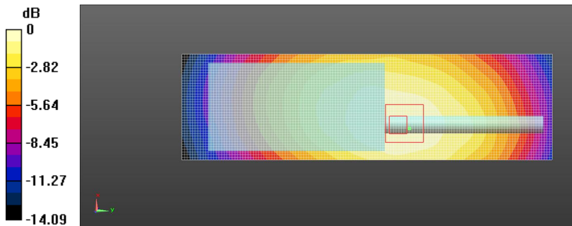
Figure 1: PMR_FM12.5KHz_Face held_25mm
