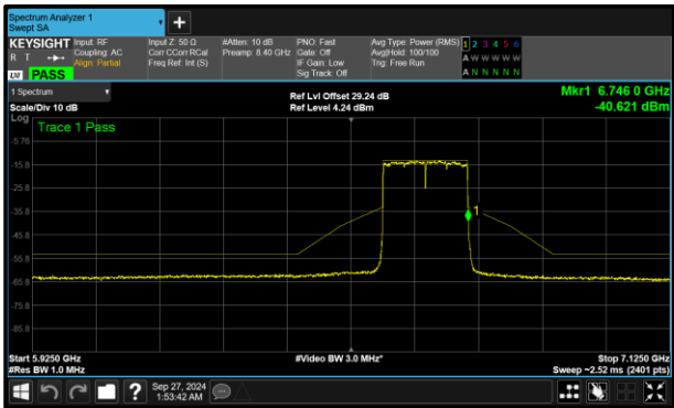
Figure 337 - A (Core 0) 802.11ax HE160 SU VLP 6665 MHz (CH143)
