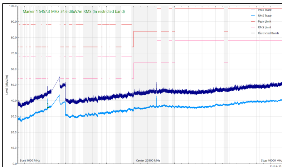
Figure 295 - U-NII-8 - 7115 MHz (CH233), HE20, SU, CDD, Core 0 + Core 1, 1 GHz to 40 GHz, Horizontal
