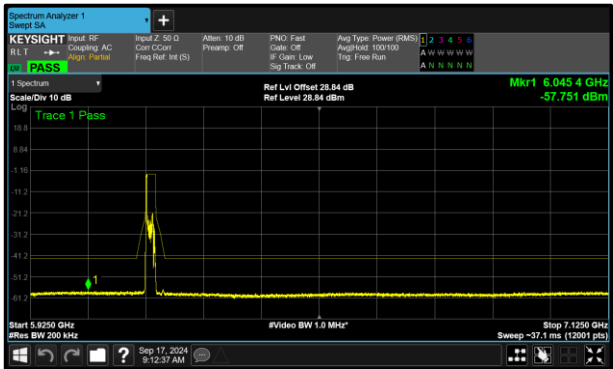
Figure 332 - A (Core 0) 802.11ax HE20 RU26 SP 6175 MHz (CH45)
