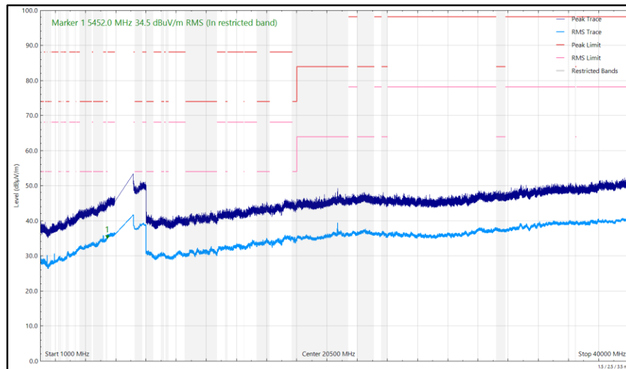
Figure 289 - U-NII-8 - 6895 MHz (CH189), HE20, SU, CDD, Core 0 + Core 1, 1 GHz to 40 GHz, Horizontal
