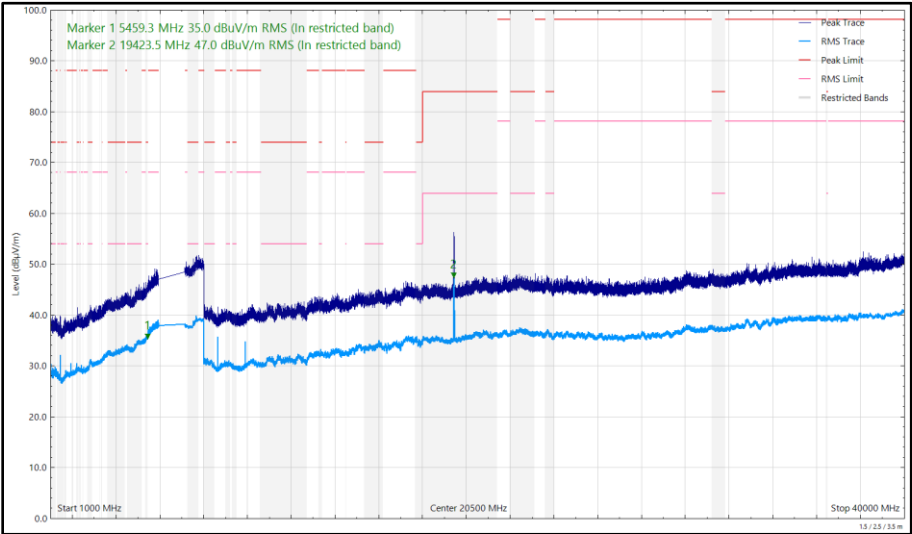
Figure 278 - U-NII-6 - 6475 MHz (CH105), HE20, SU, CDD, Core 0 + Core 1, 1 GHz to 40 GHz, Vertical
