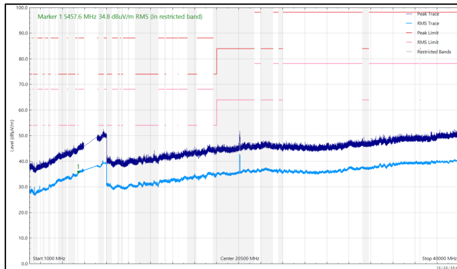
Figure 284 - U-NII-7 - 6695 MHz (CH149), HE20, SU, CDD, Core 0 + Core 1, 1 GHz to 40 GHz, Horizontal
