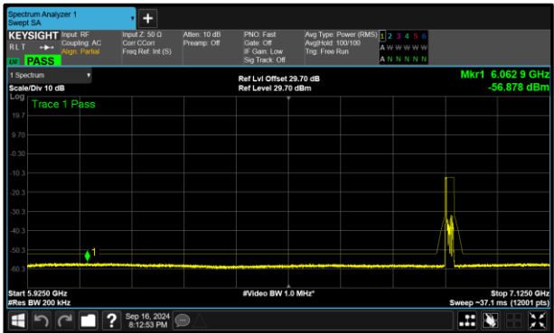
Figure 303 - A (Core 0) 802.11ax HE20 RU26 LPI 6895 MHz (CH189)
