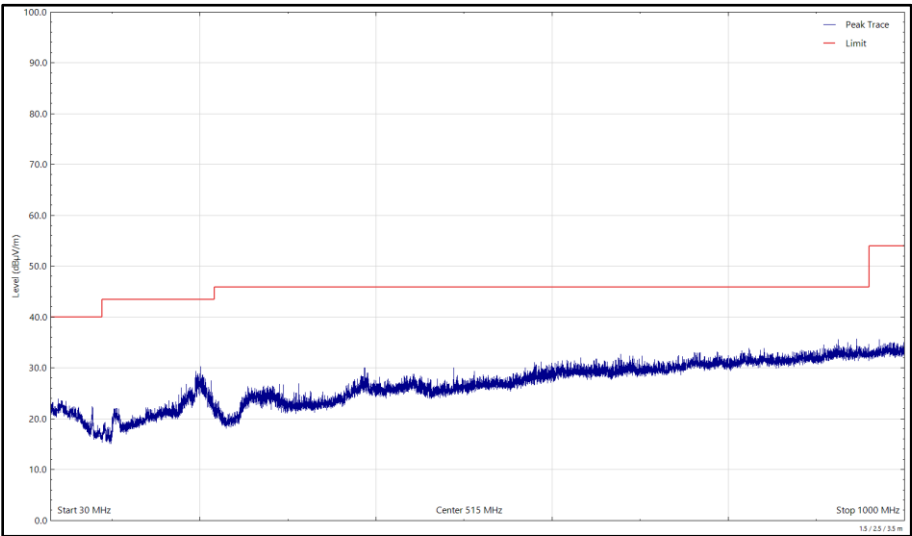
Figure 293 - U-NII-8 - 6995 MHz (CH209), HE20, SU, CDD, Core 0 + Core 1, 30 MHz to 1 GHz, Vertical (Peak)
