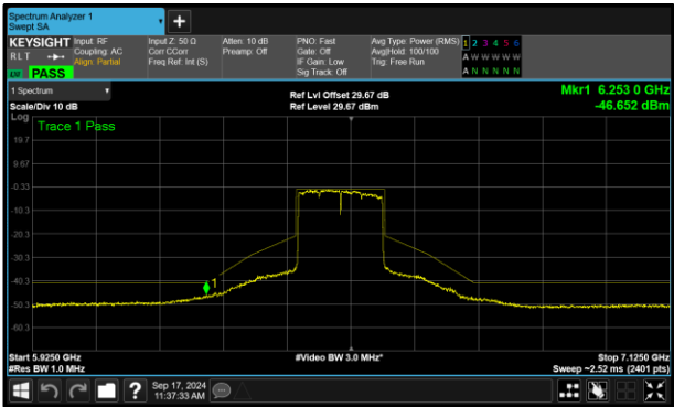
Figure 309 - A (Core 0) 802.11ax HE160 SU SP 6505 MHz (CH111)
