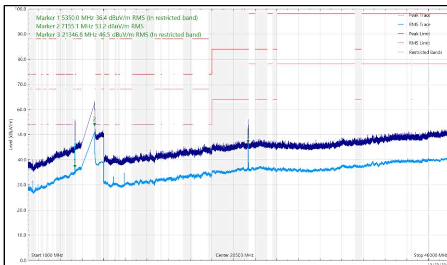
Figure 296 - U-NII-8 - 7115 MHz (CH233), HE20, SU, CDD, Core 0 + Core 1, 1 GHz to 40 GHz, Vertical
