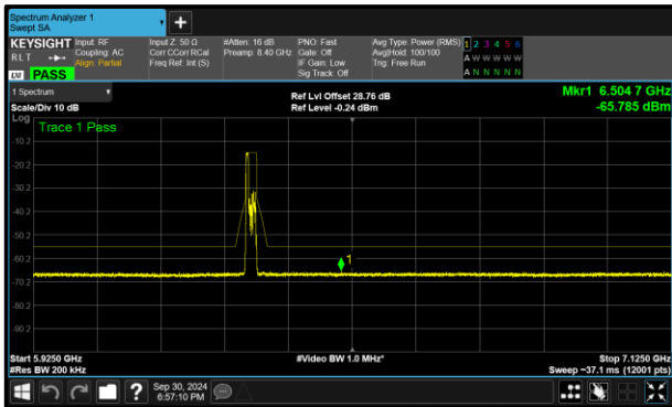
Figure 319 - A (Core 0) 802.11ax HE20 RU52 VLP 6335 MHz (CH77)
