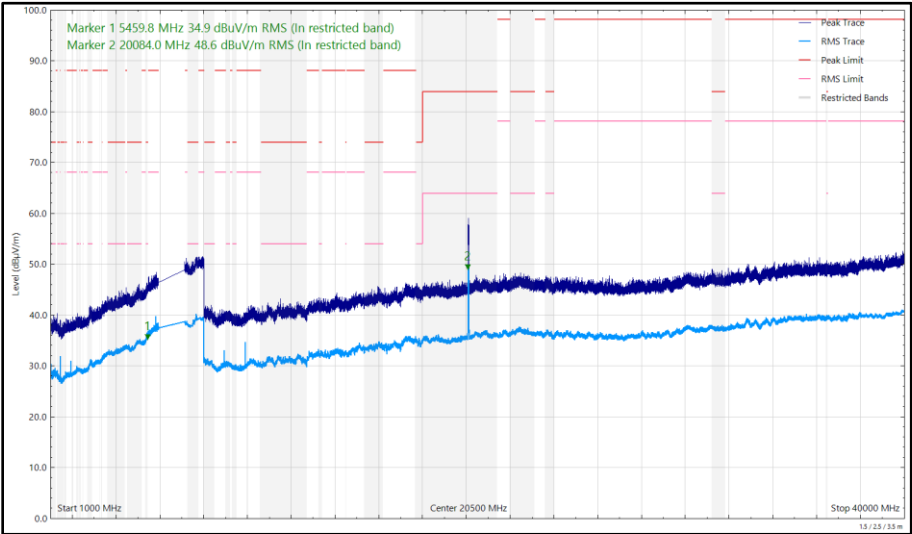
Figure 286 - U-NII-7 - 6695 MHz (CH149), HE20, SU, CDD, Core 0 + Core 1, 1 GHz to 40 GHz, Vertical
