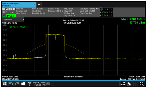
Figure 323 - B (Core 1) 802.11ax HE160 SU LPI 6345 MHz (CH79)
