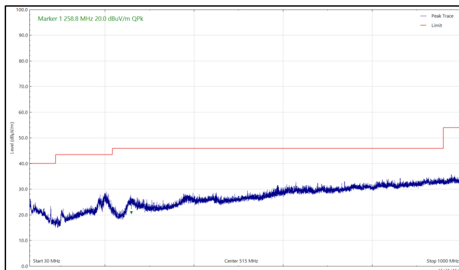
Figure 285 - U-NII-7 - 6695 MHz (CH149), HE20, SU, CDD, Core 0 + Core 1, 30 MHz to 1 GHz, Vertical (Peak)
