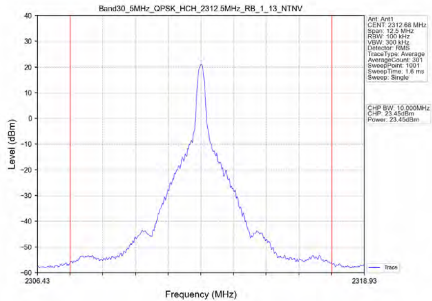
Band30_5MHz_QPSK_HCH_2312.5MHz_RB_1_13_NTNV
