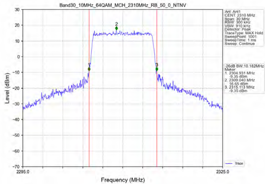
Band30_10MHz_64QAM_MCH_2310MHz_RB_50_0_NTNV
