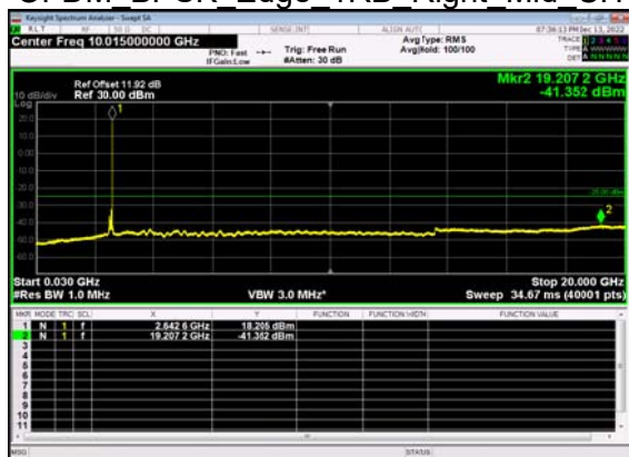
N41(100M)_DFT-s- OFDM BPSK Edge 1RB Right Mid CH
