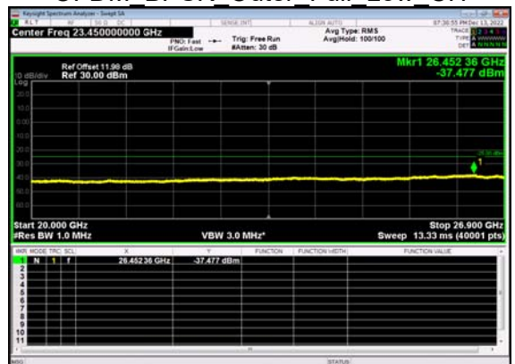
N41(100M)_DFT-s-OFDM BPSK Outer Full Low CH
