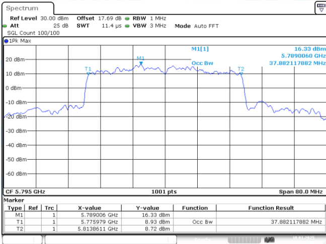
11AX40-CDD-Ant1-5795
