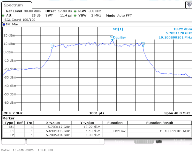
11AX20-CDD-Ant1-5700
