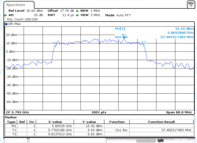
11AX40-CDD-Ant2-5795
