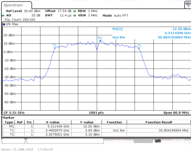
11AC40-CDD-Ant1-5510
