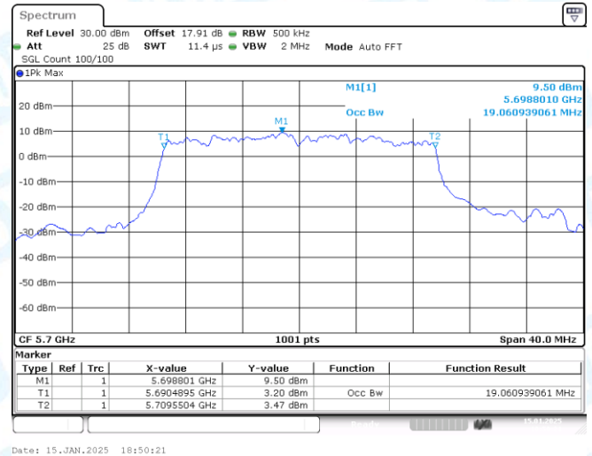
11AX20-CDD-Ant2-5700
