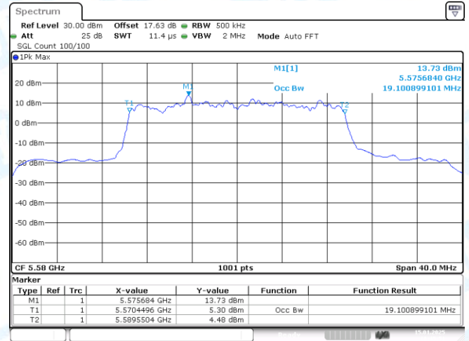
11AX20-CDD-Ant2-5580
