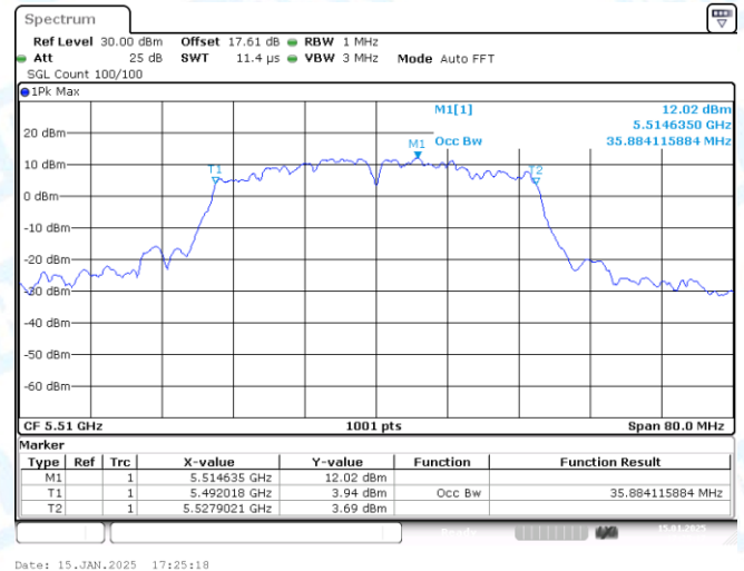
11AC40-CDD-Ant2-5510
