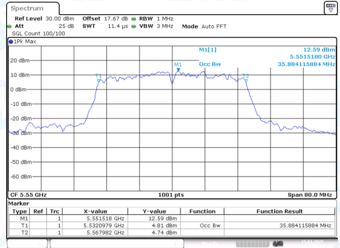
11AC40-CDD-Ant2-5550
