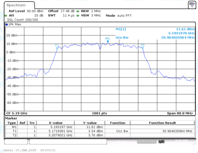
11AC40-CDD-Ant2-5190
