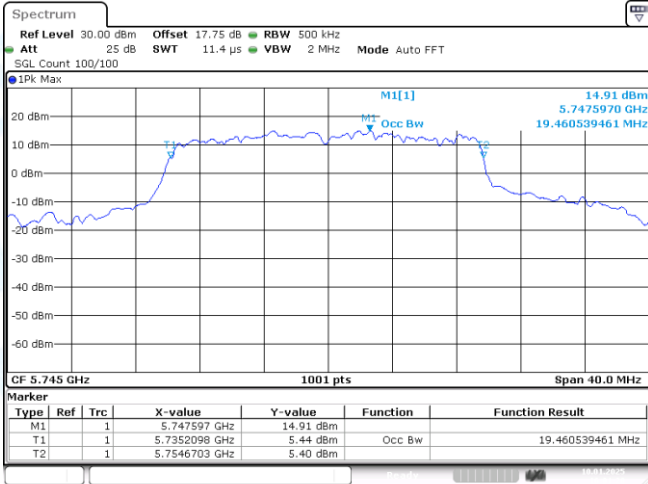
11AX20-CDD-Ant1-5745
