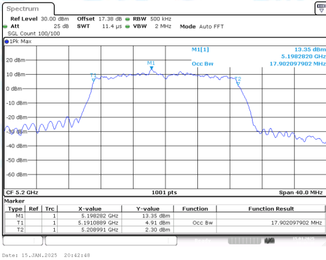
11AC20-CDD-Ant1-5200
