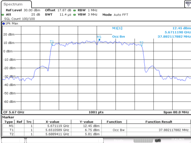
11AX40-CDD-Ant1-5670
