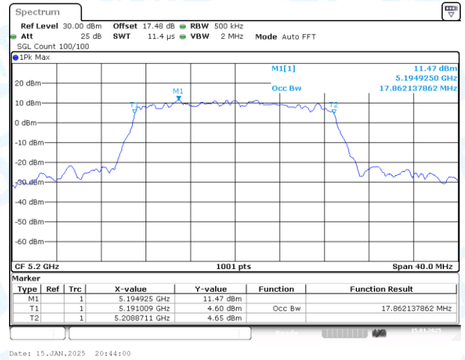
11AC20-CDD-Ant2-5200
