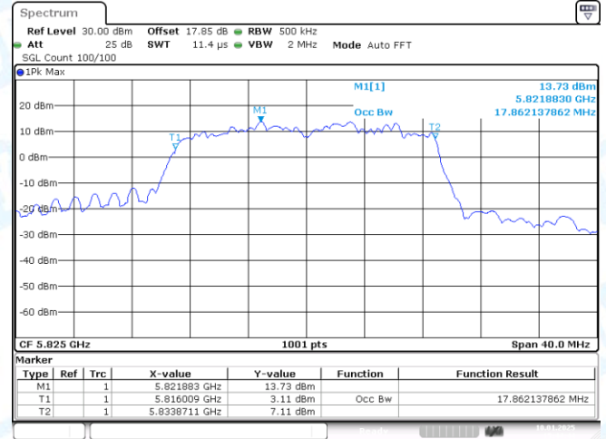
11AC20-CDD-Ant2-5825
