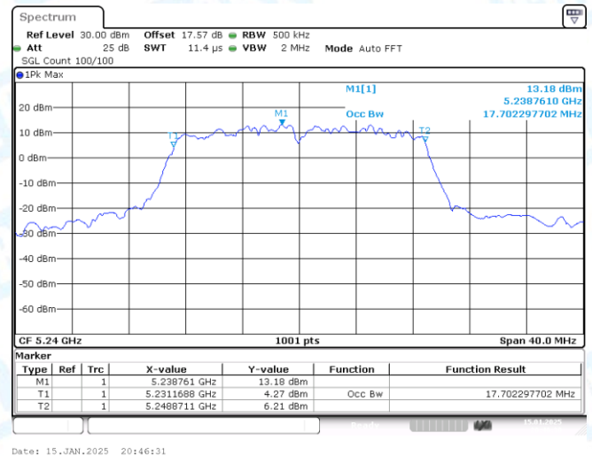
11AC20-CDD-Ant2-5240
