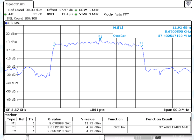
11AX40-CDD-Ant2-5670
