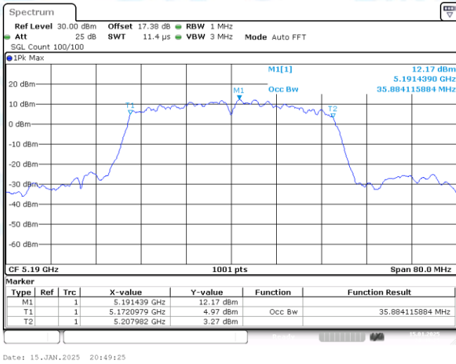
11AC40-CDD-Ant1-5190
