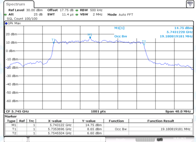
11AX20-CDD-Ant2-5745
