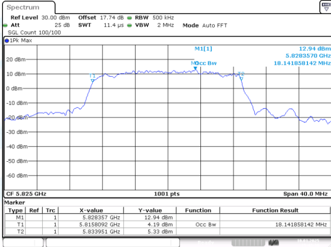
11AC20-CDD-Ant1-5825
