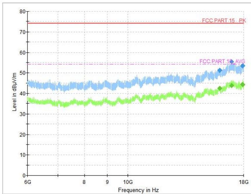
Fig. 59 Radiated Spurious Emission (8DPSK, Ch0, 6GHz ~ 18GHz)
