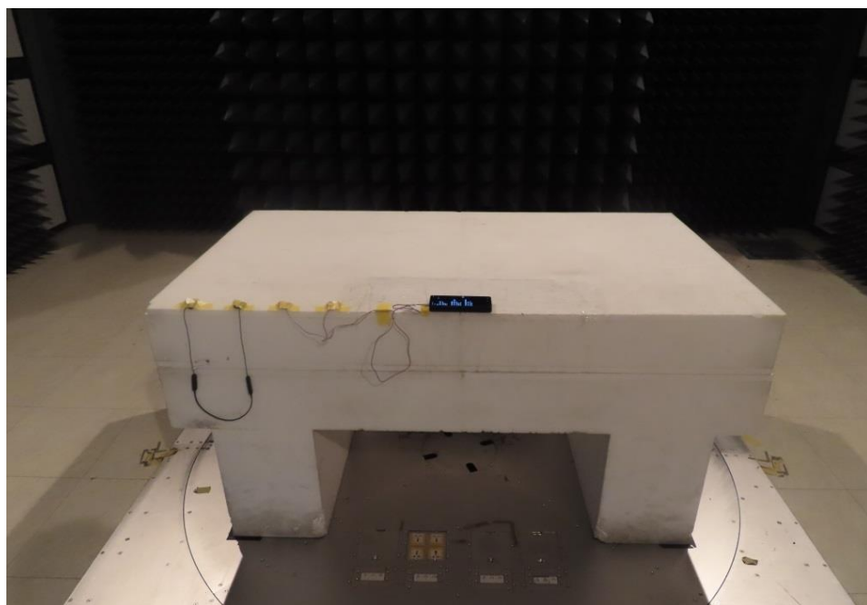
Rear View
