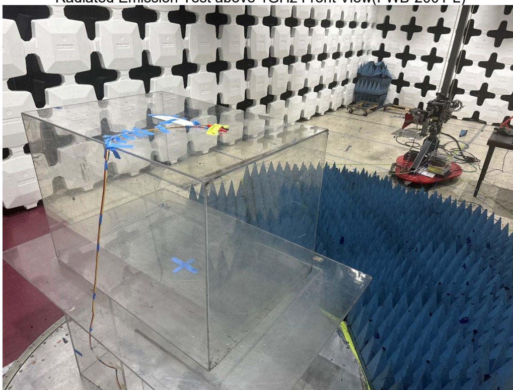
Radiated Emission Test above 1GHz Rear View(FWB-2001-L)
