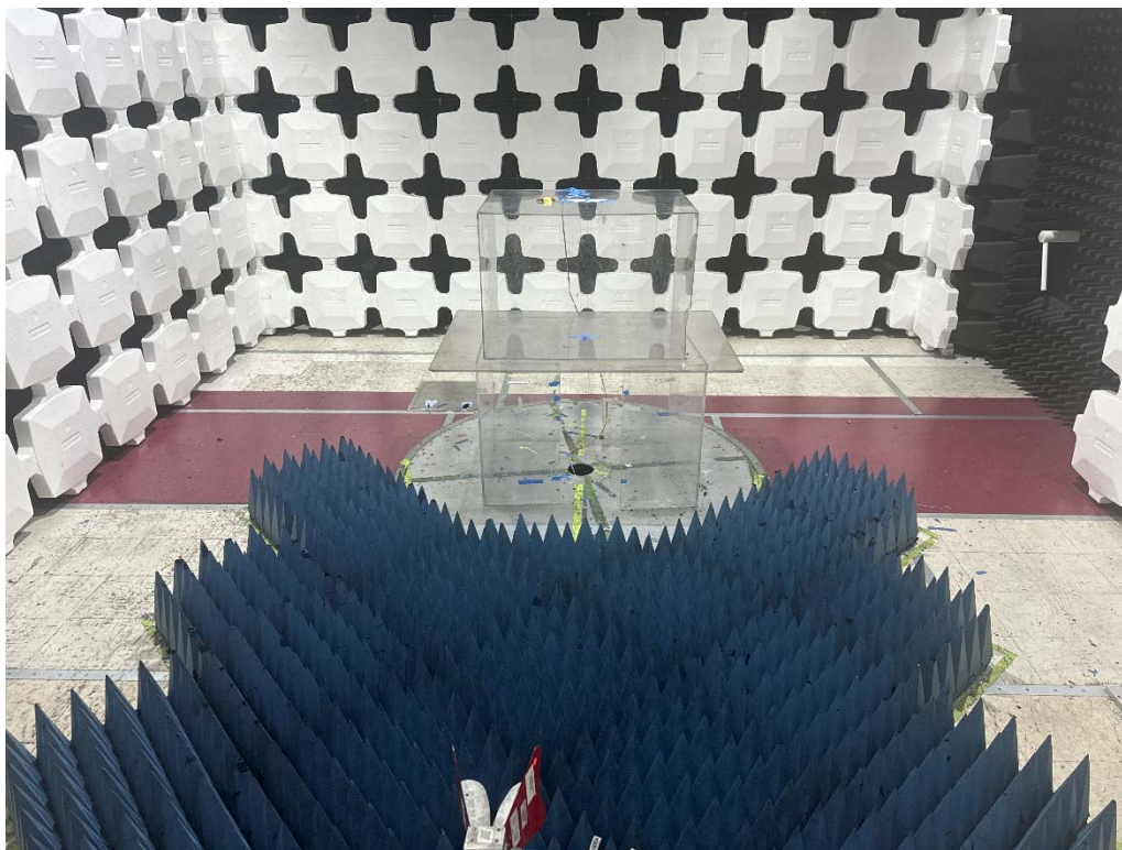
Radiated Emission Test above 1GHz Front View(FWB-2001-L)
