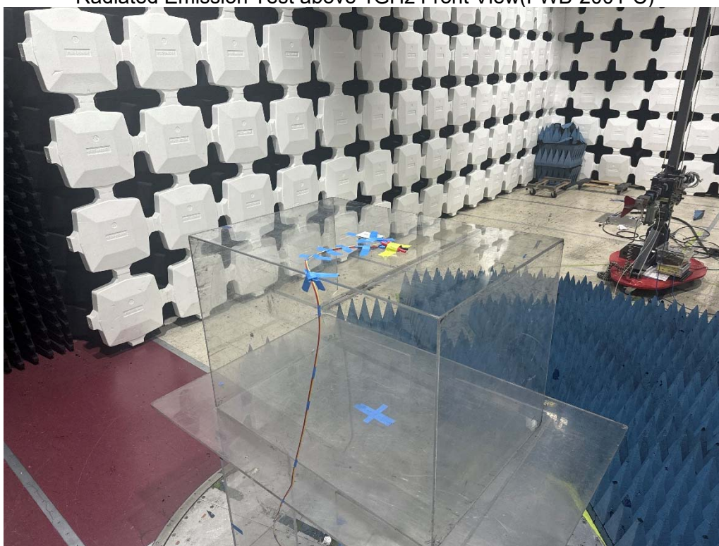
Radiated Emission Test above 1GHz Rear View(FWB-2001-C)
