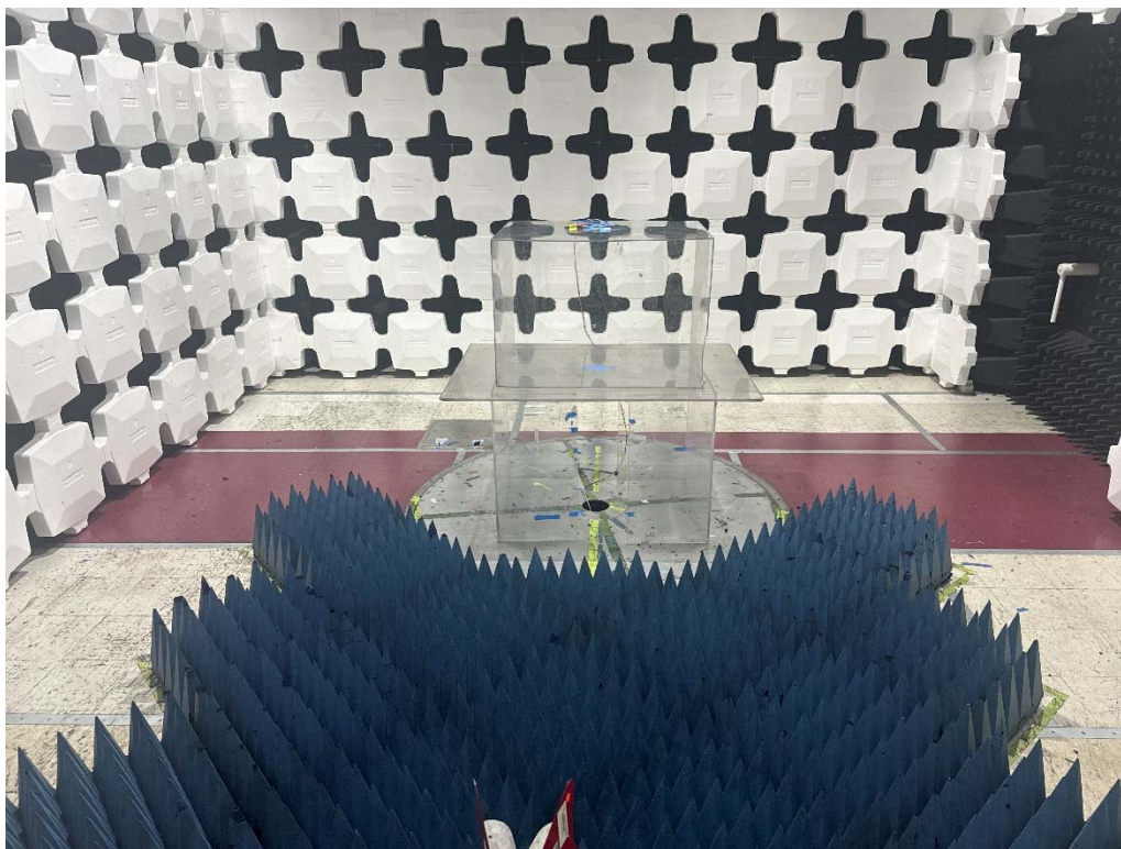
Radiated Emission Test above 1GHz Front View(FWB-2001-C)
