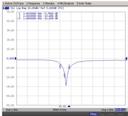
Return Loss
