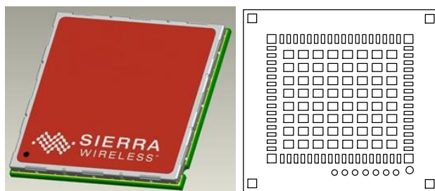
Figure 2. AirPrime HL8549 and HL8549-G Mechanical Overview
