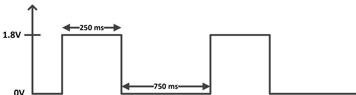
Figure 8. PPS Signal
