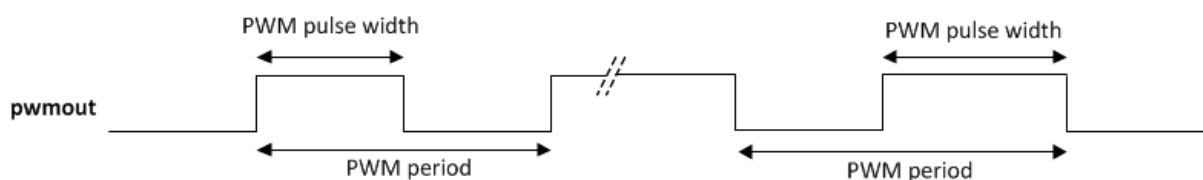
Figure 5. Relative Timing for the PWM Output
