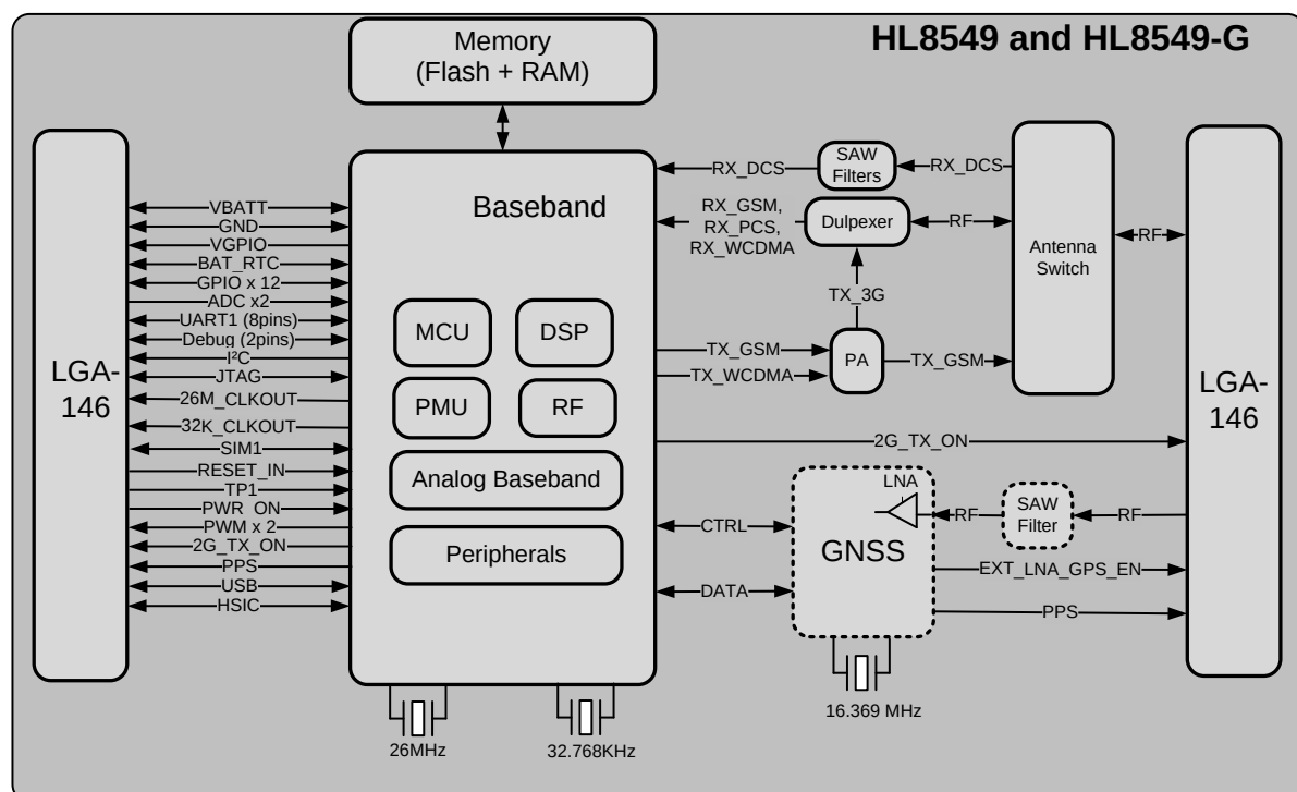
Figure 1. AirPrime HL8549 and HL8549-G Architecture Overview (TBC)
