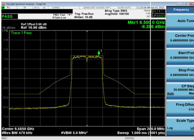
Plot 7-380. In-Band Emission Plot Antenna WF5t (40MHz 802.11ax (UNII Band 6) - Ch. 107, MCS11)
