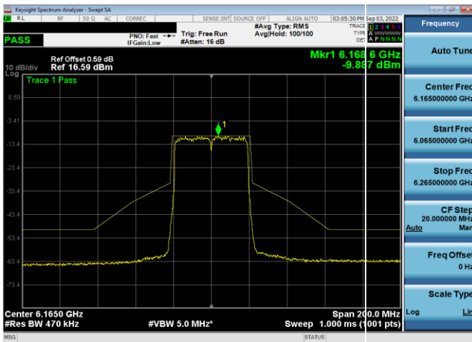
Plot 7-419. In-Band Emission Plot Antenna WF5b (40MHz 802.11ax) – Ch. 43, MCS4)
