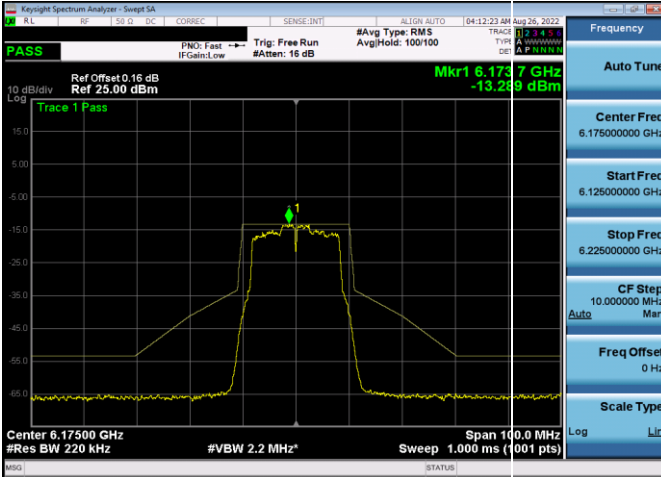
Plot 7-417. In-Band Emission Plot Antenna WF5b (20MHz 802.11a) – Ch. 45, MCS4)
