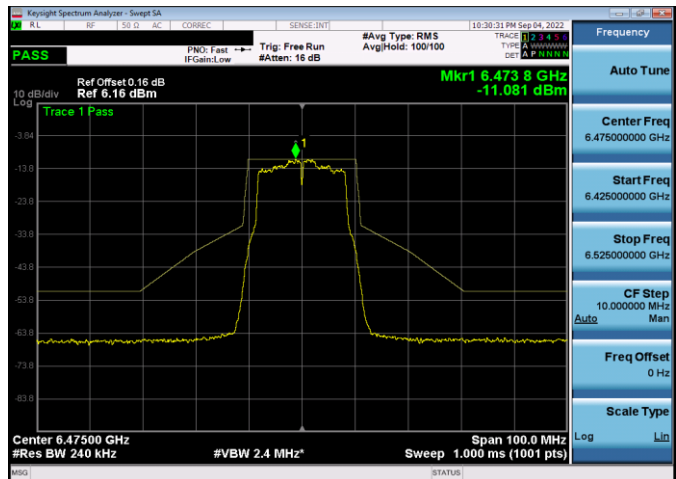
Plot 7-422. In-Band Emission Plot Antenna WF5b (20MHz 802.11a) – Ch. 105, MCS4)
