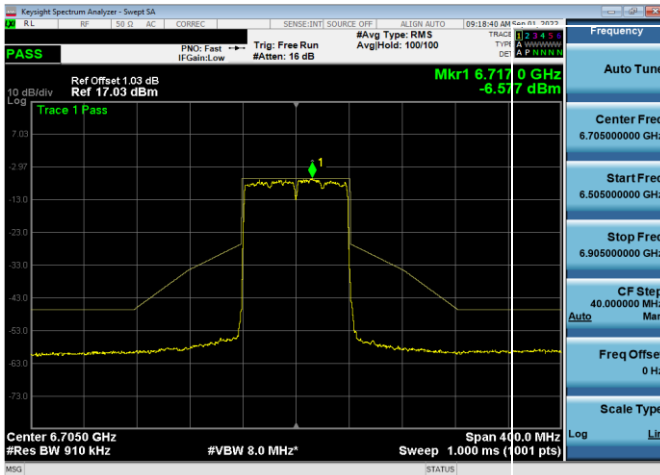
Plot 7-386. In-Band Emission Plot Antenna WI-5t (80MHz 802.11ax (UNII Band 7) – Ch. 151, MCS11)
