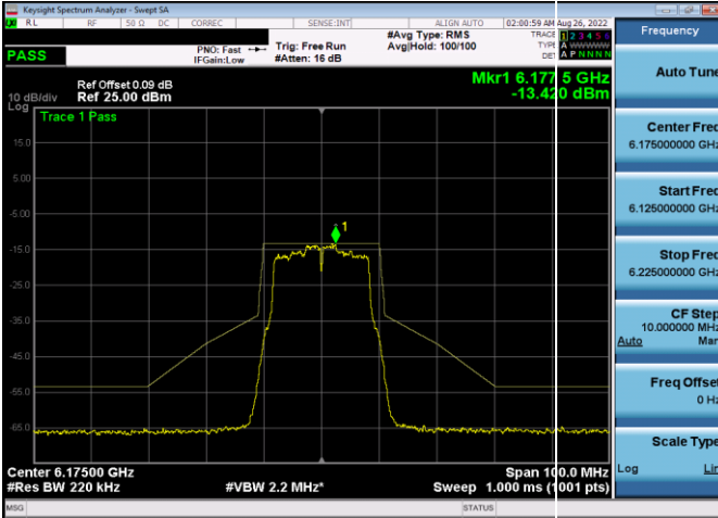
Plot 7-357. In-Band Emission Plot Antenna WF5t (20MHz 802.11a (UNII Band 5) – Ch. 45, MCS4)
