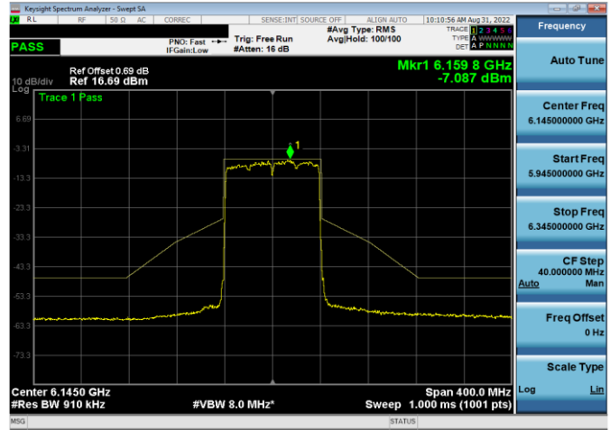
Plot 7-420. In-Band Emission Plot Antenna WF5b (80MHz 802.11ax) – Ch. 39, MCS4)
