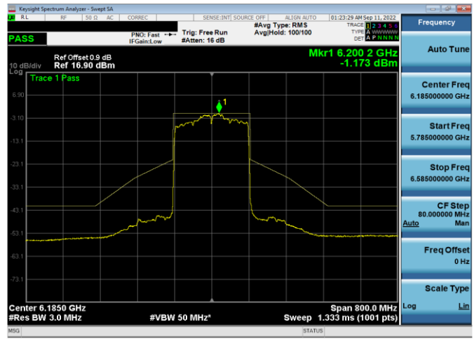
Plot 7-421. In-Band Emission Plot Antenna WF5b (160MHz 802.11ax) – Ch. 47, MCS4)
