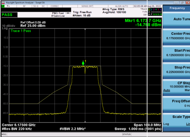
Plot 7-373. In-Band Emission Plot Antenna WF5t (20MHz 802.11a) (UNII Band 5) – Ch. 45, MCS11)
