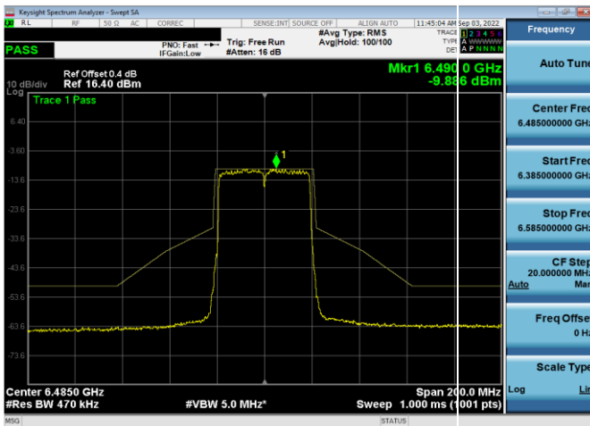
Plot 7-364. In-Band Emission Plot Antenna WF5t (40MHz 802.11ax (UNII Band 6) – Ch. 107, MCS4)
