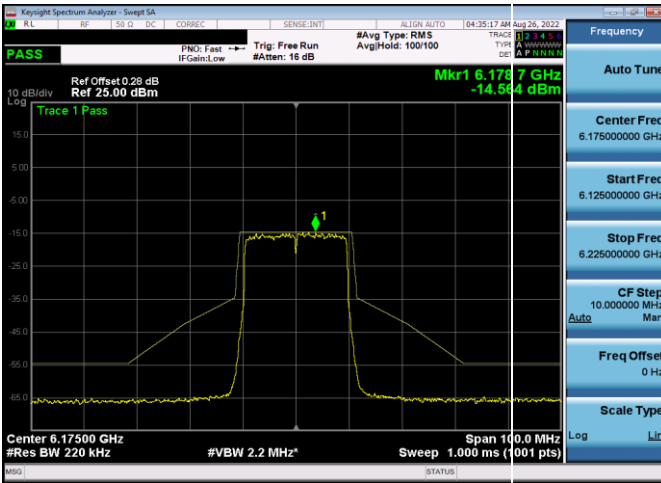
Plot 7-418. In-Band Emission Plot Antenna WF5b (20MHz 802.11ax) – Ch. 45, MCS4)
