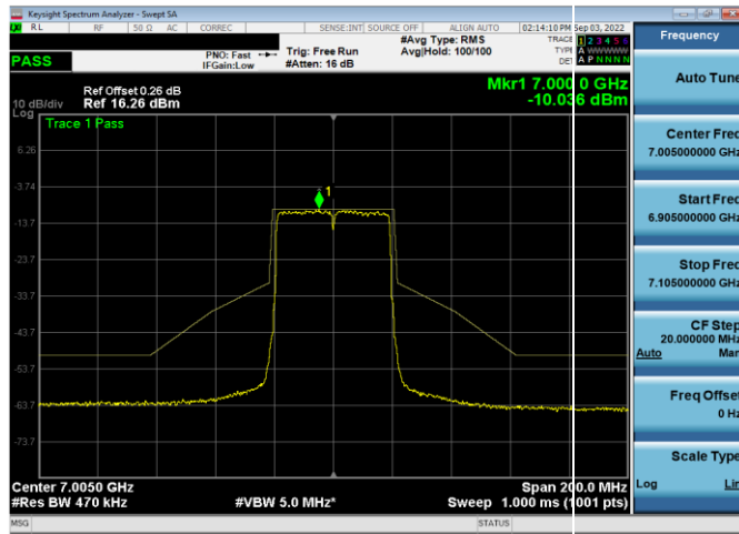
Plot 7-354. In-Band Emission Plot Antenna WF5t (40MHz 802.11ax (UNII Band 8) – Ch. 211, MCS2)
