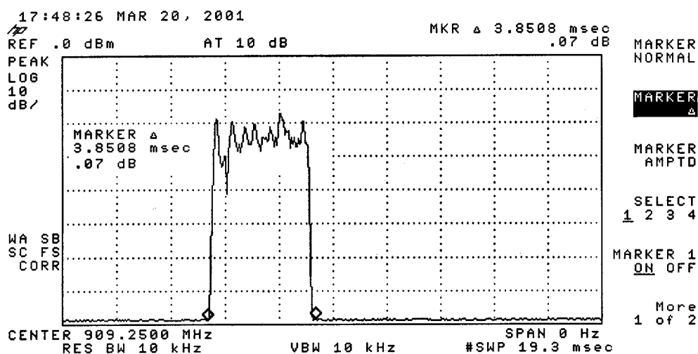
Plot 2. Master Transmit Time on a Given Channel in the Pseudorandom Hop Sequence with no Data on RS-232 port
