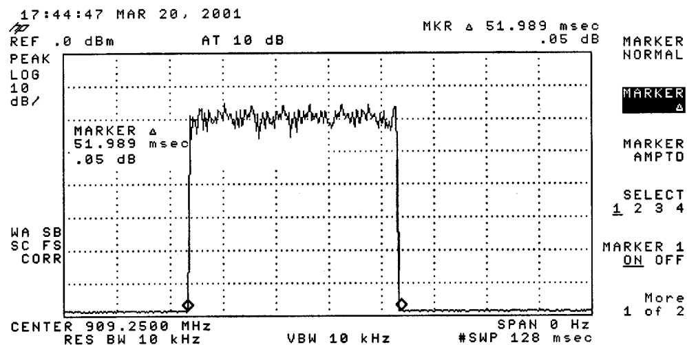
Plot 1. Master Transmit Time on a Given Channel in the Pseudorandom Hop Sequence with Data on RS-232 port
