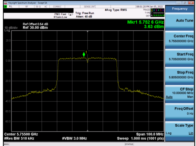
Plot 7-214. PSD Antenna WF8 (40MHz BW 802.11ax(SU) - Ch. 151, MCS5)
