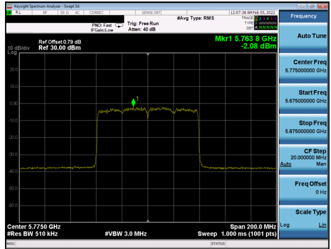
Plot 7-216. PSD Antenna WF8 (80MHz BW 802.11ax(SU) - Ch. 155, MCS5)
