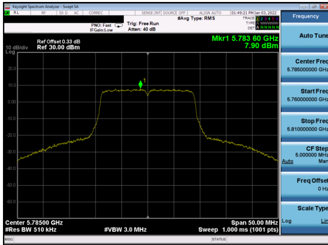
Plot 7-211. PSD Antenna WF8 (20MHz BW 802.11n - Ch. 157, MCS5)
