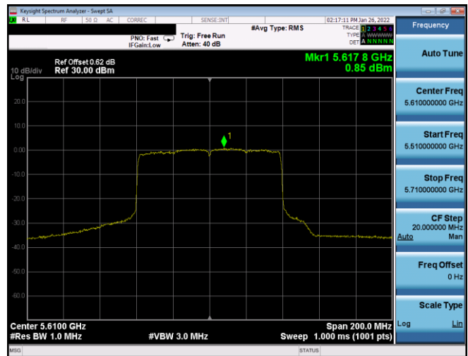
Plot 7-180. PSD Antenna WF8 (80MHz BW 802.11ax(SU) – Ch. 122, MCS3)
