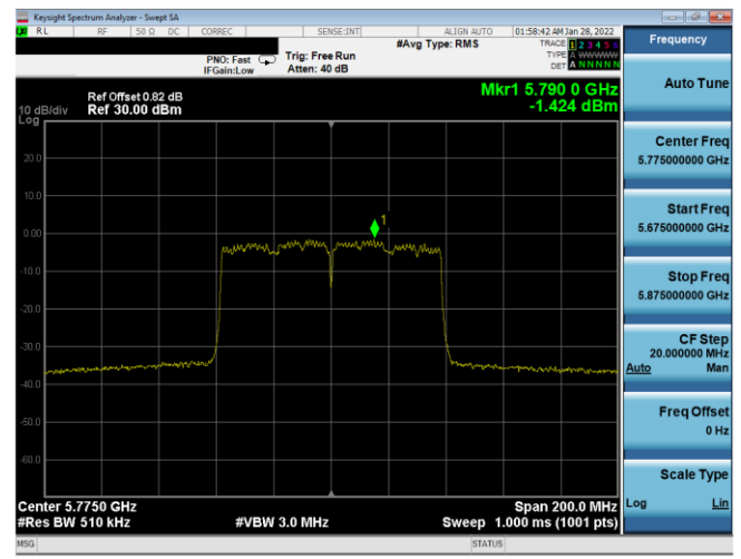
Plot 7-215. PSD Antenna WF8 (80MHz BW 802.11ac - Ch. 155, MCS5)
