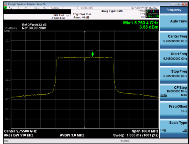
Plot 7-202. PSD Antenna WF8 (40MHz BW 802.11ax(SU) - Ch. 151, MCS0)
