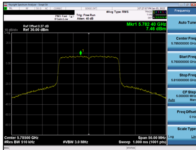
Plot 7-212. PSD Antenna WF8 (20MHz BW 802.11ax(SU) - Ch. 157, MCS5)
