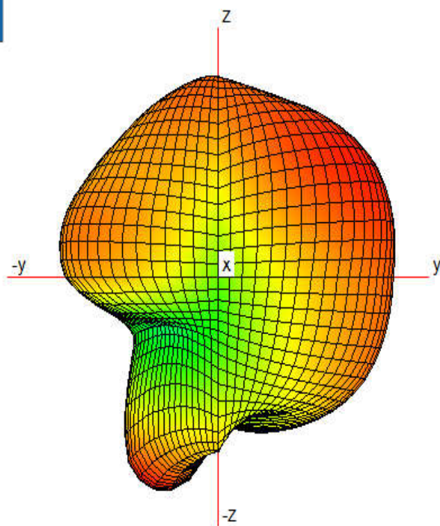
WIFI 5800MHz
