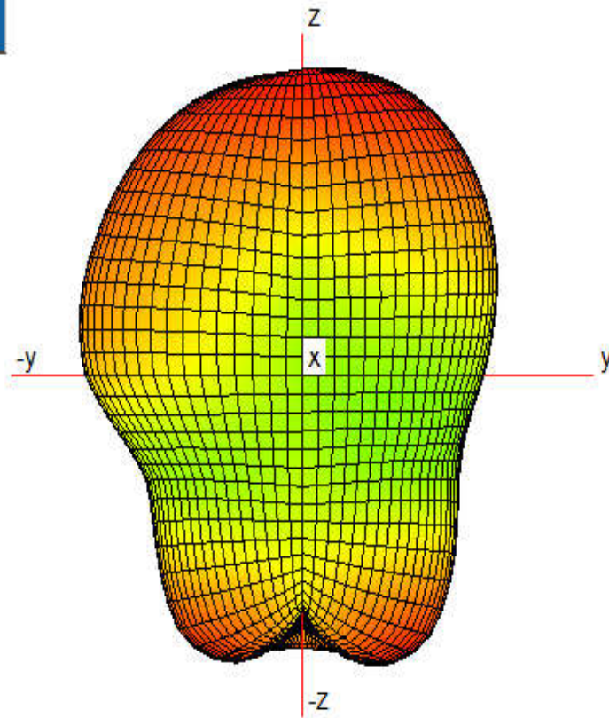
WiFi 2.42G
