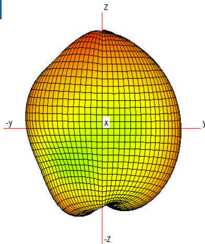
WiFi 2.45G
