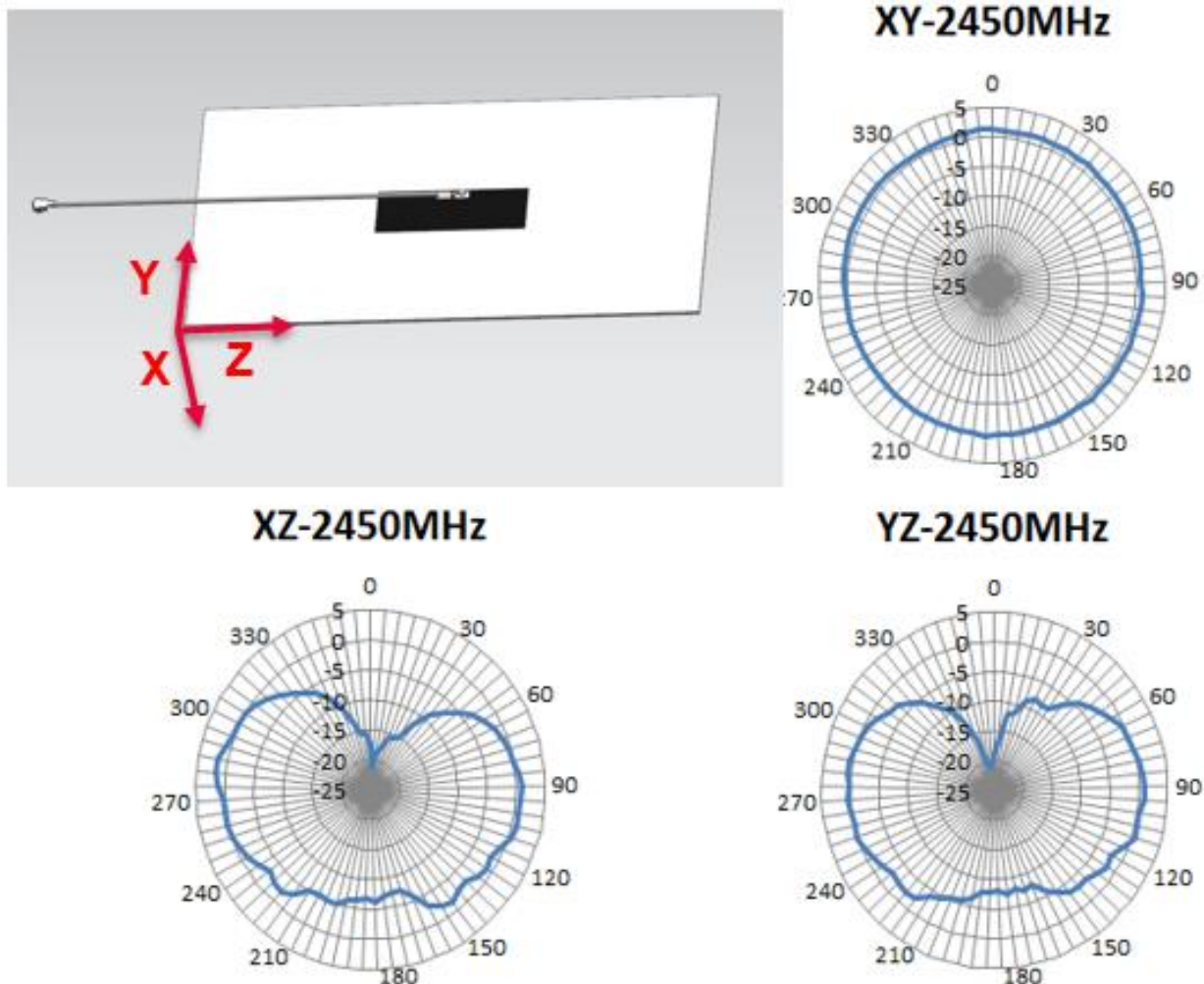
FIGURE 4.5.1 2D RADIATION PATTERN OF ANTENNA AT 2.45GHZ IN FREE SPACE
