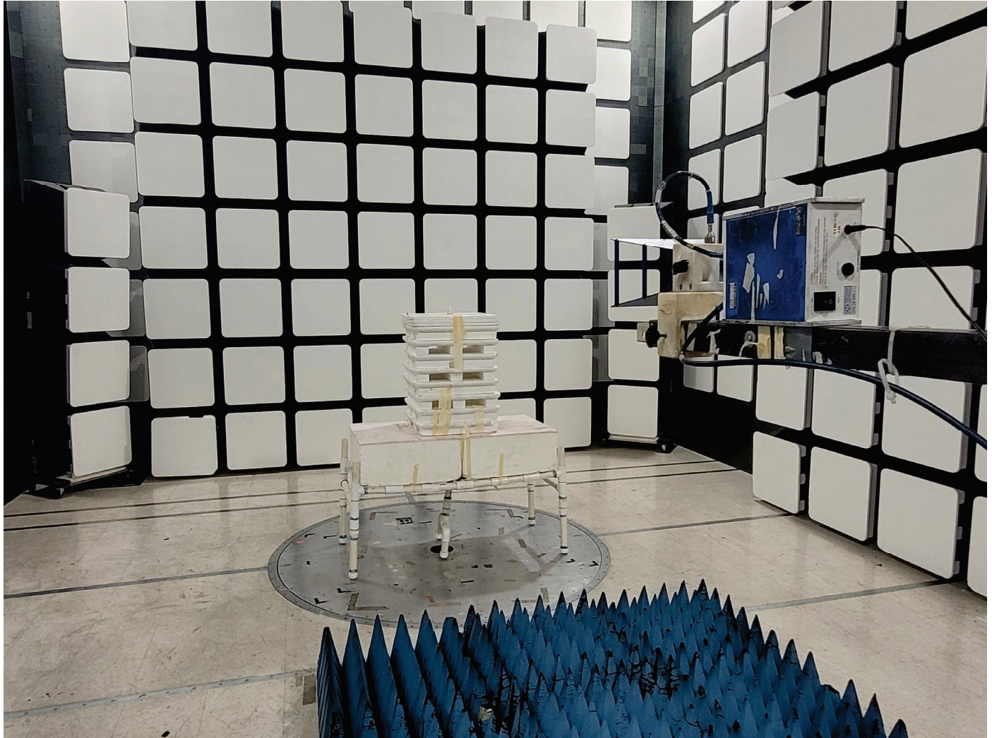
REAR VIEW
