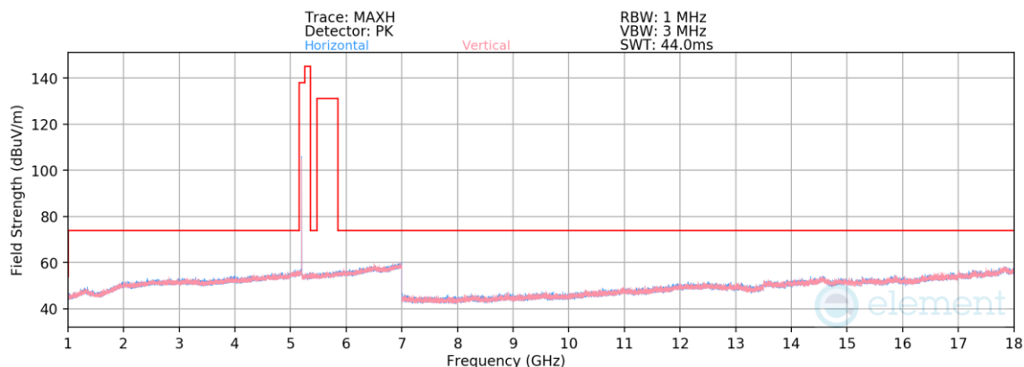
Plot 7-79. Radiated Spurious Emissions 1-18GHz (NB UNII LE2M – 5201MHz)
