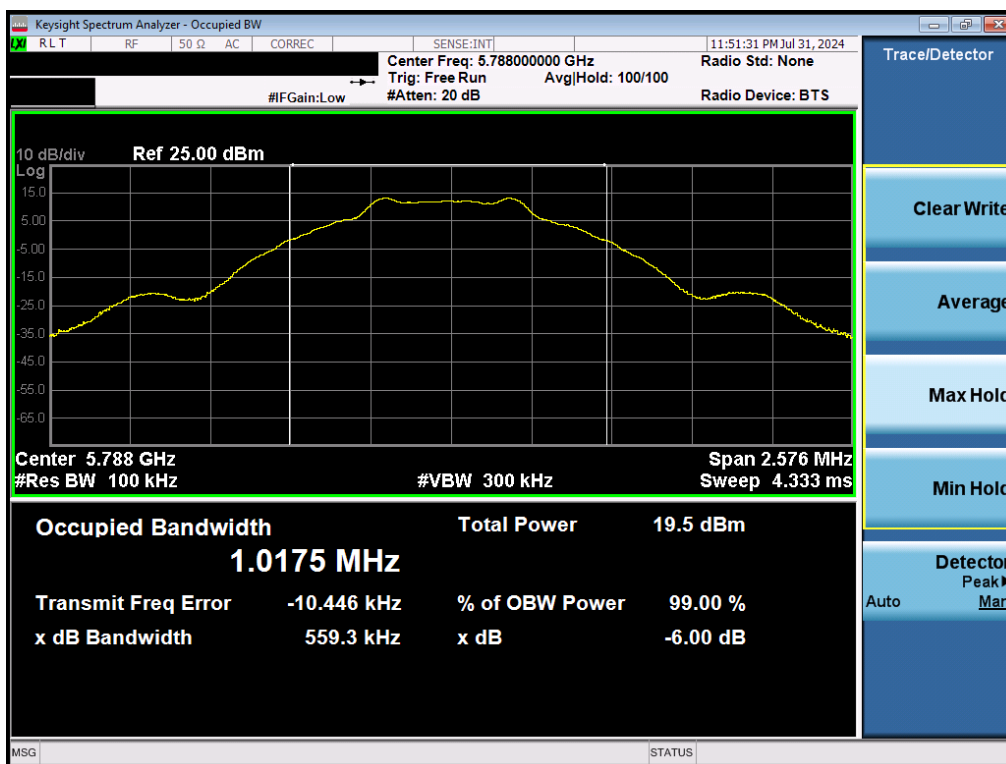
Plot 7-20. 6dB BW & 99% OBW (NB UNII BDR – 5788MHz)
