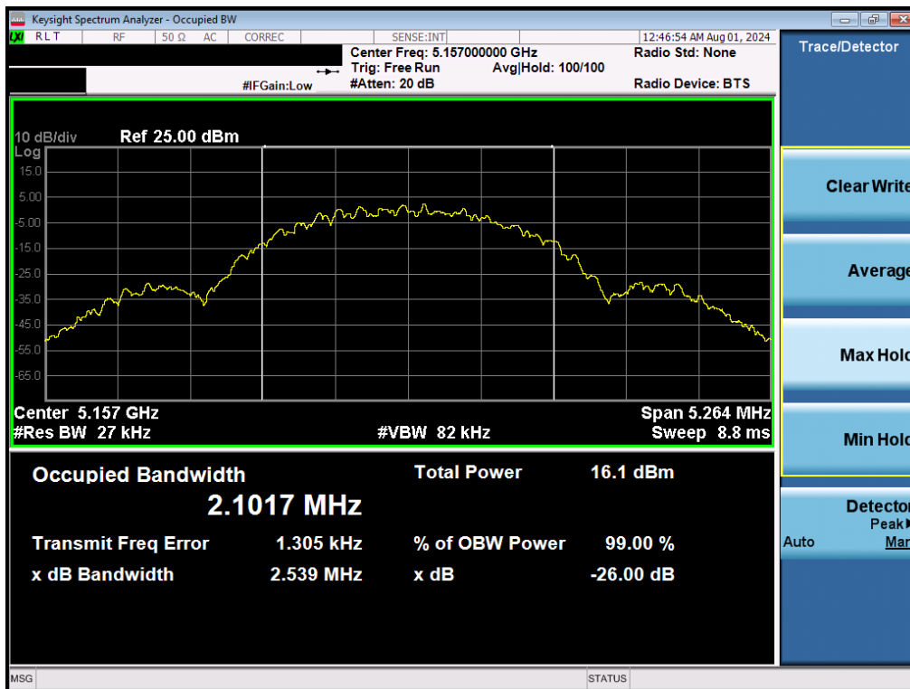
Plot 7-4. 26dB BW & 99% OBW (NB UNII LE2M – 5157MHz)
