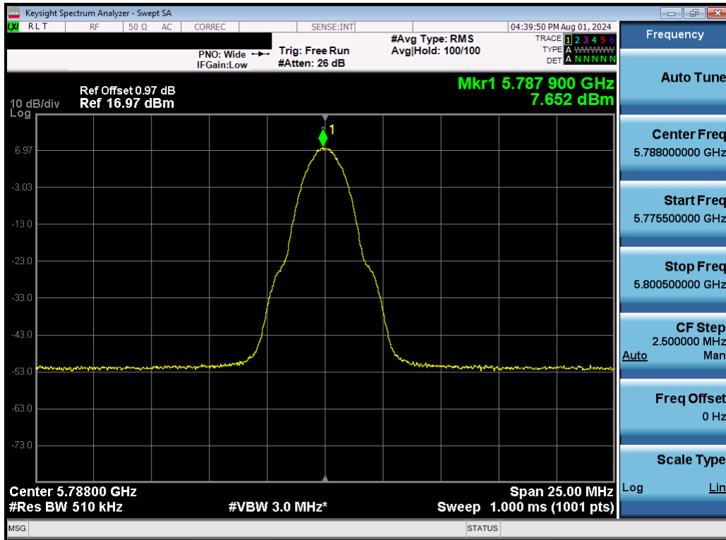
Plot 7-59. PSD (NB UNII LE2M – 5788MHz)
