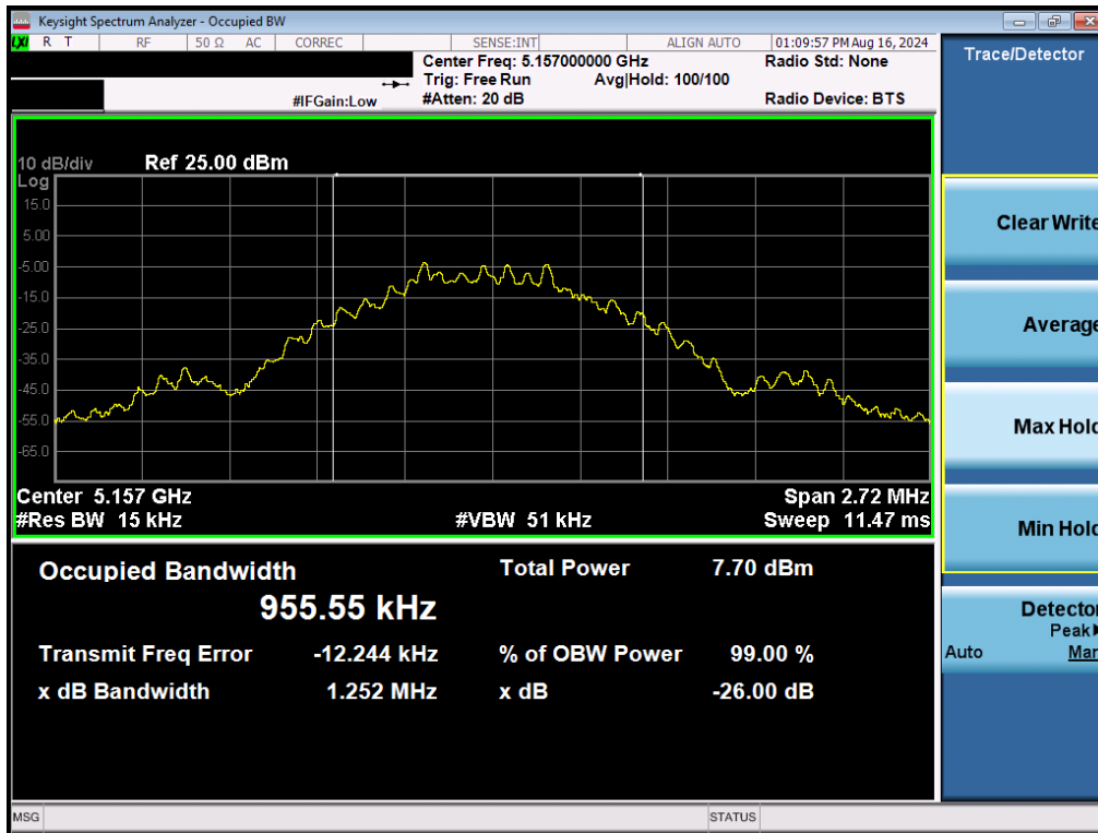
Plot 7-1. 26dB BW & 99% OBW (NB UNII BDR – 5157MHz)
