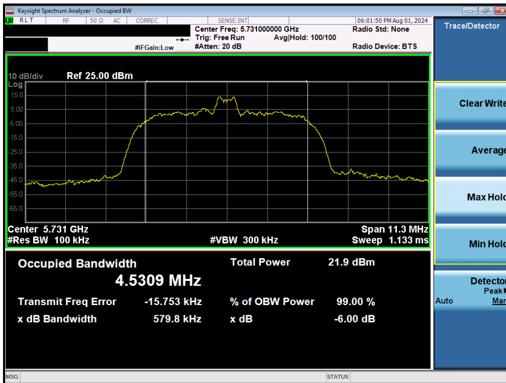
Plot 7-28. 6dB BW & 99% OBW (NB UNII HDR8 – 5731MHz)
