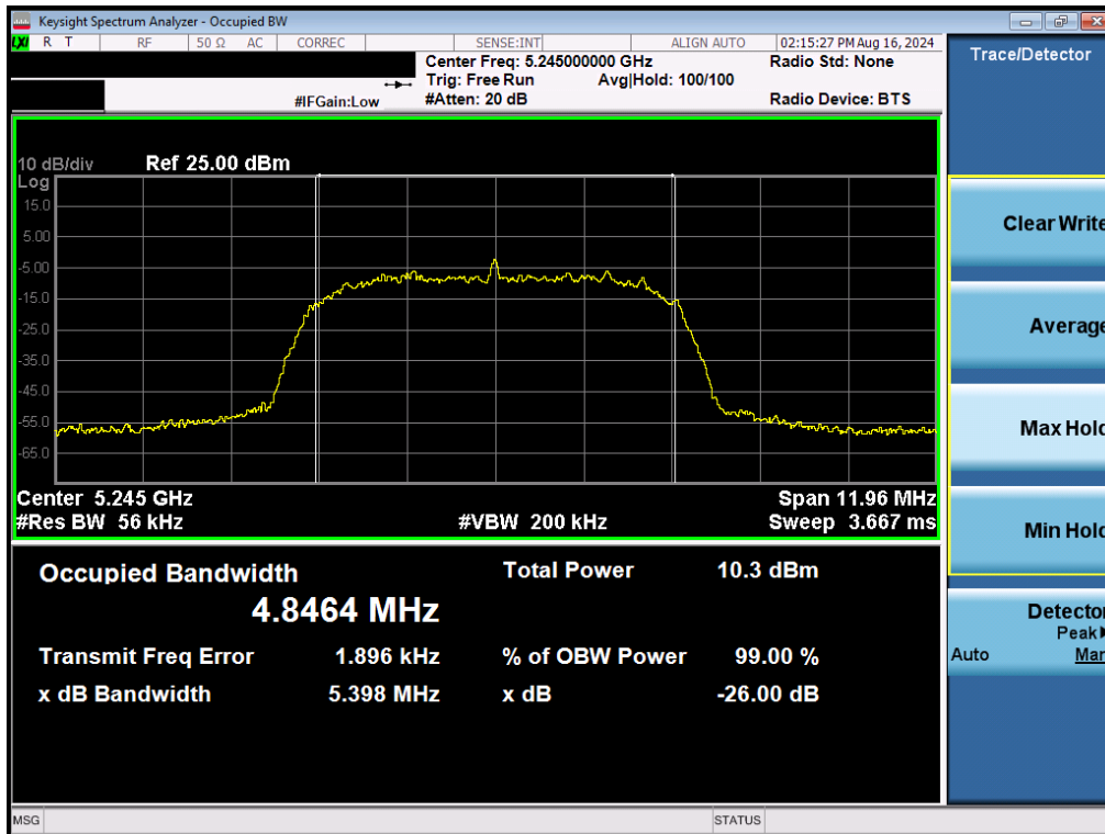
Plot 7-18. 26dB BW & 99% OBW (NB UNII HDRp8 – 5245MHz)
