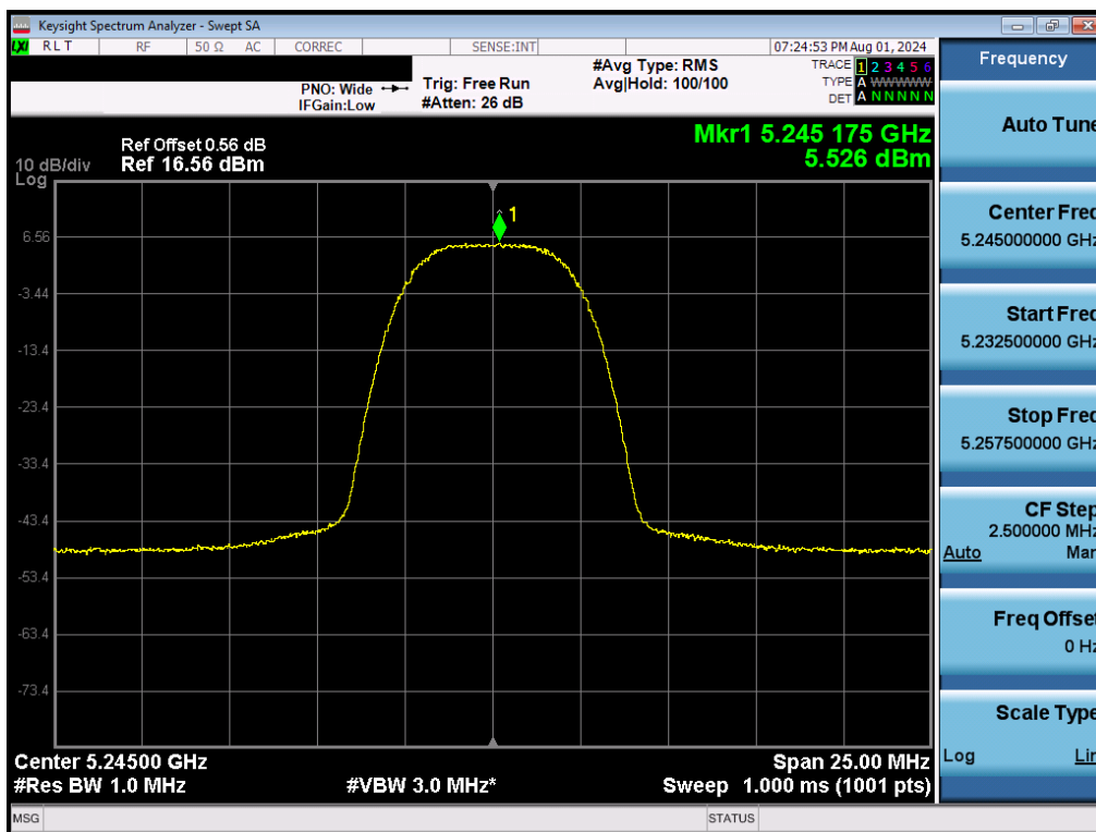
Plot 7-54. FCC PSD (NB UNII HDRp8 – 5245MHz)
