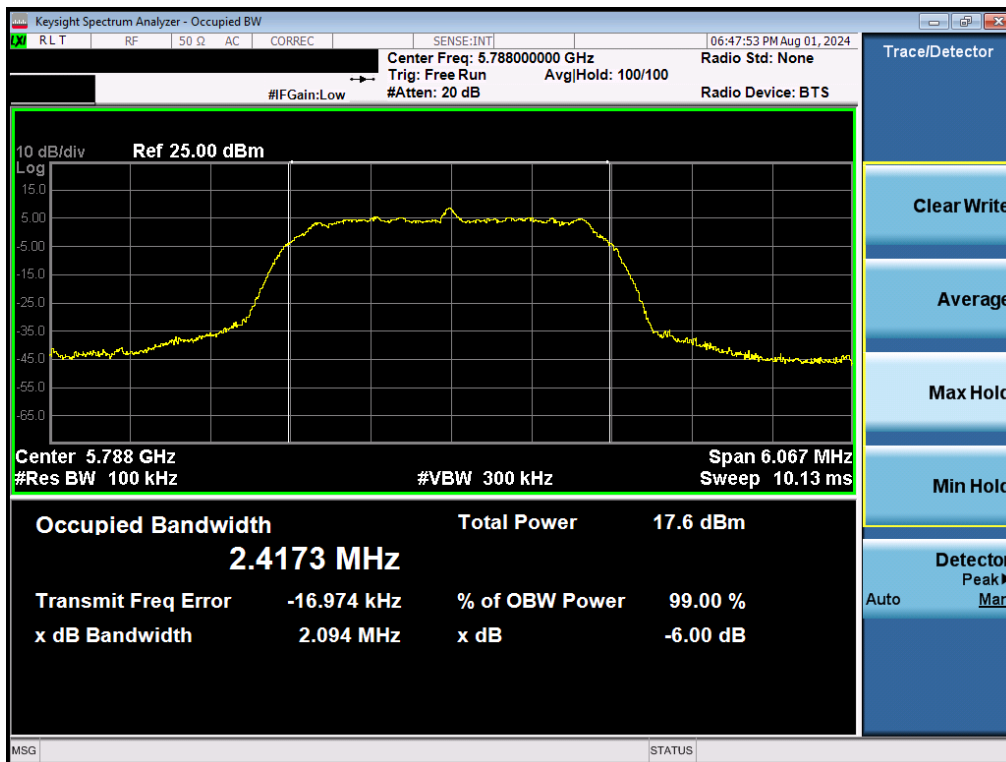
Plot 7-32. 6dB BW & 99% OBW (NB UNII HDRp4 – 5788MHz)
