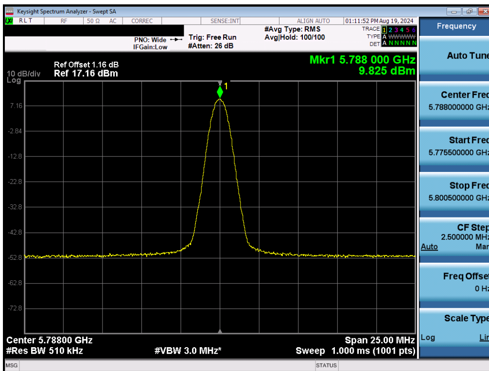
Plot 7-56. PSD (NB UNII BDR – 5788MHz)
