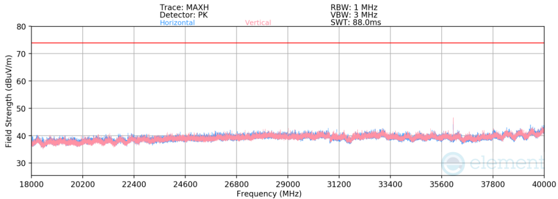
Plot 7-74. Radiated Spurious Emissions 18-40GHz (NB UNII BDR – 5157MHz)
