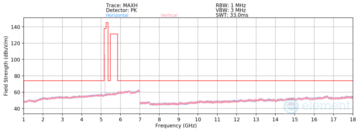
Plot 7-75. Radiated Spurious Emissions 1-18GHz (NB UNII BDR – 5201MHz)
