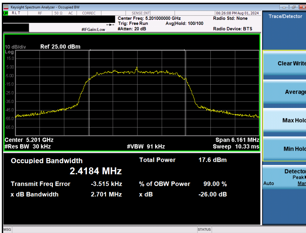
Plot 7-14. 26dB BW & 99% OBW (NB UNII HDRp4 – 5201MHz)
