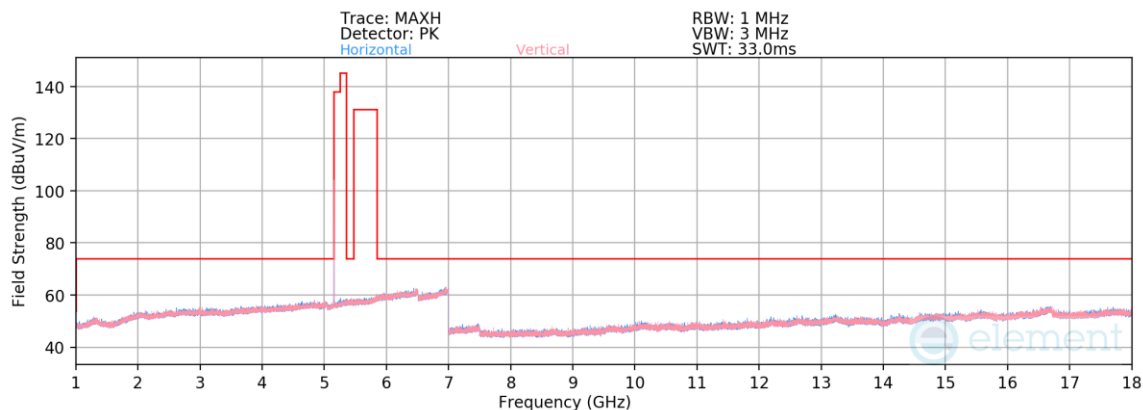
Plot 7-81. Radiated Spurious Emissions 1-18GHz (NB UNII HDR4 – 5157MHz)
