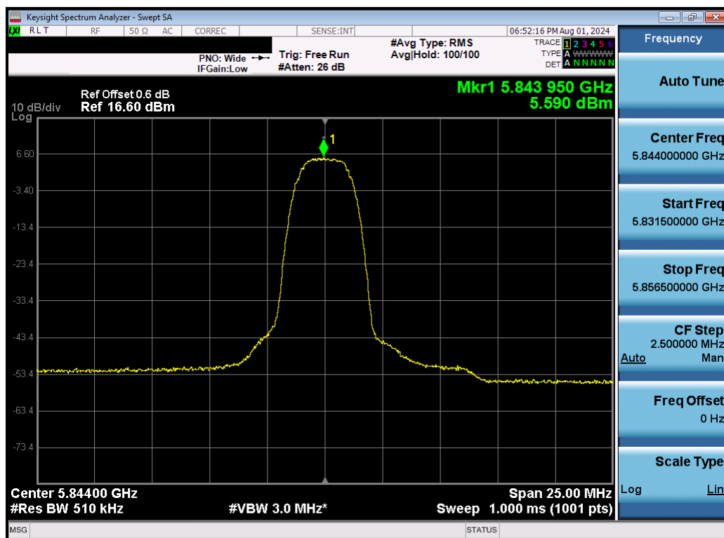
Plot 7-69. PSD (NB UNII HDRp4 – 5844MHz)
