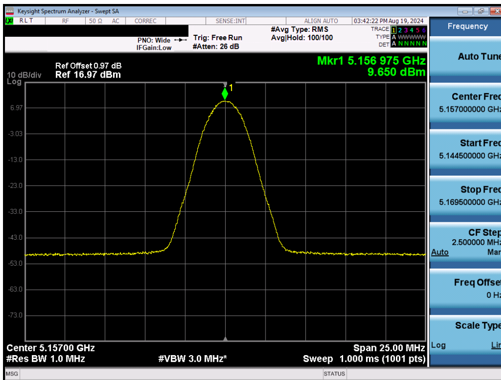
Plot 7-40. FCC PSD (NB UNII LE2M – 5157MHz)
