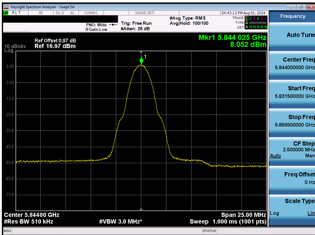
Plot 7-60. PSD (NB UNII LE2M – 5844MHz)
