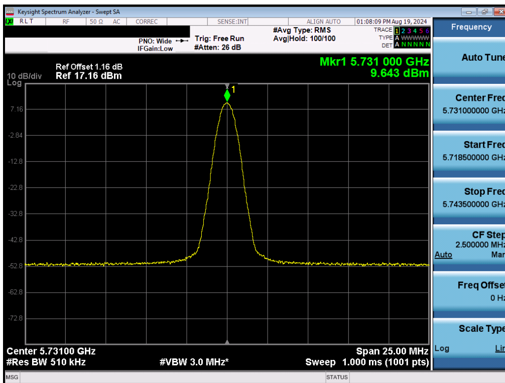
Plot 7-55. PSD (NB UNII BDR – 5731MHz)
