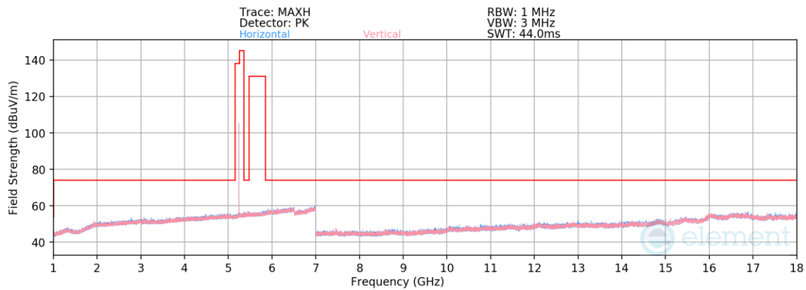
Plot 7-76. Radiated Spurious Emissions 1-18GHz (NB UNII BDR – 5245MHz)
