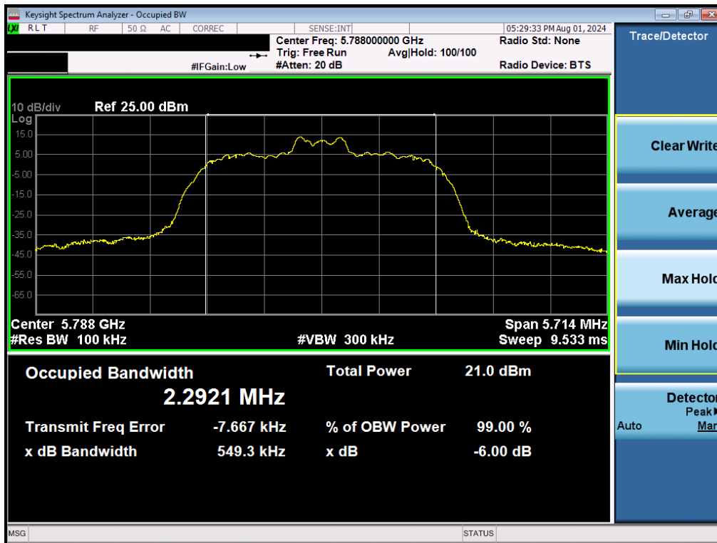
Plot 7-26. 6dB BW & 99% OBW (NB UNII HDR4 – 5788MHz)
