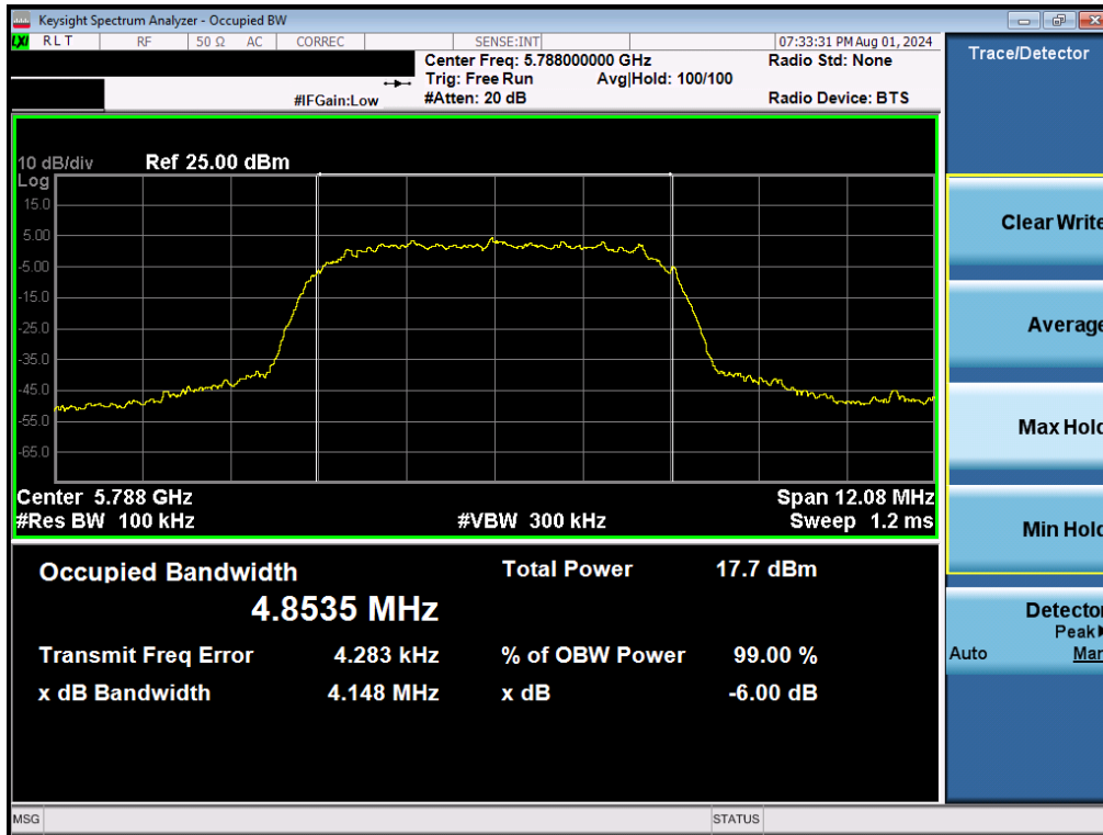
Plot 7-35. 6dB BW & 99% OBW (NB UNII HDRp8 – 5788MHz)
