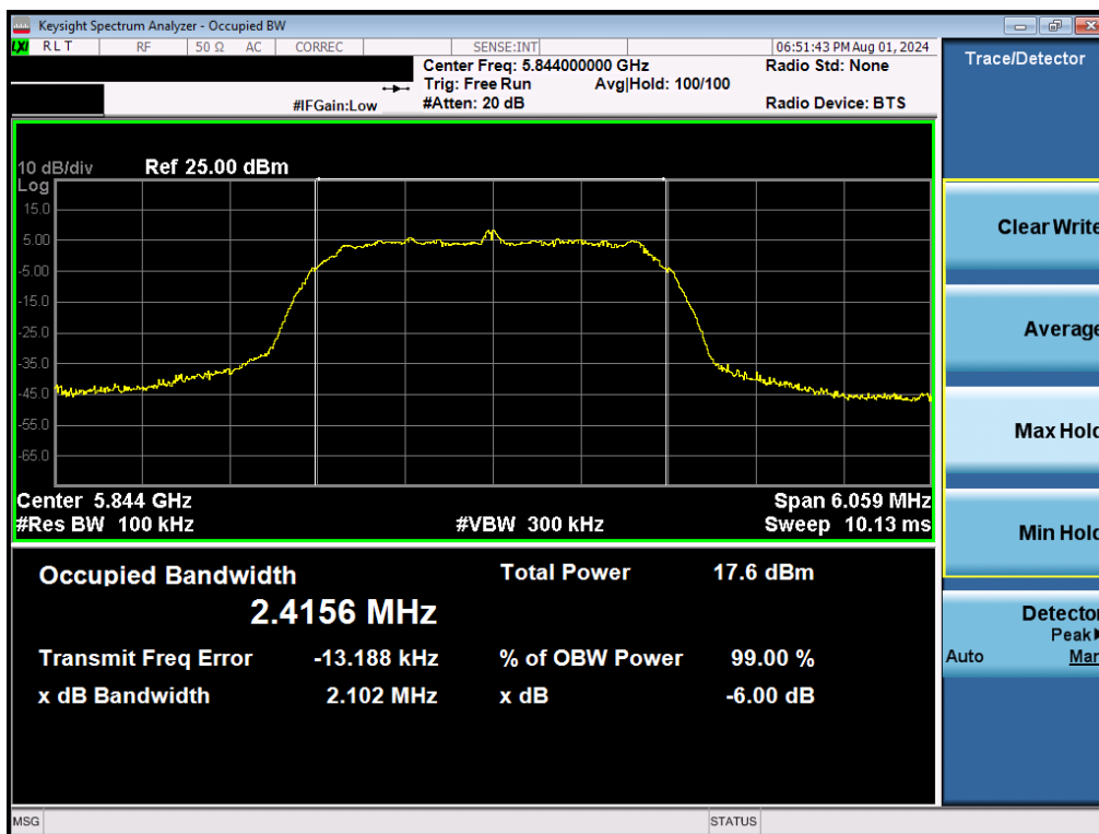
Plot 7-33. 6dB BW & 99% OBW (NB UNII HDRp4 – 5844MHz)
