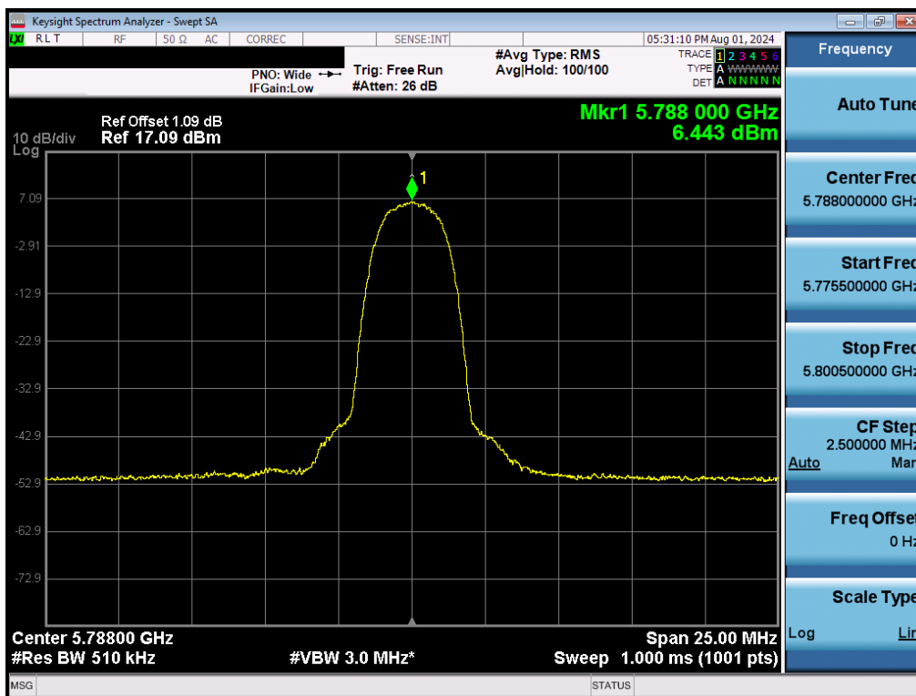
Plot 7-62. PSD (NB UNII HDR4 – 5788MHz)
