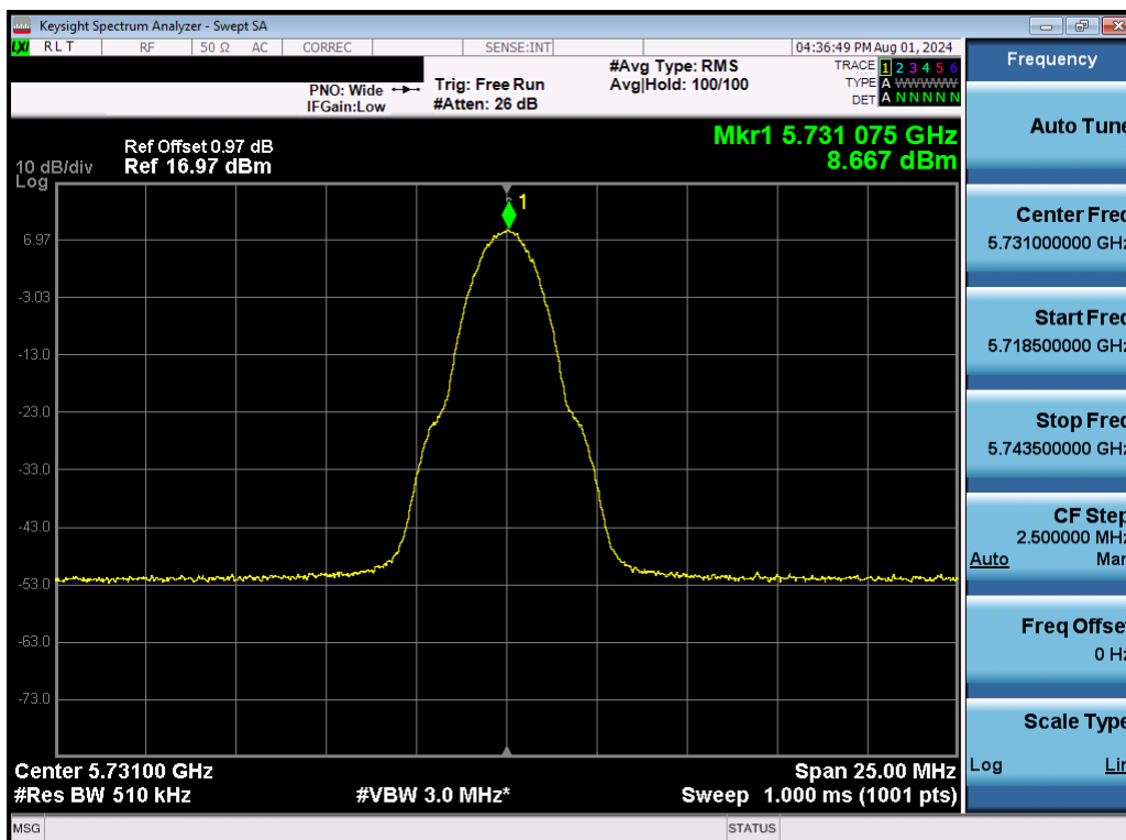
Plot 7-58. PSD (NB UNII LE2M – 5731MHz)
