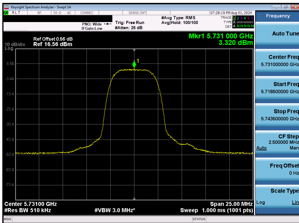
Plot 7-70. PSD (NB UNII HDRp8 – 5731MHz)
