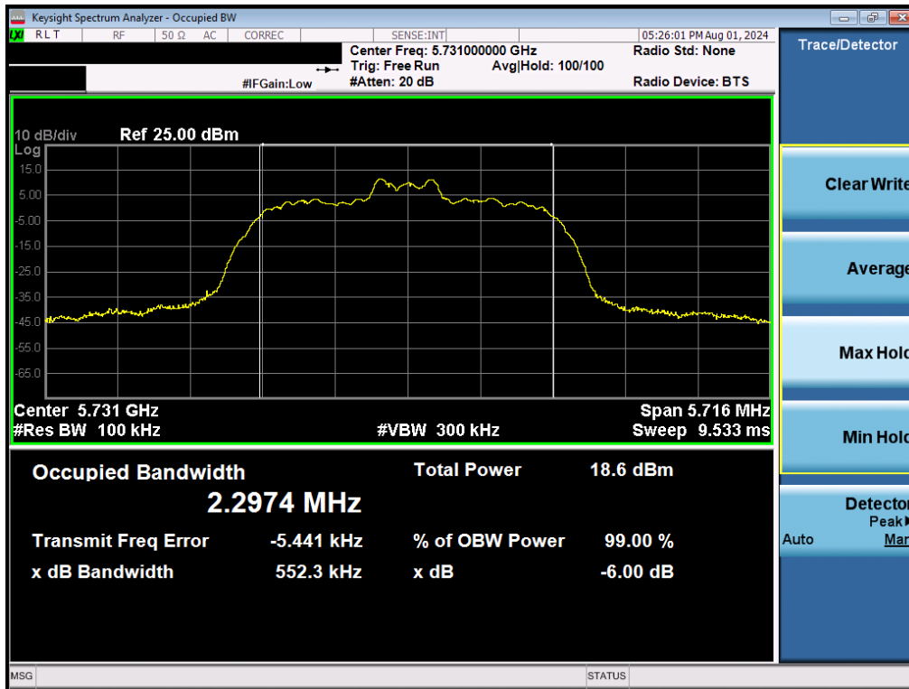
Plot 7-25. 6dB BW & 99% OBW (NB UNII HDR4 – 5731MHz)
