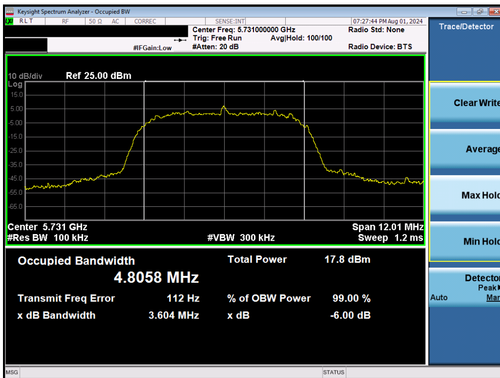
Plot 7-34. 6dB BW & 99% OBW (NB UNII HDRp8 – 5731MHz)
