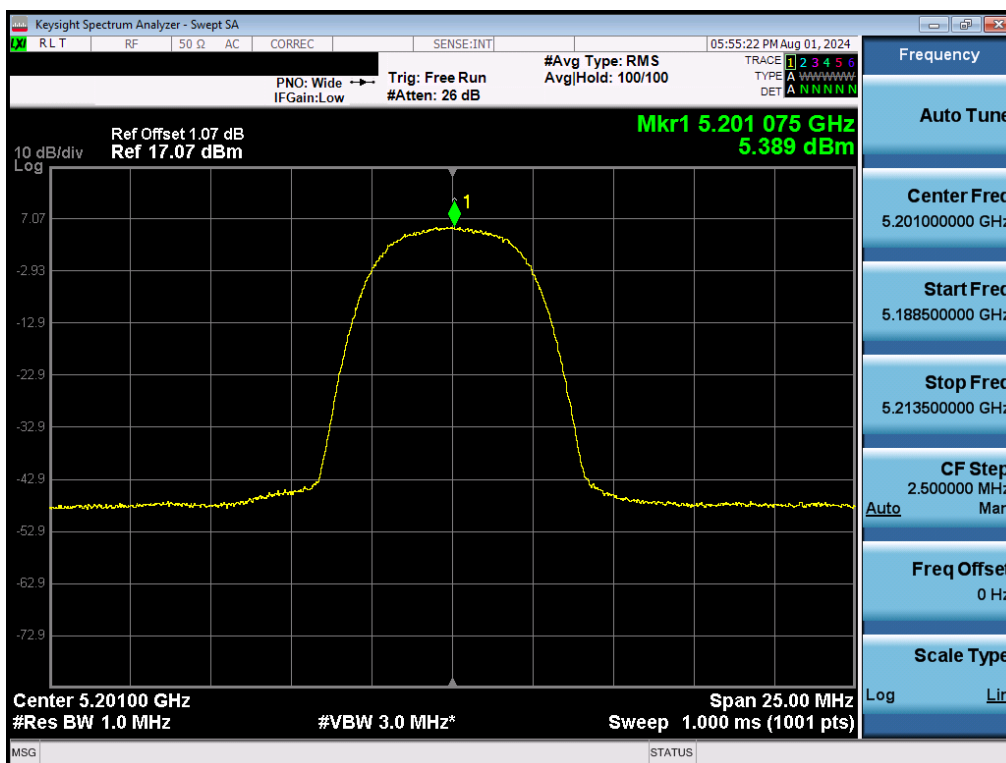
Plot 7-47. FCC PSD (NB UNII HDR8 – 5201MHz)
