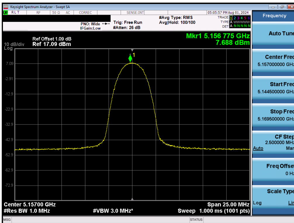
Plot 7-43. FCC PSD (NB UNII HDR4 – 5157MHz)
