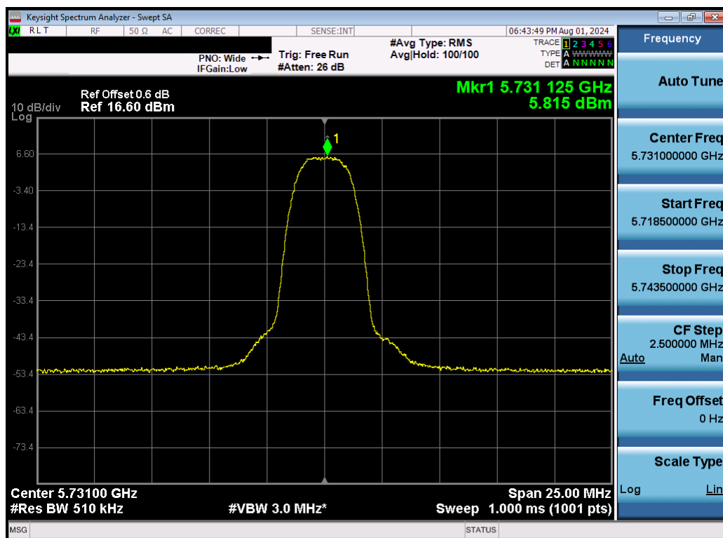
Plot 7-67. PSD (NB UNII HDRp4 – 5731MHz)
