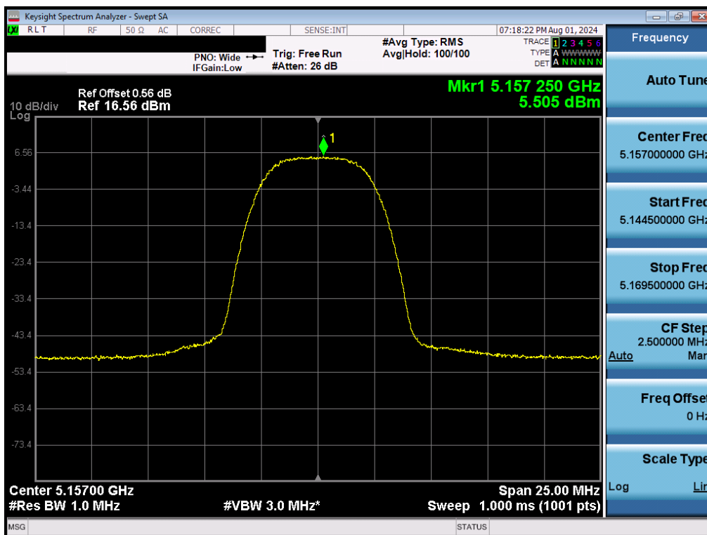
Plot 7-52. FCC PSD (NB UNII HDRp8 – 5157MHz)
