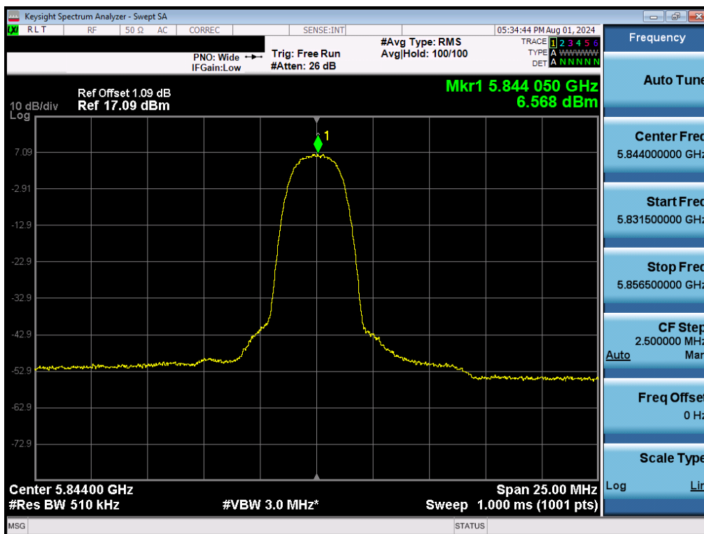
Plot 7-63. PSD (NB UNII HDR4 – 5844MHz)
