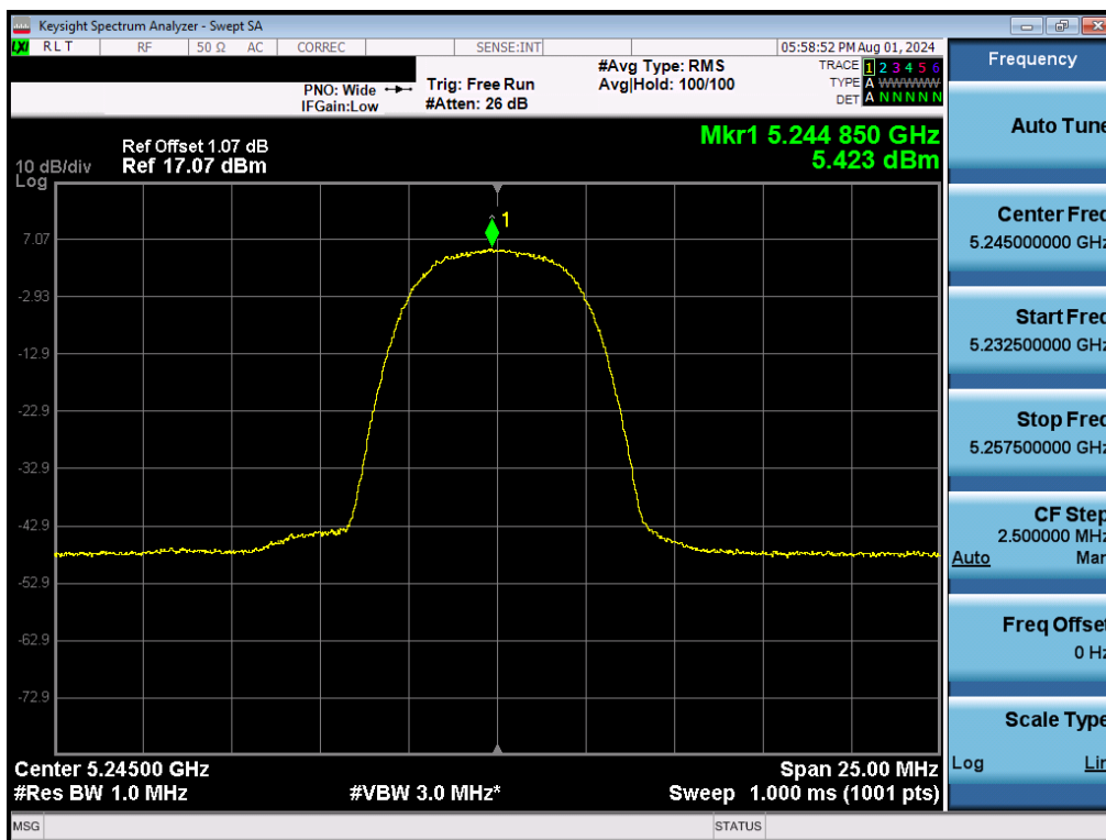
Plot 7-48. FCC PSD (NB UNII HDR8 – 5245MHz)
