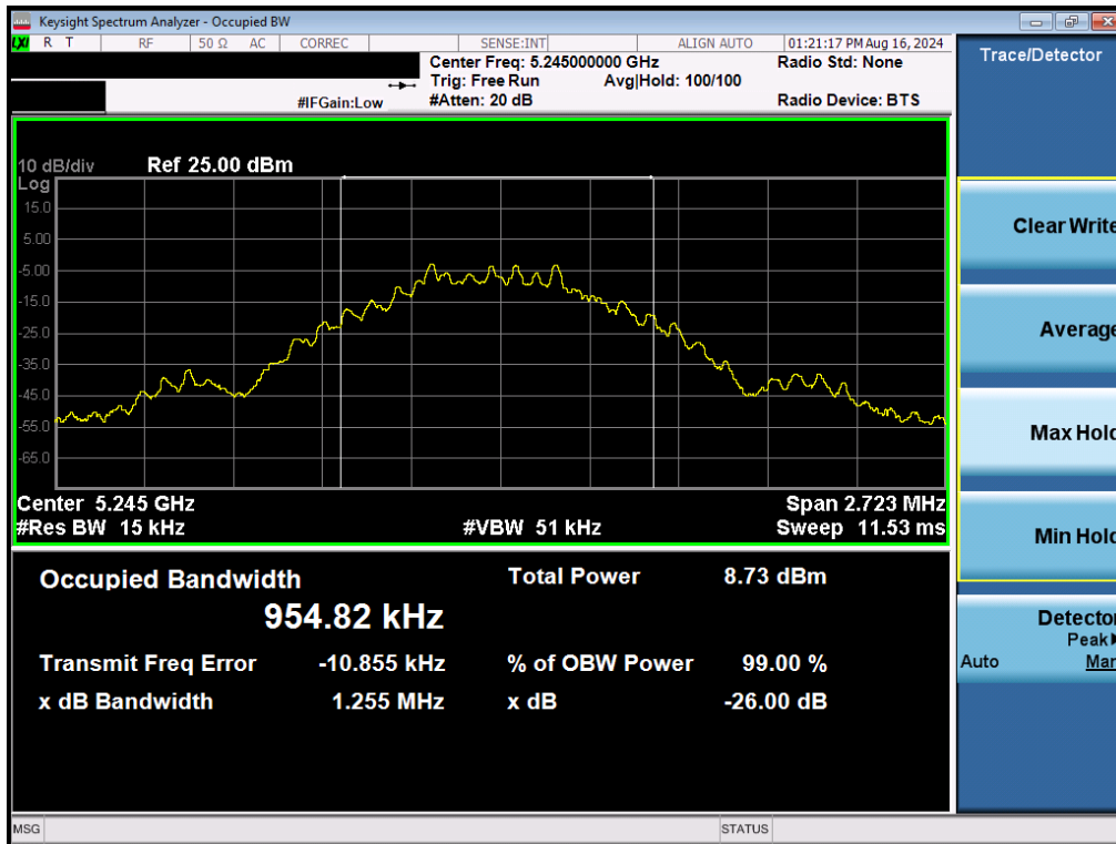
Plot 7-3. 26dB BW & 99% OBW (NB UNII BDR – 5245MHz)
