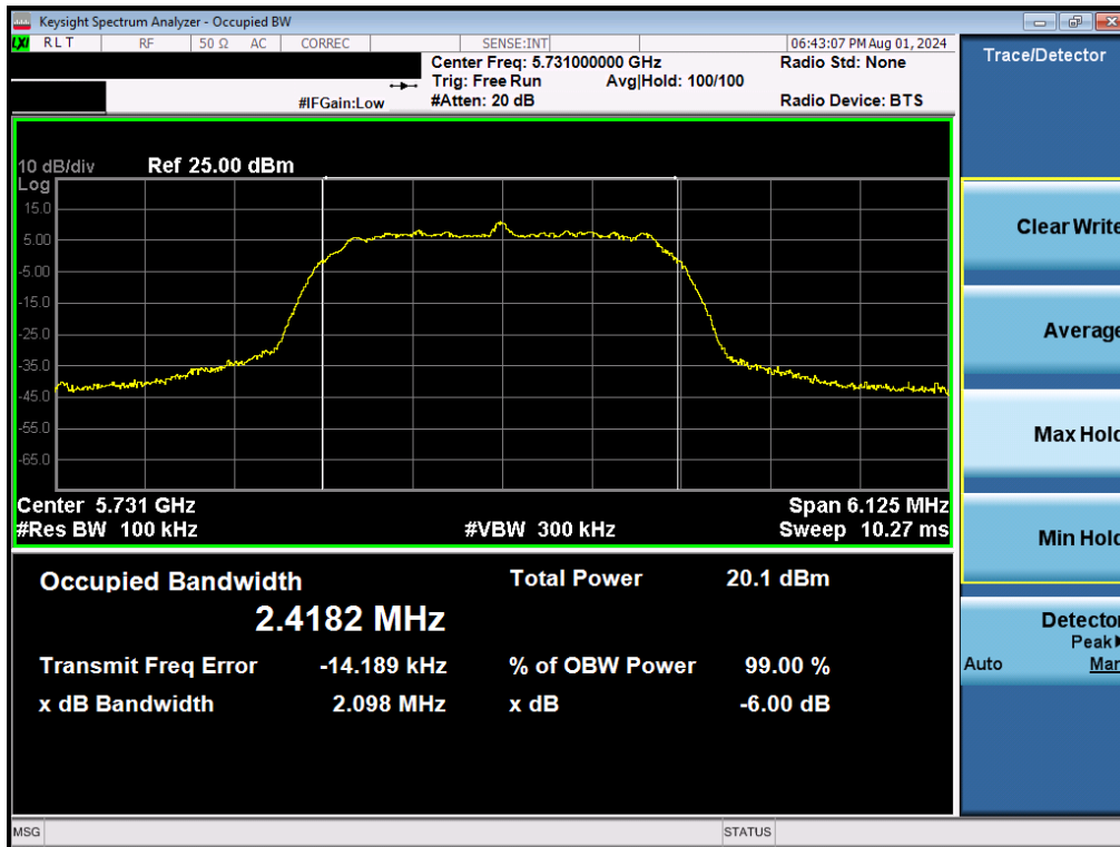
Plot 7-31. 6dB BW & 99% OBW (NB UNII HDRp4 – 5731MHz)
