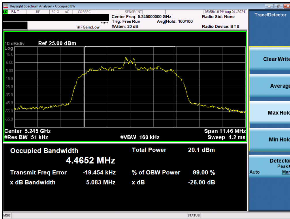
Plot 7-12. 26dB BW & 99% OBW (NB UNII HDR8 – 5245MHz)
