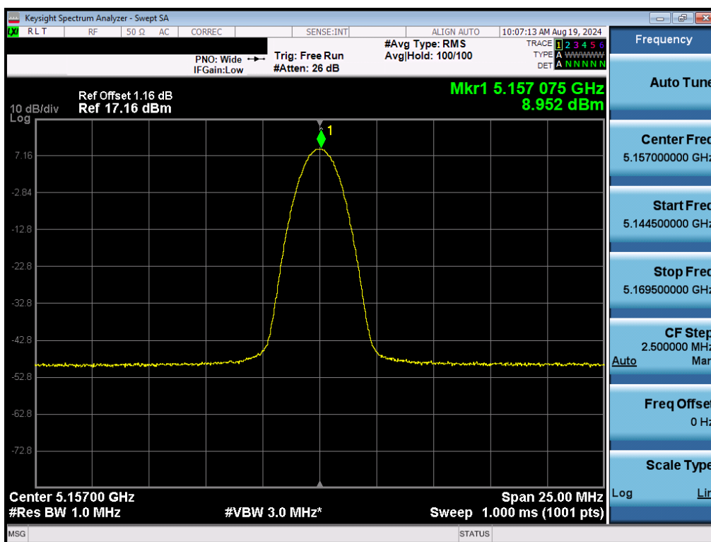
Plot 7-37. FCC PSD (NB UNII BDR – 5157MHz)
