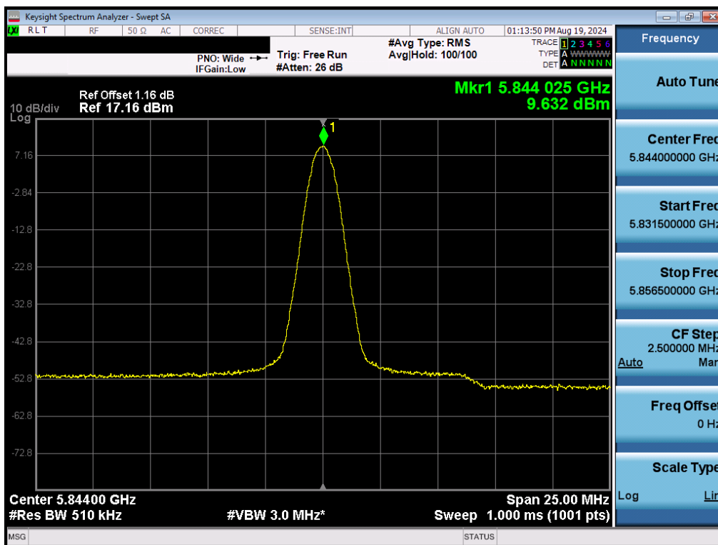
Plot 7-57. PSD (NB UNII BDR – 5844MHz)
