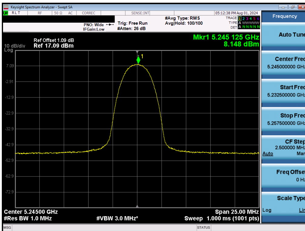
Plot 7-45. FCC PSD (NB UNII HDR4 – 5245MHz)
