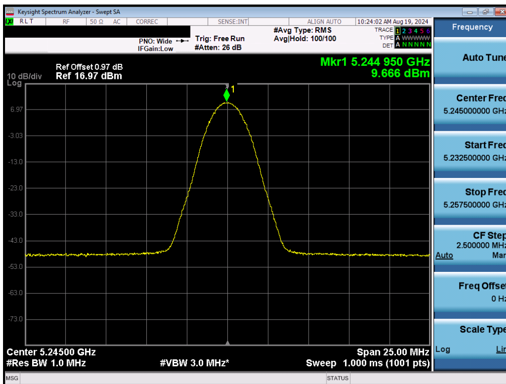
Plot 7-42. FCC PSD (NB UNII LE2M – 5245MHz)
