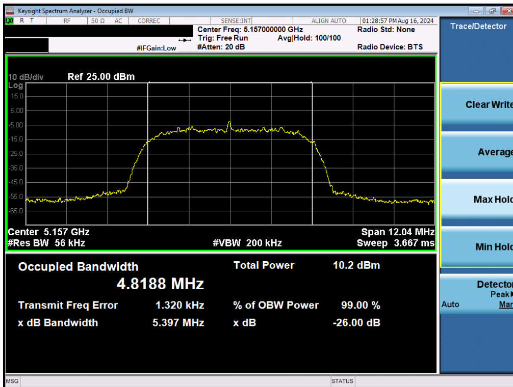
Plot 7-16. 26dB BW & 99% OBW (NB UNII HDRp8 – 5157MHz)
