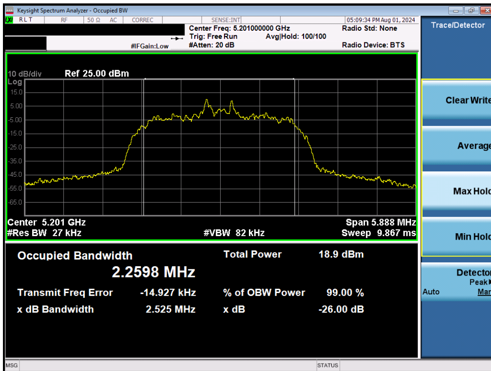
Plot 7-8. 26dB BW & 99% OBW (NB UNII HDR4 – 5201MHz)
