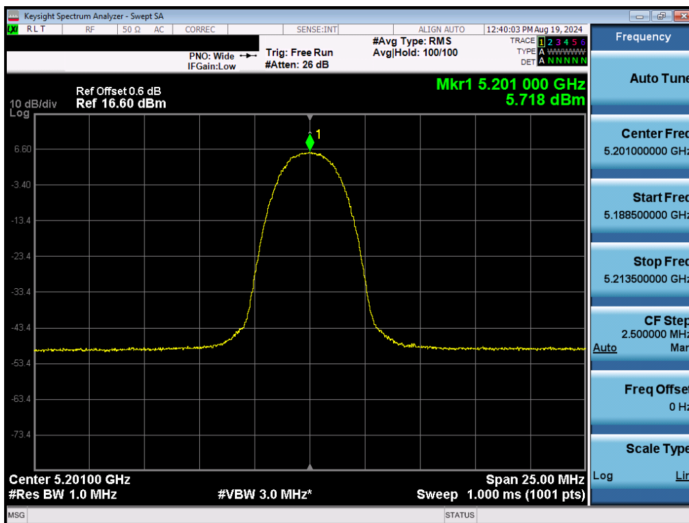
Plot 7-50. FCC PSD (NB UNII HDRp4 – 5201MHz)
