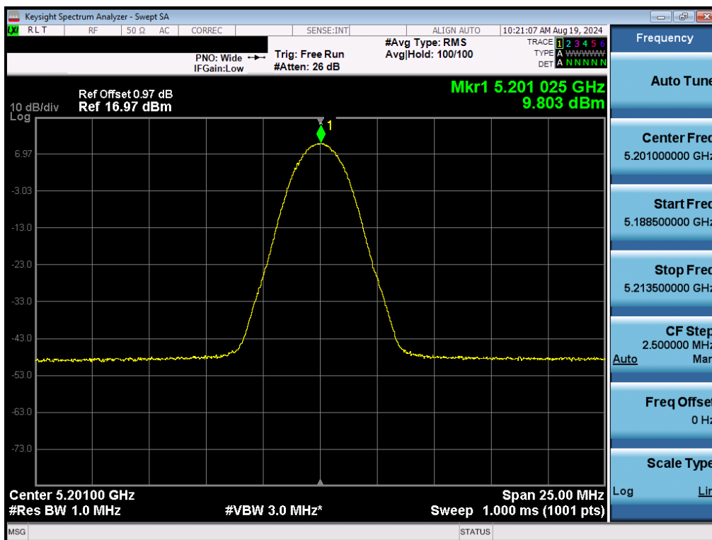
Plot 7-41. FCC PSD (NB UNII LE2M – 5201MHz)
