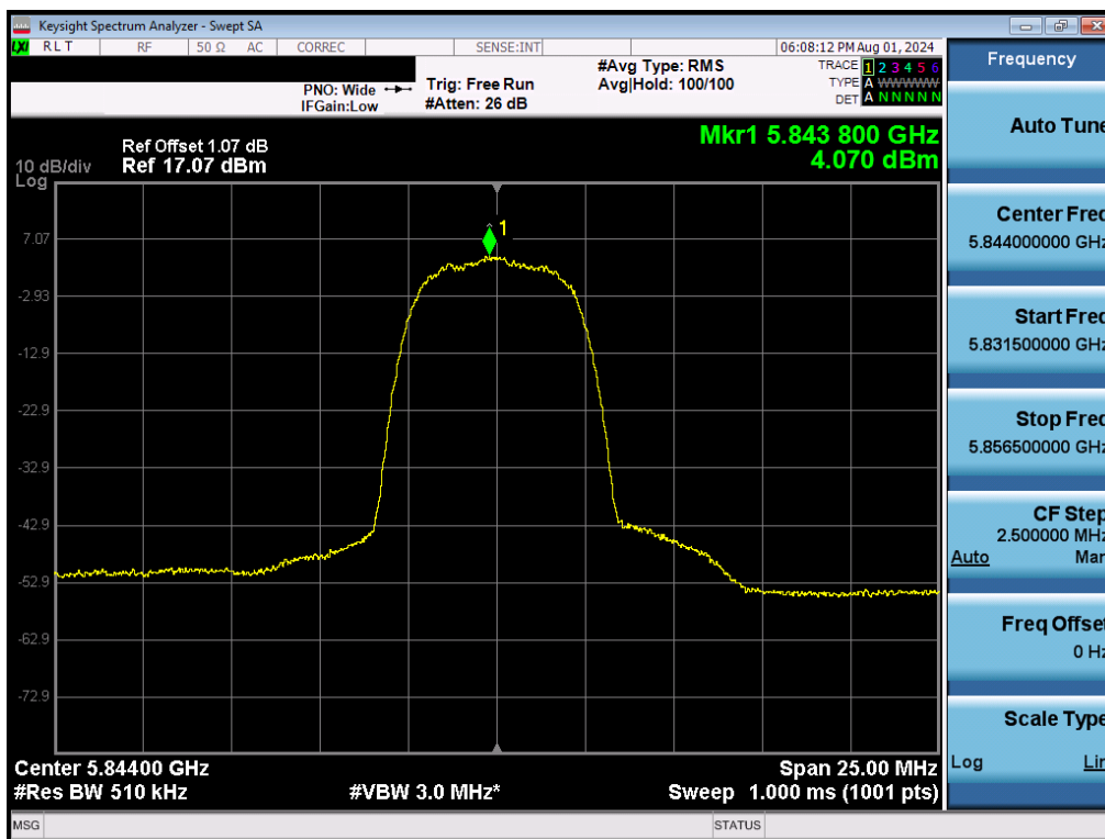
Plot 7-66. PSD (NB UNII HDR8 – 5844MHz)
