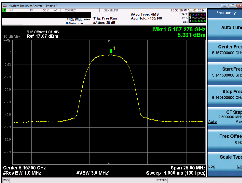
Plot 7-46. FCC PSD (NB UNII HDR8 – 5157MHz)
