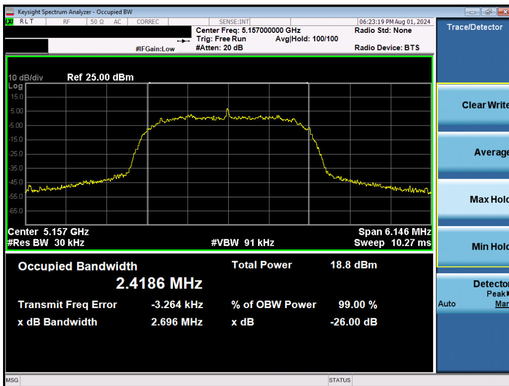
Plot 7-13. 26dB BW & 99% OBW (NB UNII HDRp4 – 5157MHz)
