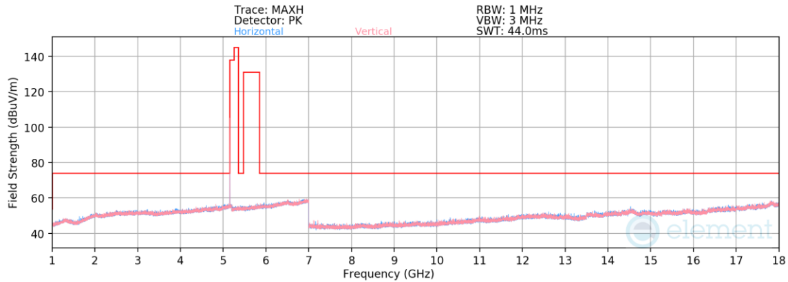
Plot 7-77. Radiated Spurious Emissions 1-18GHz (NB UNII LE2M – 5157MHz)
