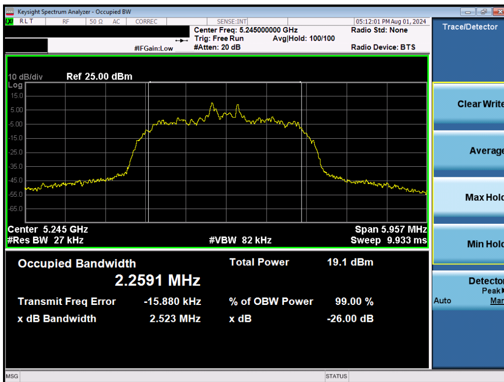
Plot 7-9. 26dB BW & 99% OBW (NB UNII HDR4 – 5245MHz)
