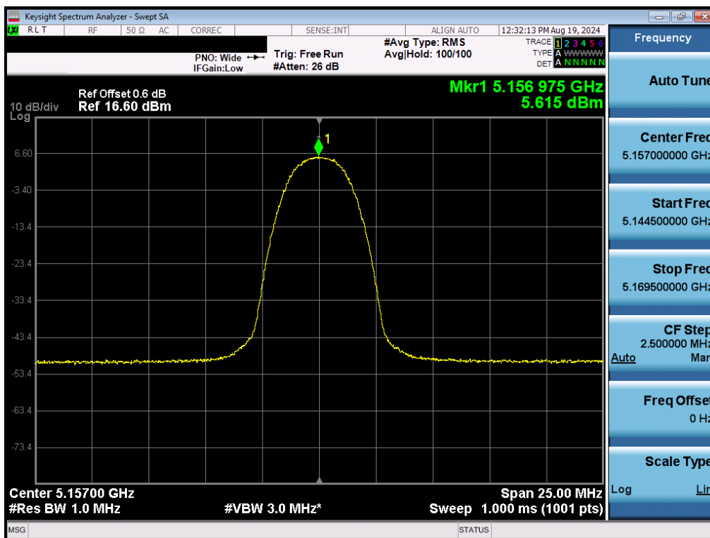
Plot 7-49. FCC PSD (NB UNII HDRp4 – 5157MHz)
