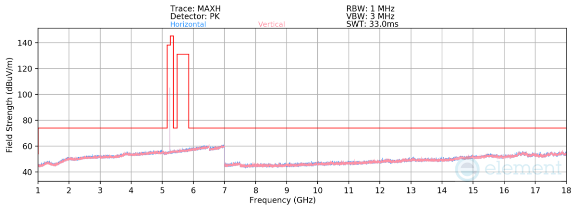
Plot 7-80. Radiated Spurious Emissions 1-18GHz (NB UNII LE2M – 5245MHz)
