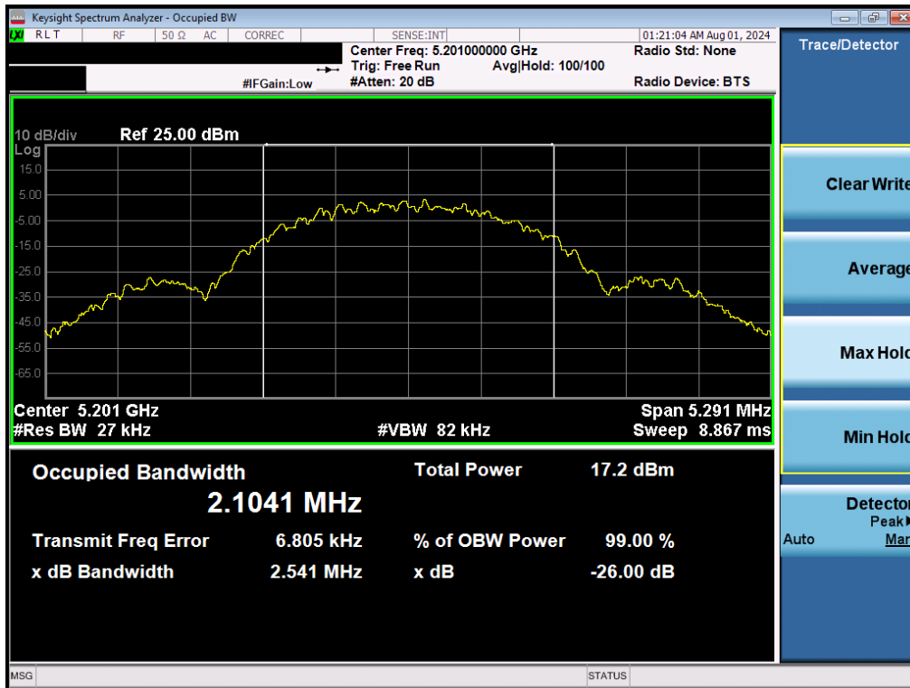
Plot 7-5. 26dB BW & 99% OBW (NB UNII LE2M – 5201MHz)
