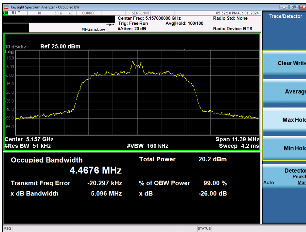
Plot 7-10. 26dB BW & 99% OBW (NB UNII HDR8 – 5157MHz)
