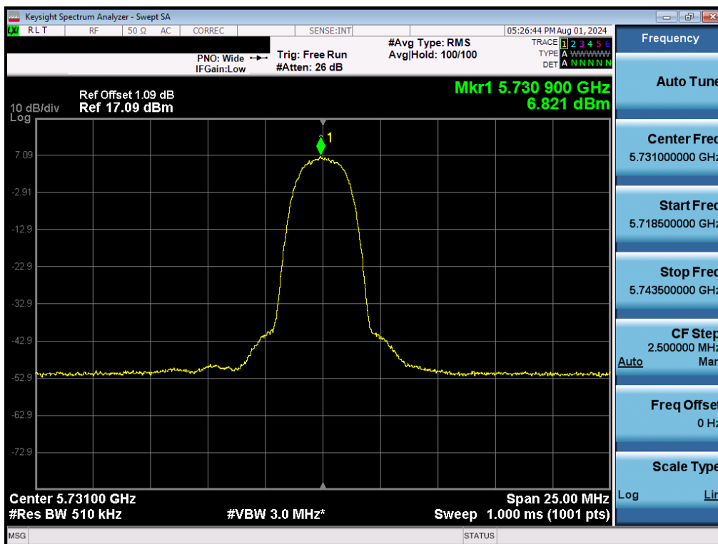
Plot 7-61. PSD (NB UNII HDR4 – 5731MHz)
