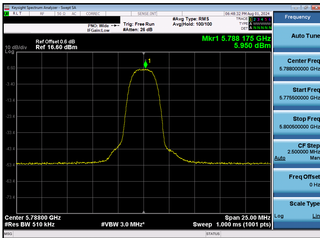
Plot 7-68. PSD (NB UNII HDRp4 – 5788MHz)
