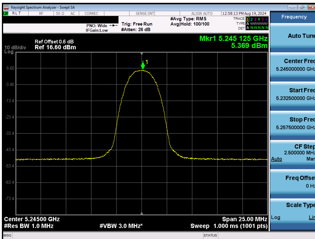
Plot 7-51. FCC PSD (NB UNII HDRp4 – 5245MHz)
