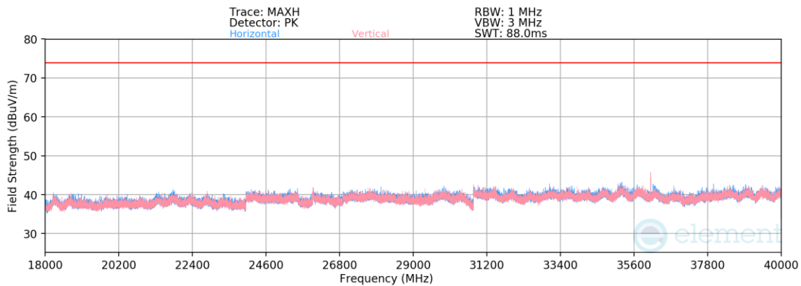
Plot 7-78. Radiated Spurious Emission 18-40GHz (NB UNII LE2M – 5157MHz)
