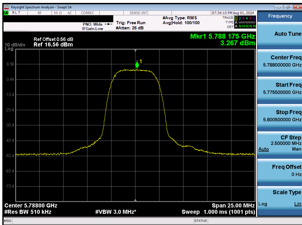
Plot 7-71. PSD (NB UNII HDRp8 – 5788MHz)
