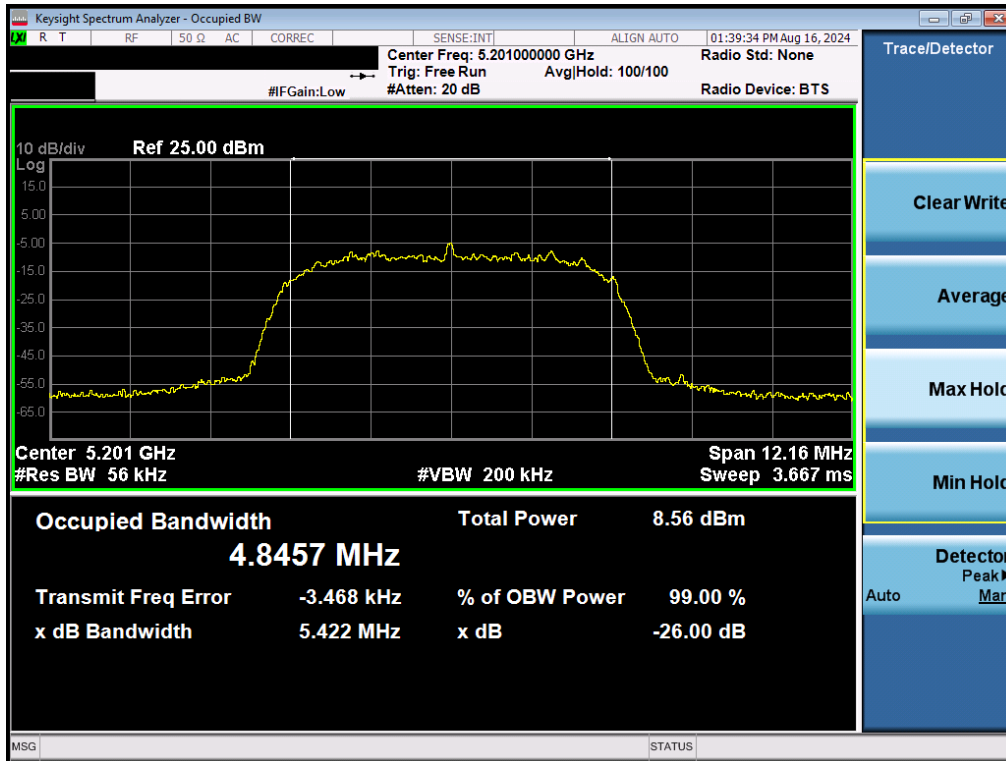
Plot 7-17. 26dB BW & 99% OBW (NB UNII HDRp8 – 5201MHz)
