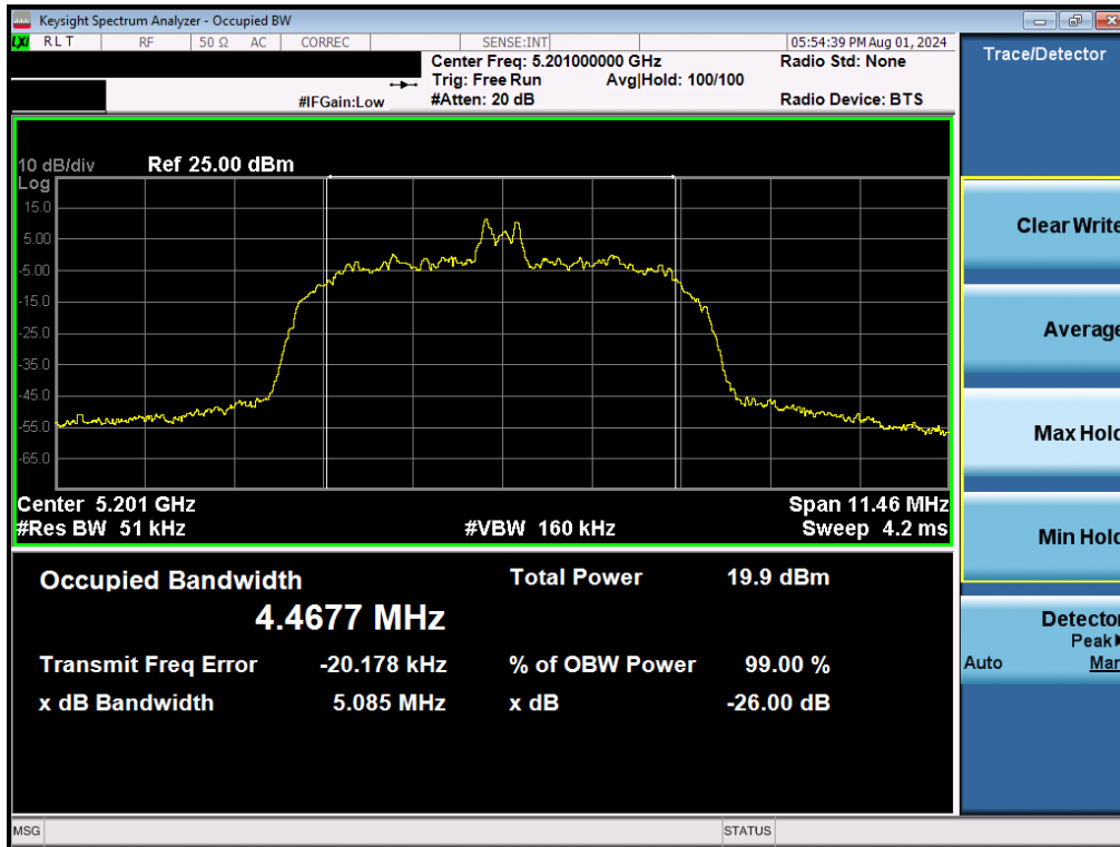
Plot 7-11. 26dB BW & 99% OBW (NB UNII HDR8 – 5201MHz)
