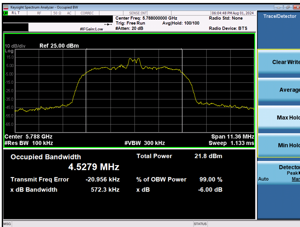
Plot 7-29. 6dB BW & 99% OBW (NB UNII HDR8 – 5788MHz)
