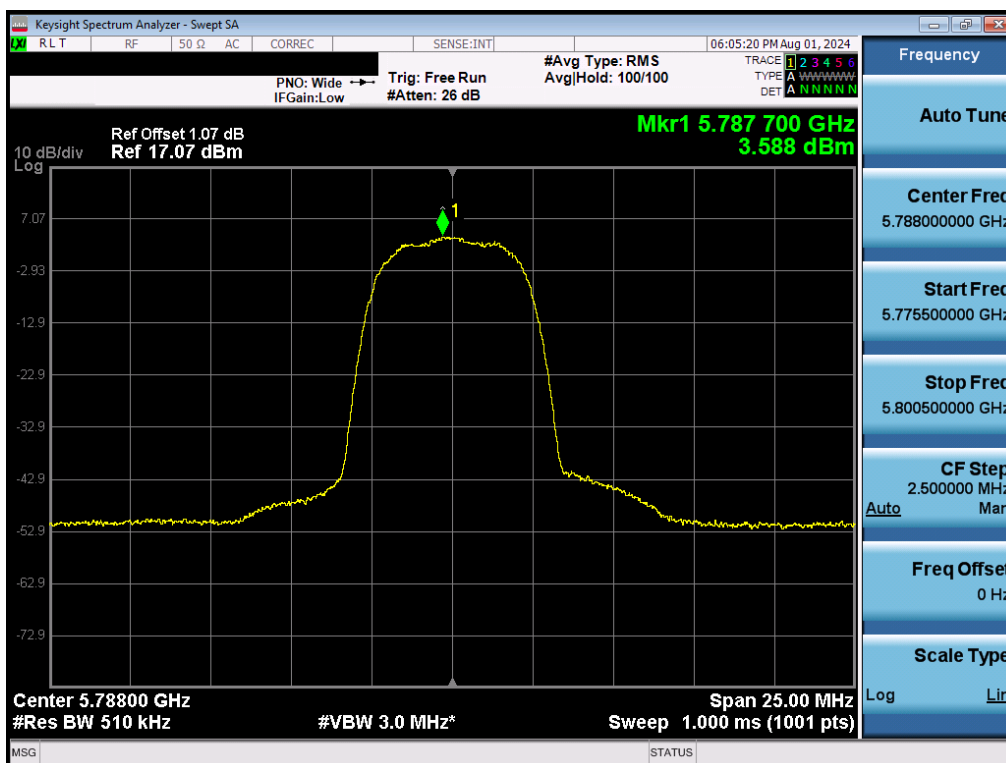
Plot 7-65. PSD (NB UNII HDR8 – 5788MHz)
