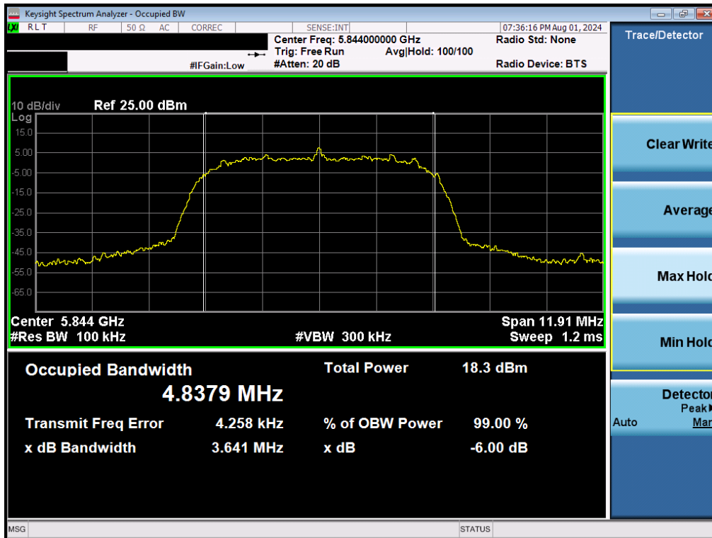
Plot 7-36. 6dB BW & 99% OBW (NB UNII HDRp8 – 5844MHz)
