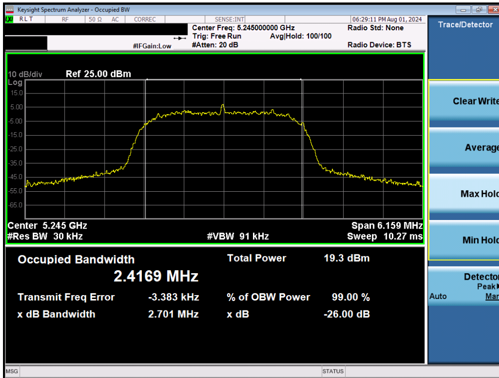
Plot 7-15. 26dB BW & 99% OBW (NB UNII HDRp4 – 5245MHz)
