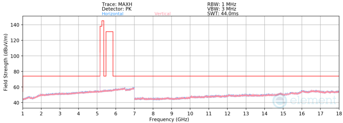
Plot 7-73. Radiated Spurious Emissions 1-18GHz (NB UNII BDR – 5157MHz)
