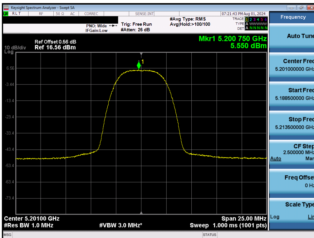
Plot 7-53. FCC PSD (NB UNII HDRp8 – 5201MHz)
