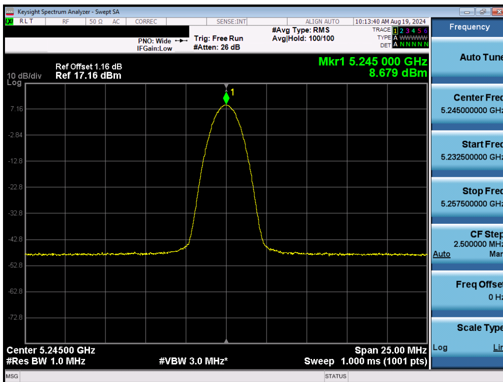
Plot 7-39. FCC PSD (NB UNII BDR – 5245MHz)
