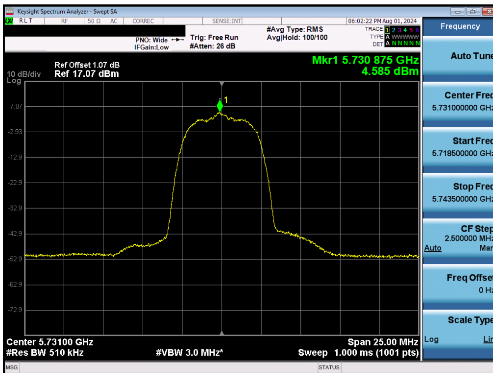
Plot 7-64. PSD (NB UNII HDR8 – 5731MHz)
