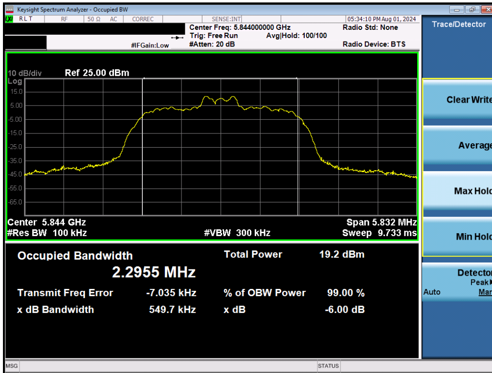
Plot 7-27. 6dB BW & 99% OBW (NB UNII HDR4 – 5844MHz)
