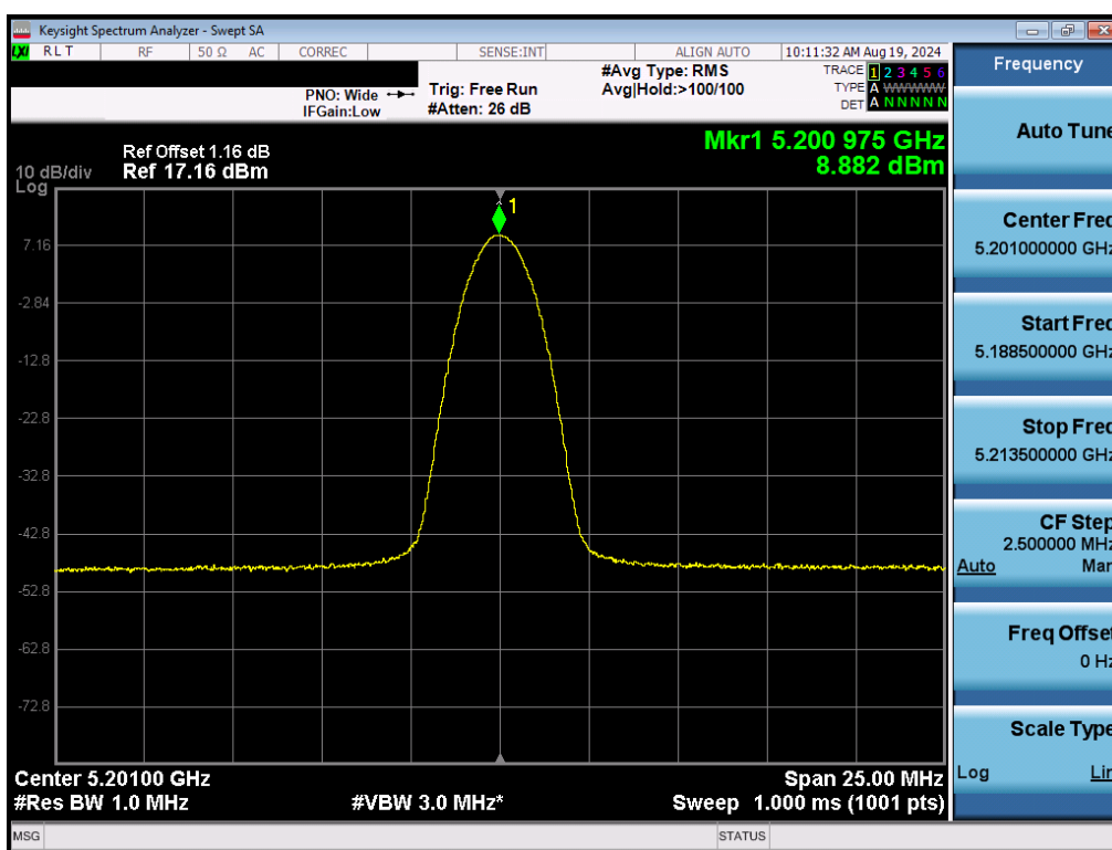
Plot 7-38. FCC PSD (NB UNII BDR – 5201MHz)
