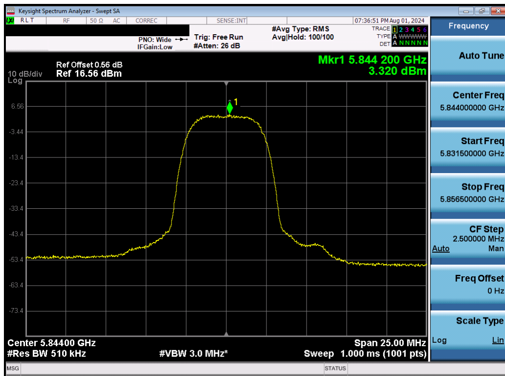
Plot 7-72. PSD (NB UNII HDRp8 – 5844MHz)
