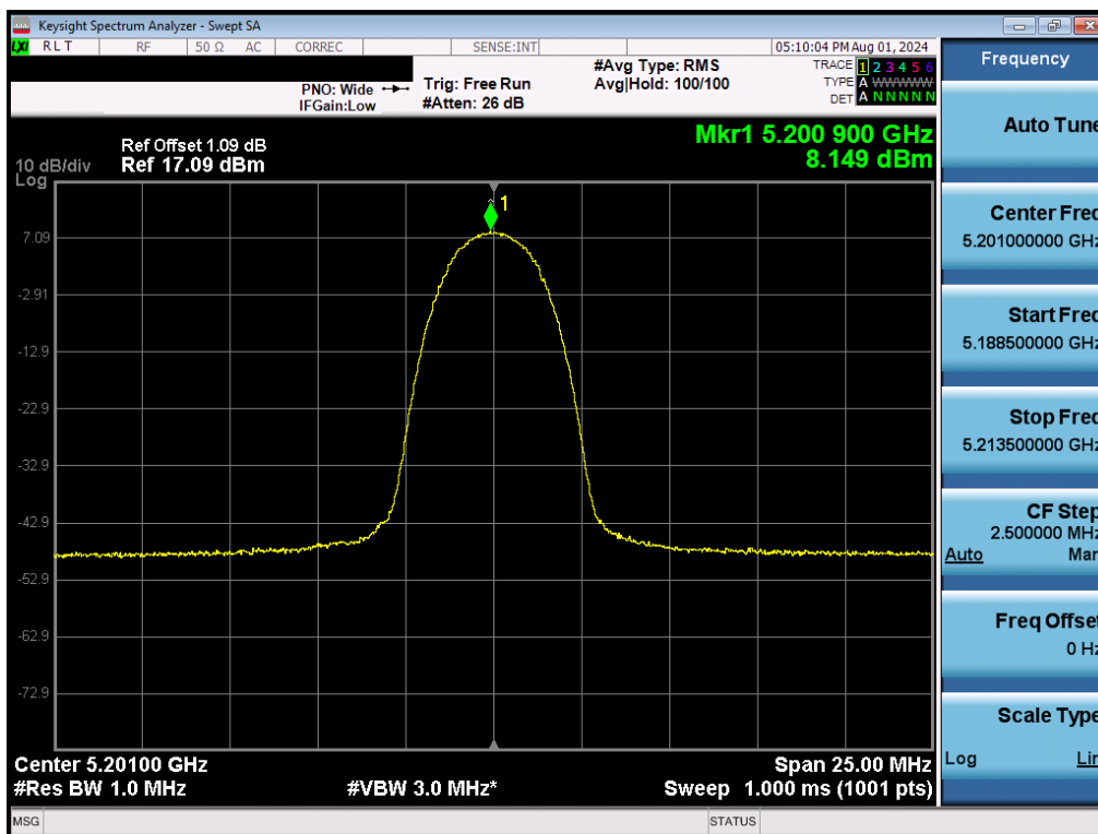
Plot 7-44. FCC PSD (NB UNII HDR4 – 5201MHz)
