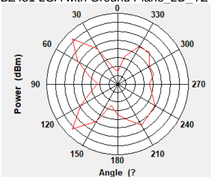
WBZ451 LGA with Ground Plane_2D_YZ-Cut
