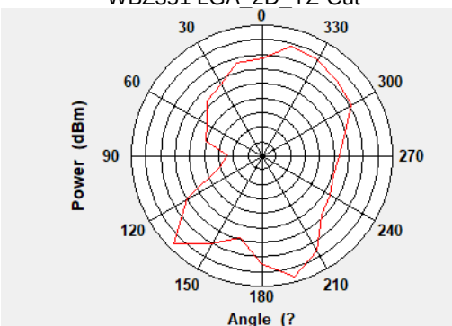
WBZ351 LGA_2D_YZ-Cut
