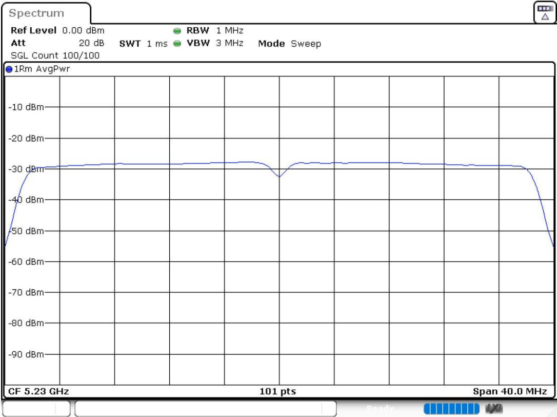
PSD Chain 1
