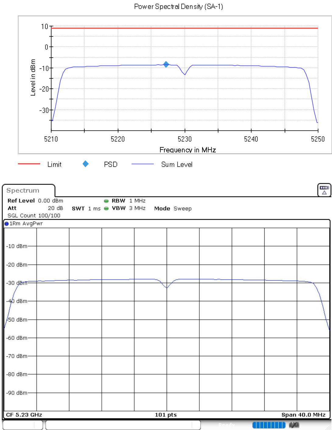
PSD Chain 1
