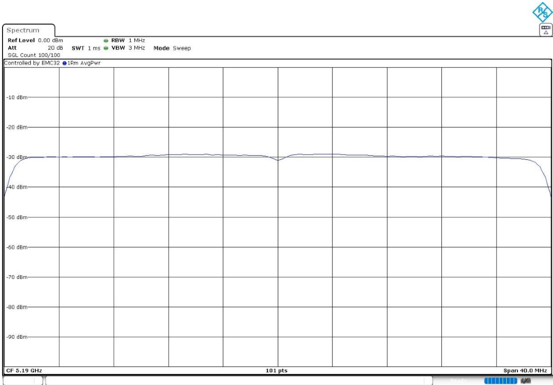
PSD Chain 1
