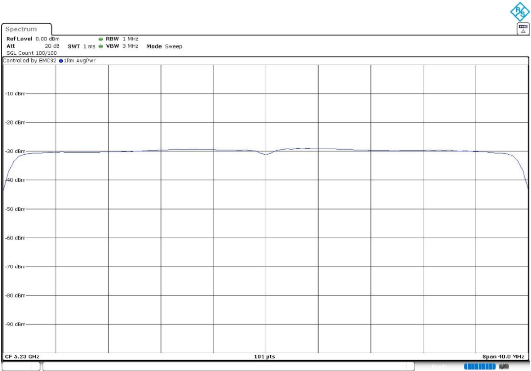
PSD Chain 1
