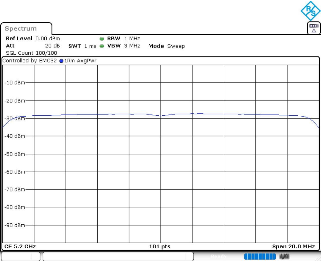
PSD Chain 0
