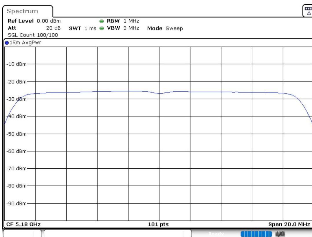
PSD Chain 1
