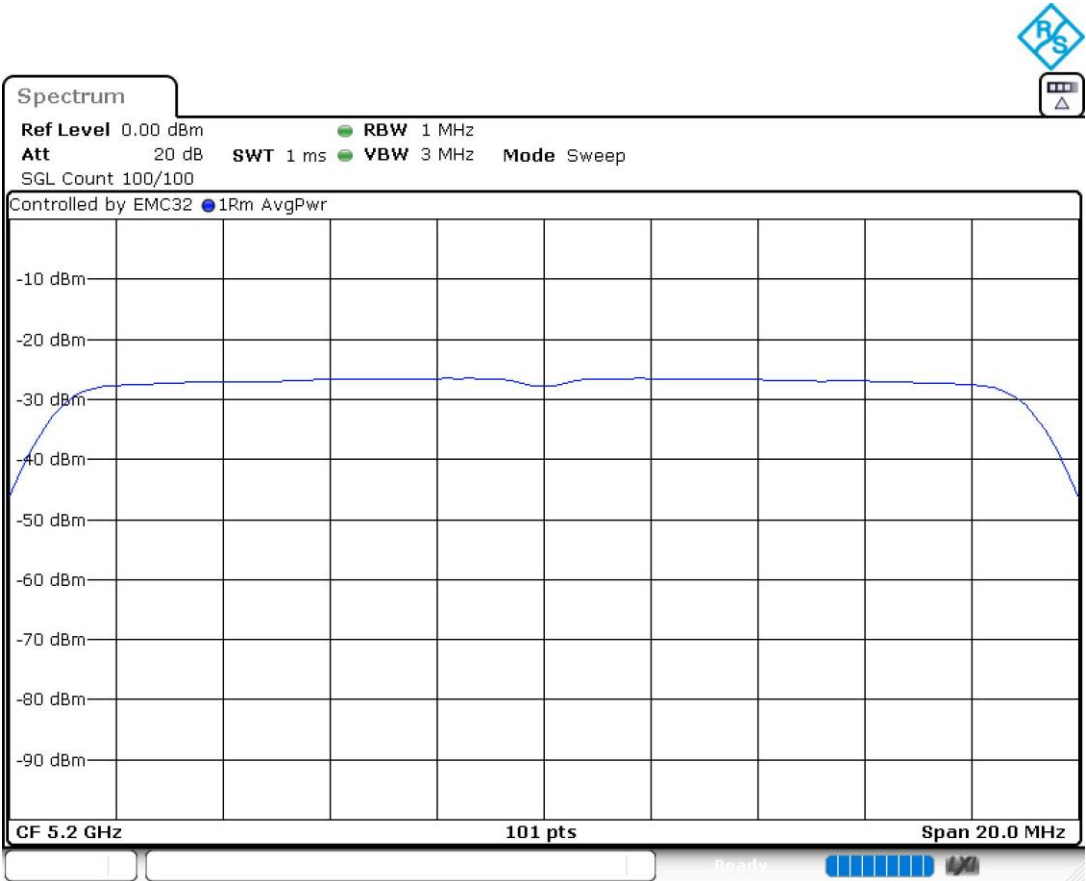
PSD Chain 1
