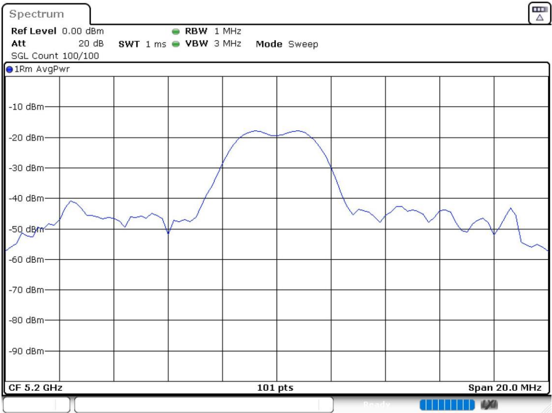
PSD Chain 1
