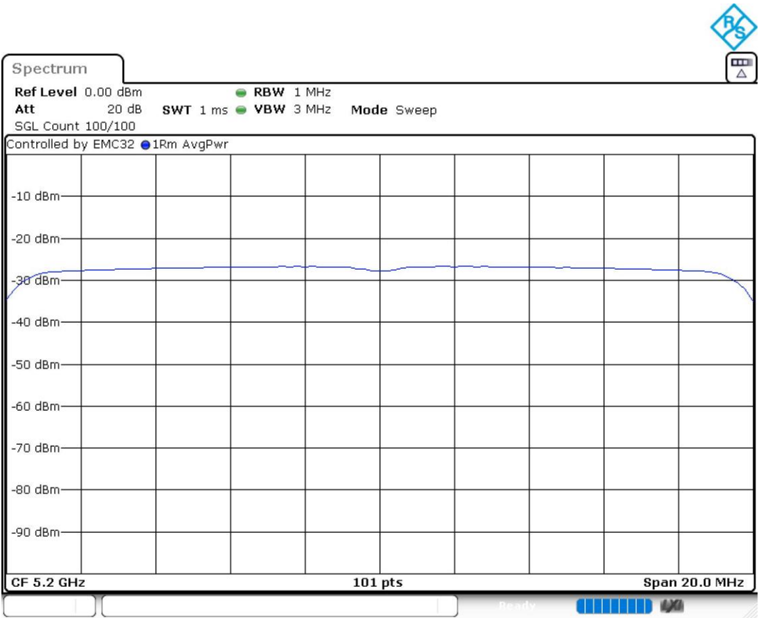
PSD Chain 1
