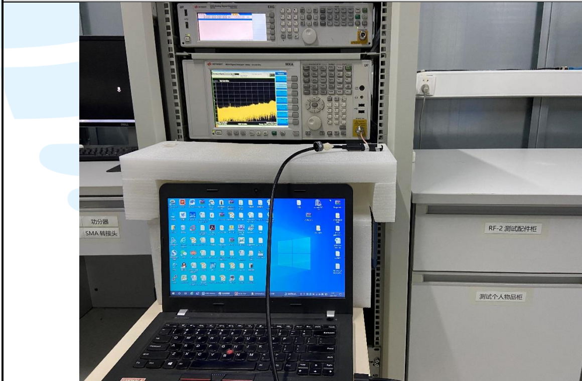
Conducted RF Test Setup
