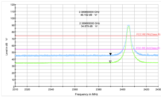
ZigBee-Channel 11: Peak + Average
