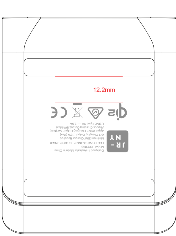
BASE VIEW
