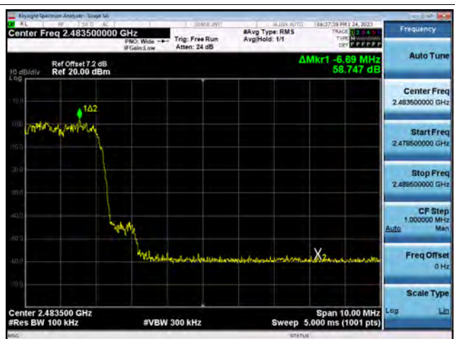
\pi/4 DQPSK (with hopping) Band Edge(CH.78)
