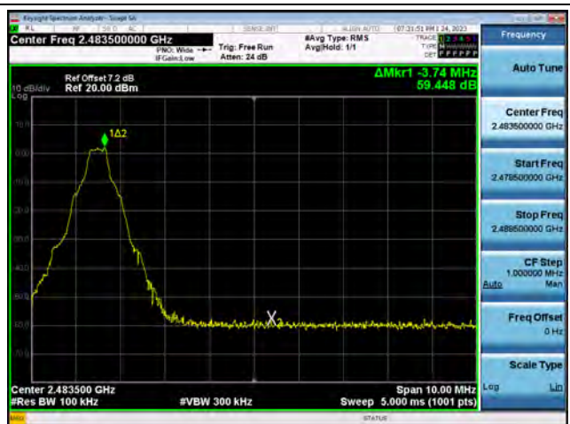
8DPSK(without hopping) Band Edge(CH.78)
