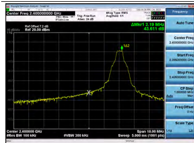
8DPSK(without hopping) Band Edge(CH.0)
