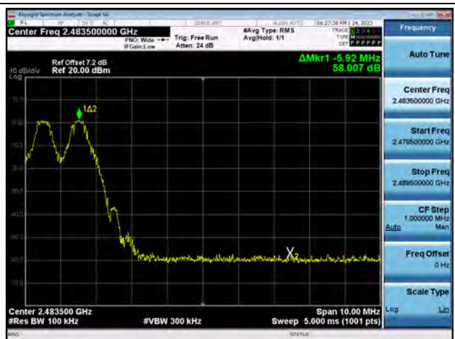
8DPSK(with hopping) Band Edge(CH.78)
