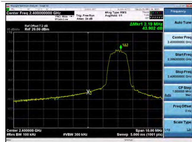
\pi/4 DQPSK(without hopping) Band Edge(CH.0)
