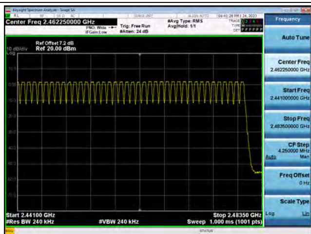
8DPSK Number of Channels (2.441 GHz - 2.483.5 GHz)
