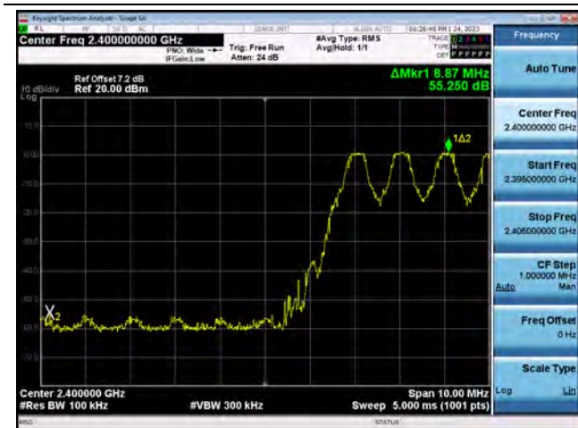
8DPSK(with hopping) Band Edge(CH.0)
