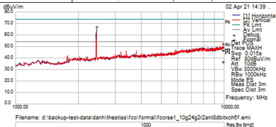
TX Spurious Emissions from 1GHz-10GHz – Ch6 (2437 MHz)
