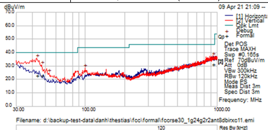
Title: TX Spurious Emissions from 30MHz-1GHz – Ch11 (2462 MHz)
