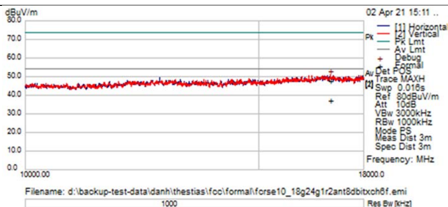
TX Spurious Emissions from 10GHz-18GHz – Ch6 (2437 MHz)
