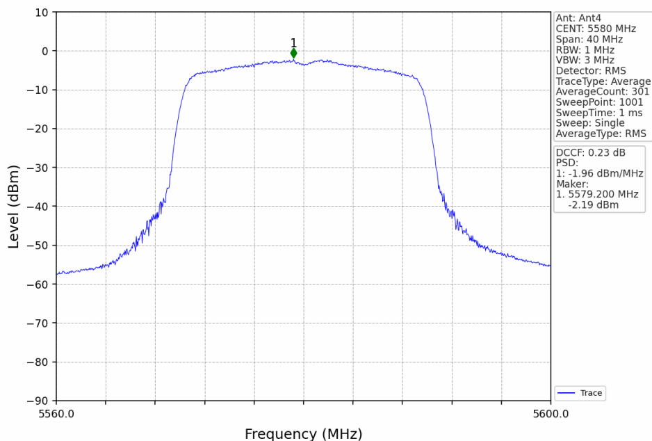
802.11ax(HEW20)_MCH_5580MHz_RU242_Left_Ant4_NTNV
