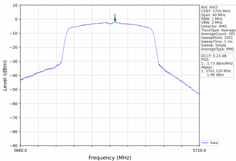
802.11ax(HEW20)_HCH_5700MHz_RU242_Left_Ant3_NTNV
