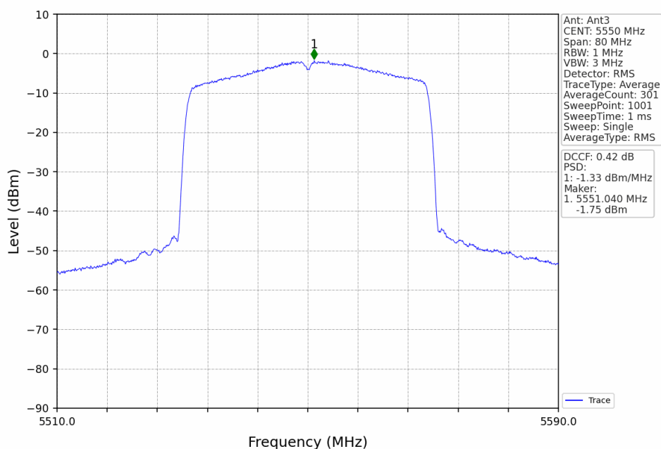
802.11ax(HEW40)_MCH_5550MHz_RU484_Left_Ant3_NTNV
