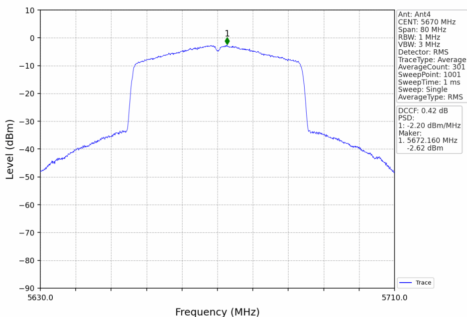
802.11ax(HEW40)_HCH_5670MHz_RU484_Left_Ant4_NTNV
