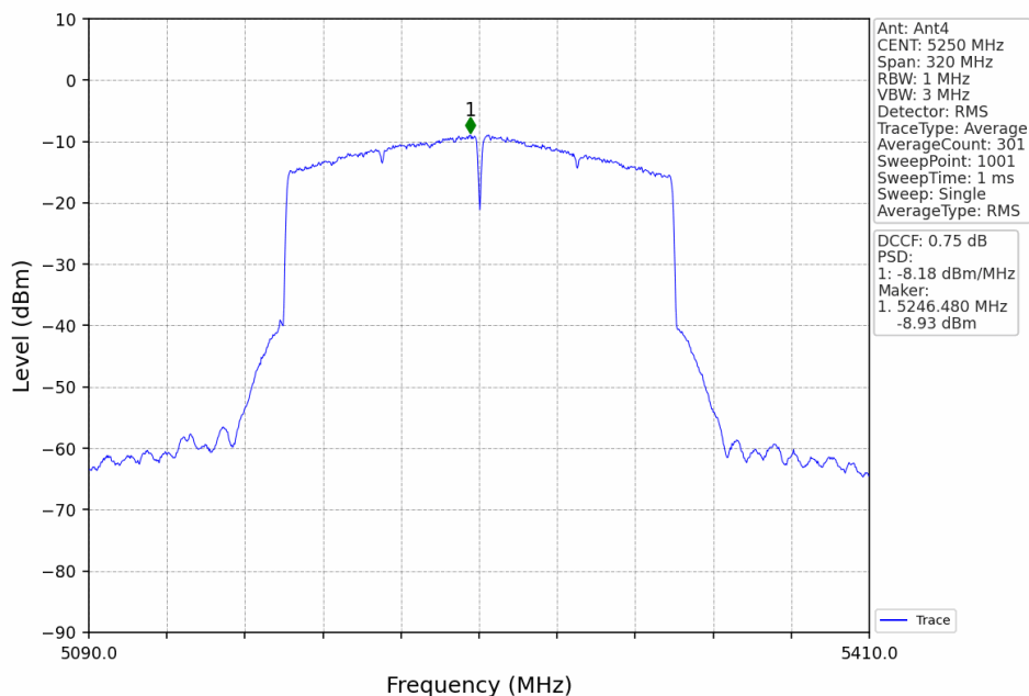
802.11ax(HEW160)_MCH_5250MHz_2xRU996_Left_Ant4_NTNV
