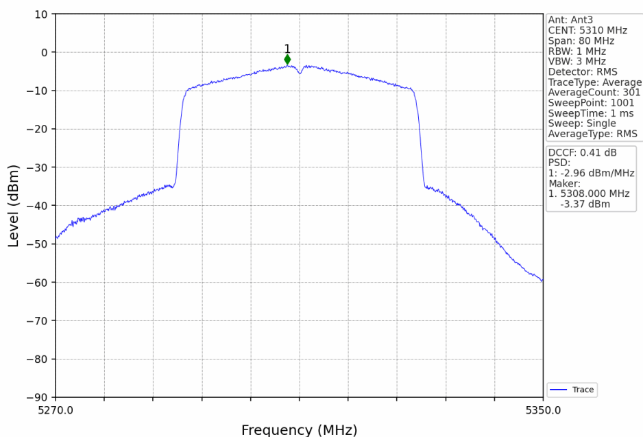
802.11ax(HEW40)_HCH_5310MHz_RU484_Left_Ant3_NTNV
