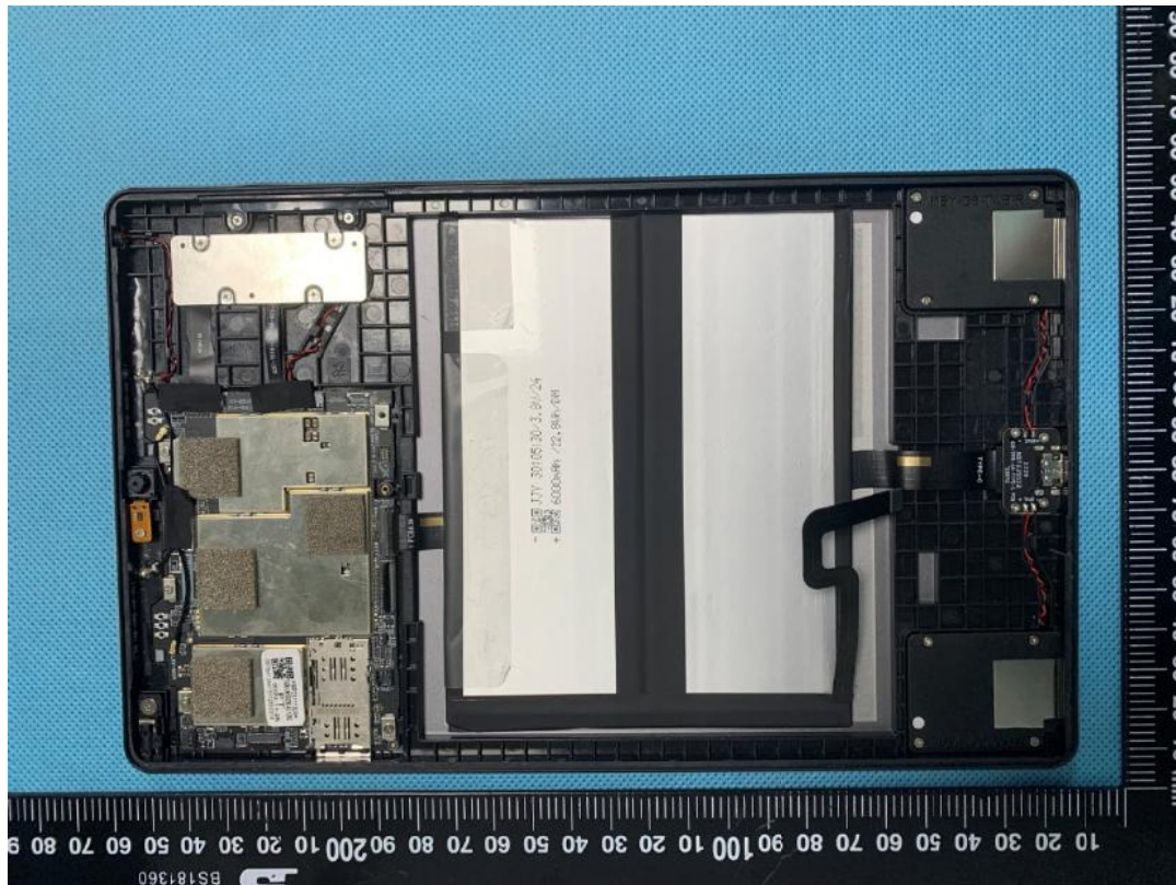
BT/WI-Fi ANT
