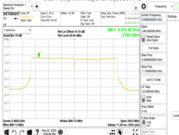
802.11be_160MHz_Chain0_6985MHz_996+484+242_MRU2
