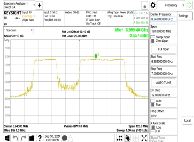
802.11be_80MHz_Chain1_6945MHz_484+242_MRU2
