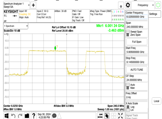
802.11be_160MHz_Chain0_6025MHz_996+484+242_MR2
