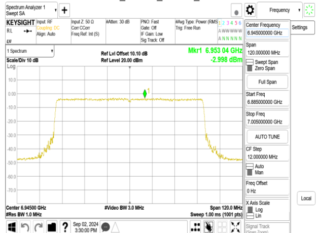
802.11be_80MHz_Chain0_6945MHz_484+242_MR2
