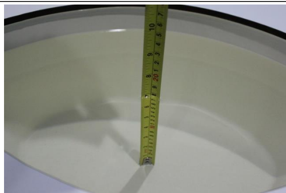
Liquid depth in the body phantom (5200MHz)
