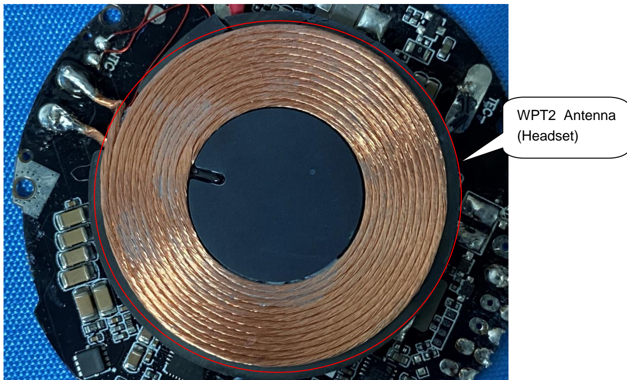
INTERNAL VIEW OF EUT (FIGURE 8)
