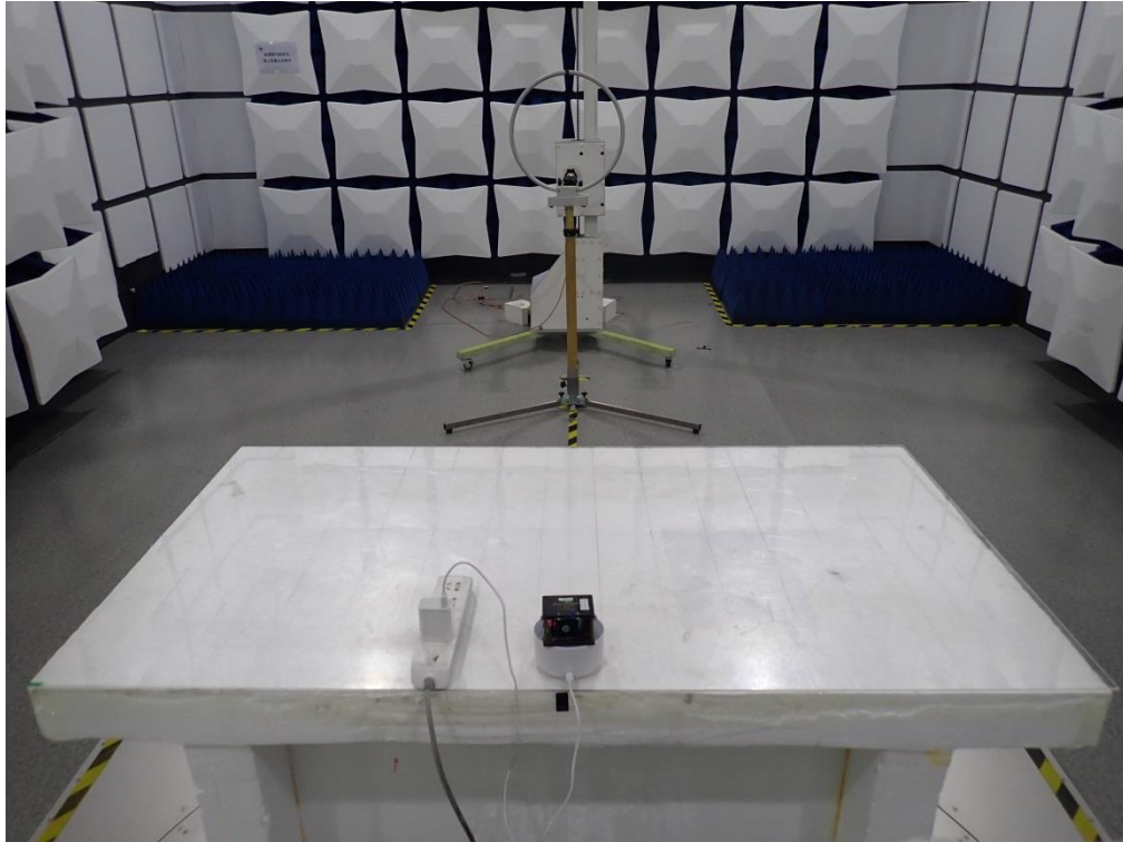
WPT Radiated Emission Below 30MHz
