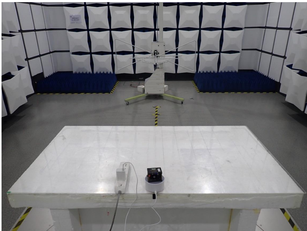
WPT Radiated Emission Below 1GHz
