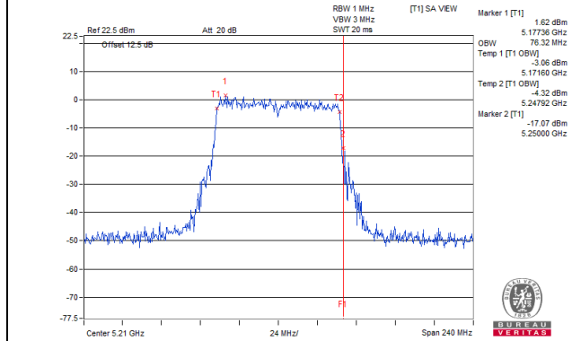
802.11ac (VHT80)_Chain 3 / CH42
