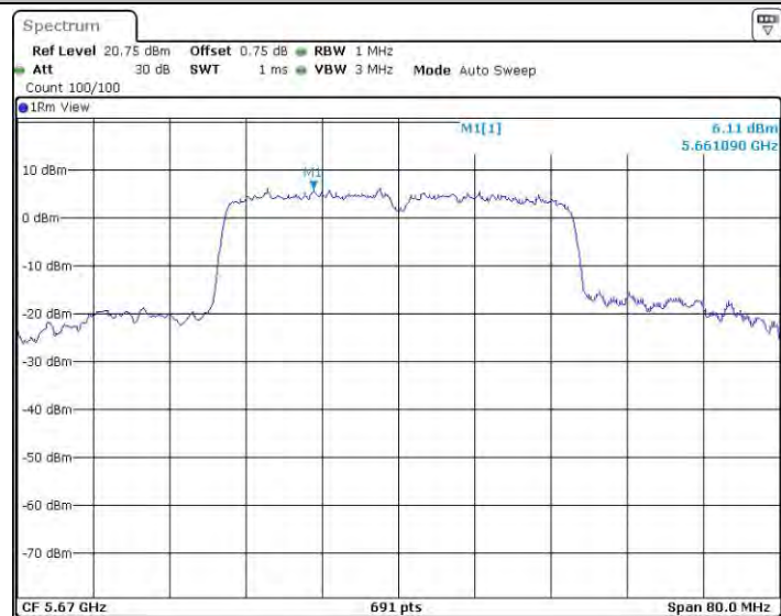
11N40SISO_Ant1_5670
