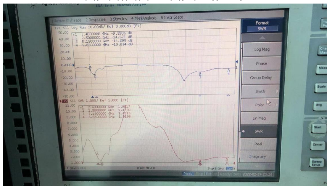
A antenna: dual-band WIFI antenna L=100mm VSWR
