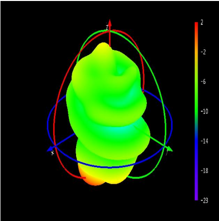
Phi=90 freq=2440MHz
