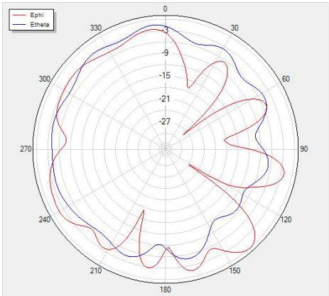
Phi=90 freq=2440MHz
