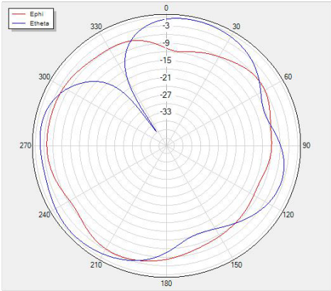
Phi=0 freq=2440MHz
