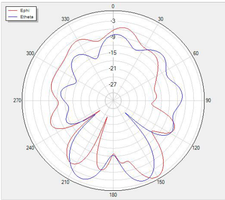
Phi=0 freq=2440MHz
