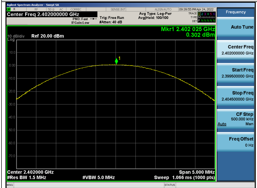
Test_Graph_EDR_ANT1_2402_3Mbps_Peak Power
