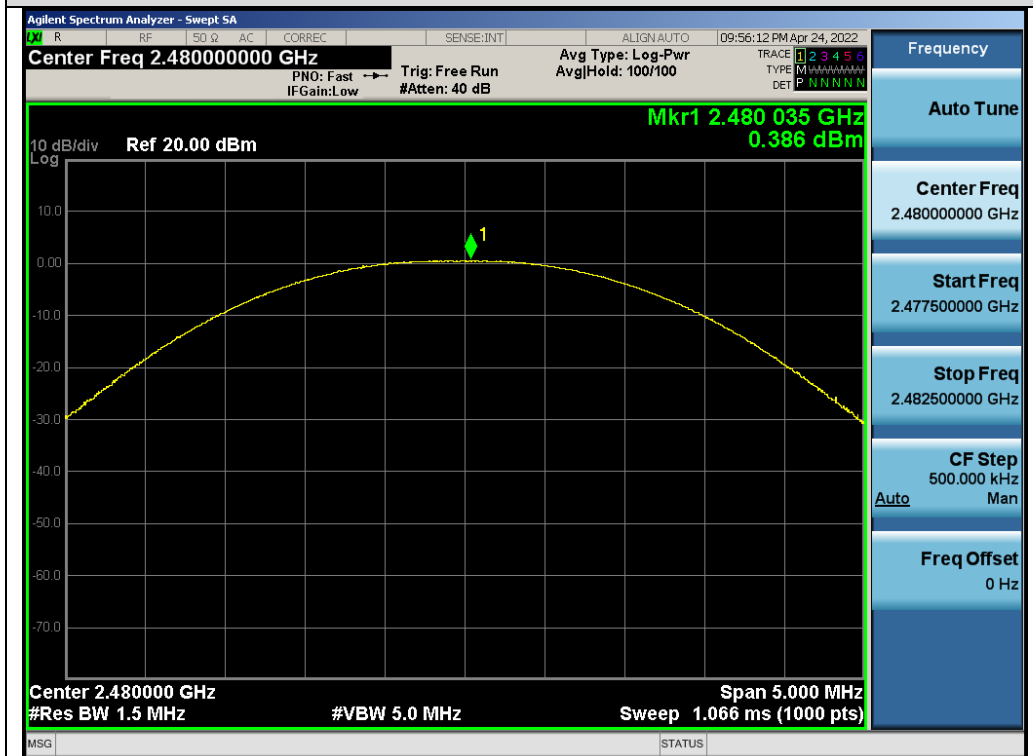
Test_Graph_BR_ANT1_2480_1Mbps_Peak Power
