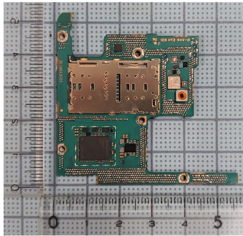
Internal Main-PWB Rear without Shield cases (Front-side)
