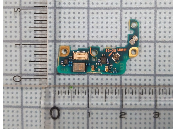
Internal Sub-PBA (Rear-side)
