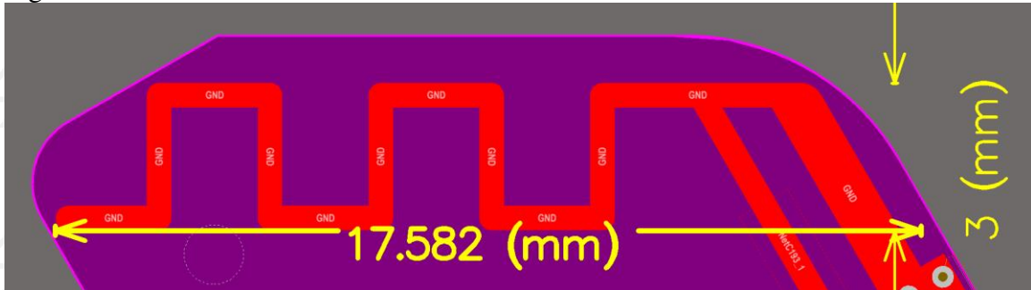
Fig.1: The dimension of the PCB Antenna
