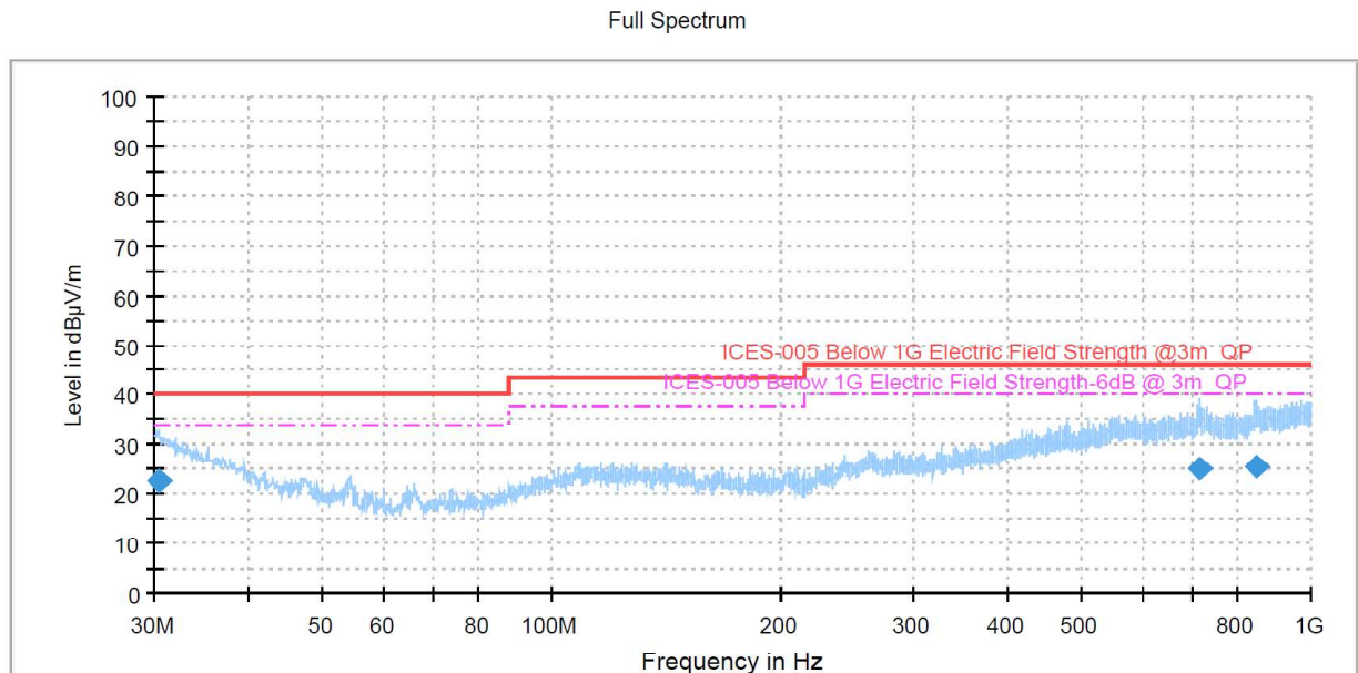
Figure 4: Spectral Diagrams, Radiated Emission, 30MHz-1000MHz, Vertical polarization
