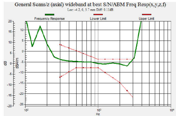
Fig 7.2 GSM1900 Ch661
