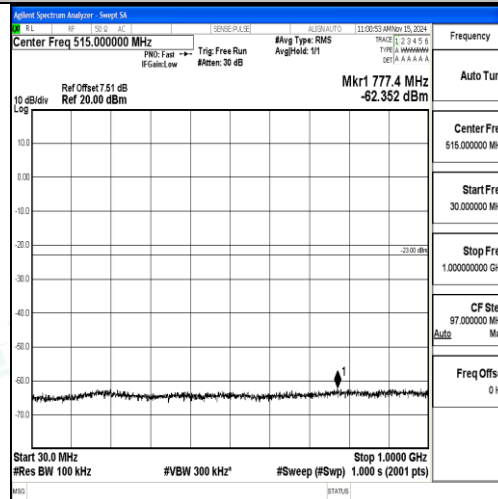
Band2_15MHz_16QAM_18675_1RB#0_30~1000_30~1000
