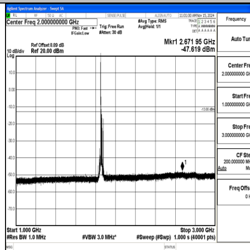
Band2_15MHz_16QAM_18675_1RB#0_1000~3000_1000~3000
