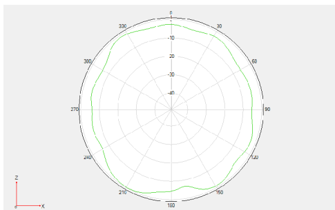
Phi =0 freq=2500MHz
