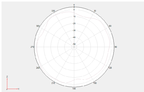
Phi =90 freq=2450MHz
