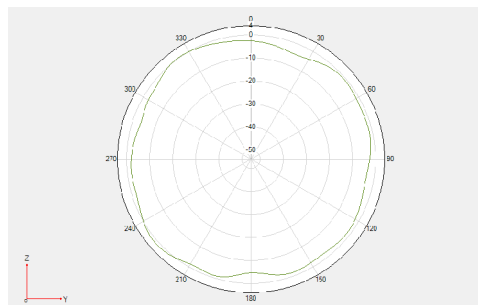
Phi =90 freq=2500MHz
