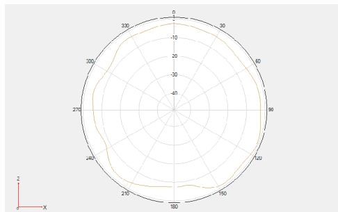
Phi =0 freq=2400MHz
