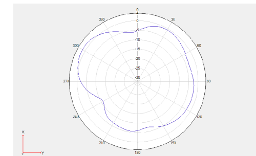
Theta =90 freq=2500MHz
