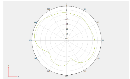
Theta =90 freq=2450MHz
