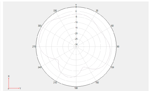
Theta =90 freq=2400MHz
