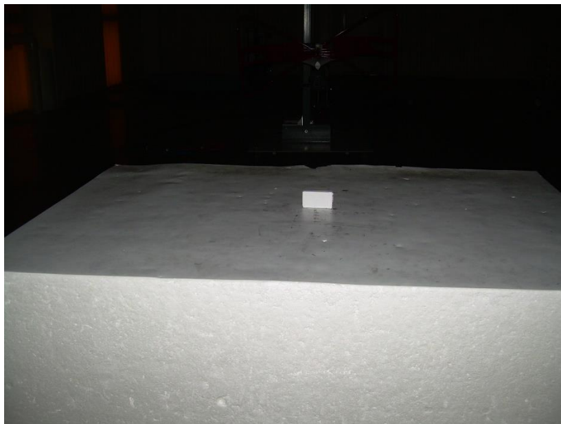
Photograph 2: Back View Radiated Emissions Worst-Case Configuration – 30 to 1000 MHz
