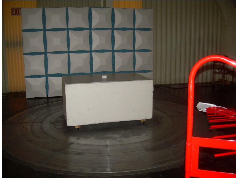
Photograph 1: Front View Radiated Emissions Worst-Case Configuration – 30 to 1000 MHz
