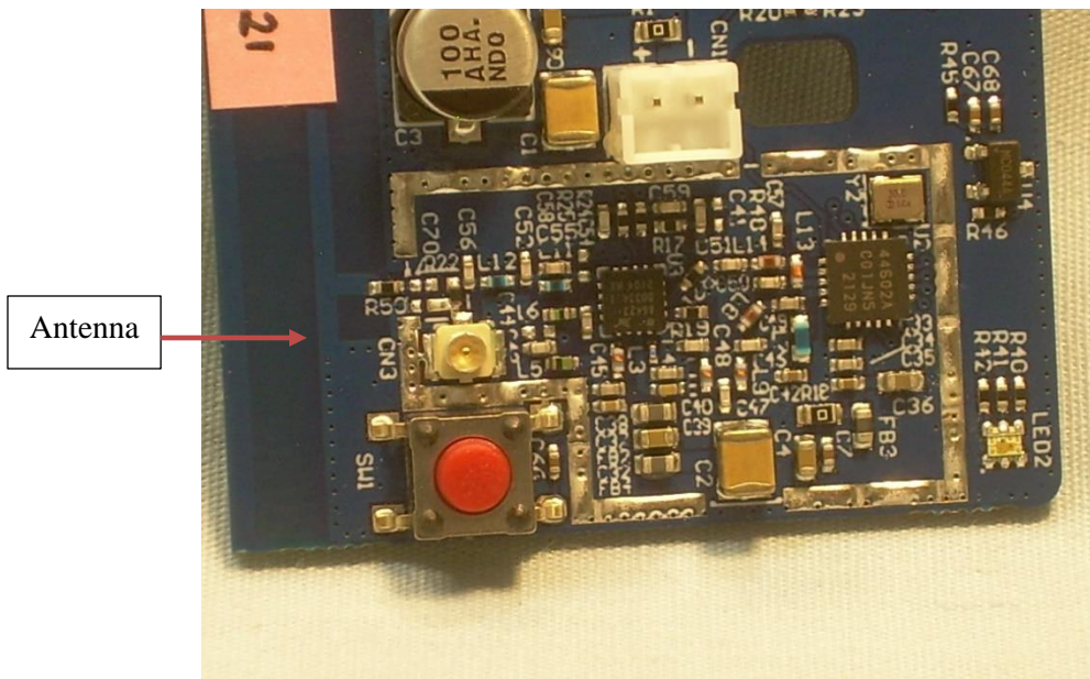
Photograph 15: View of the Circuitry Under the RF Shield
