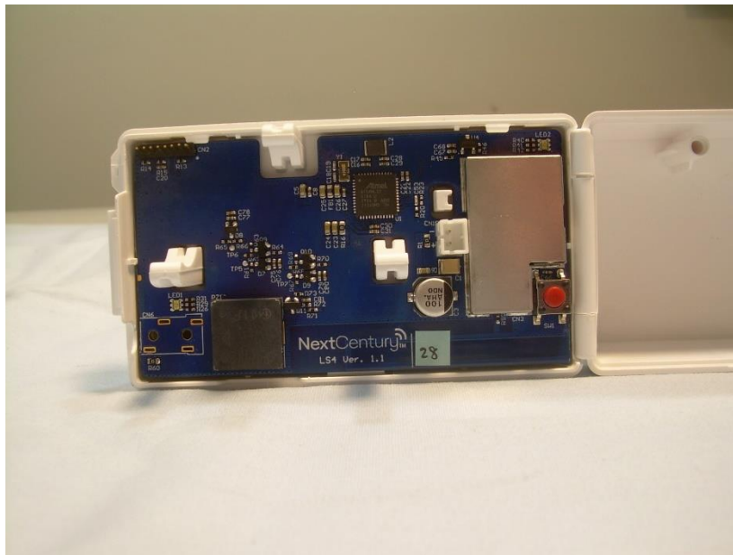
Photograph 12: PCB in Housing
