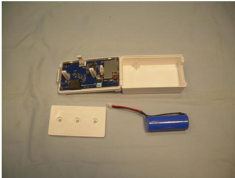
Photograph 11: Housing Open Showing PCB in Housing, Wall Mounting Plate, and Battery
