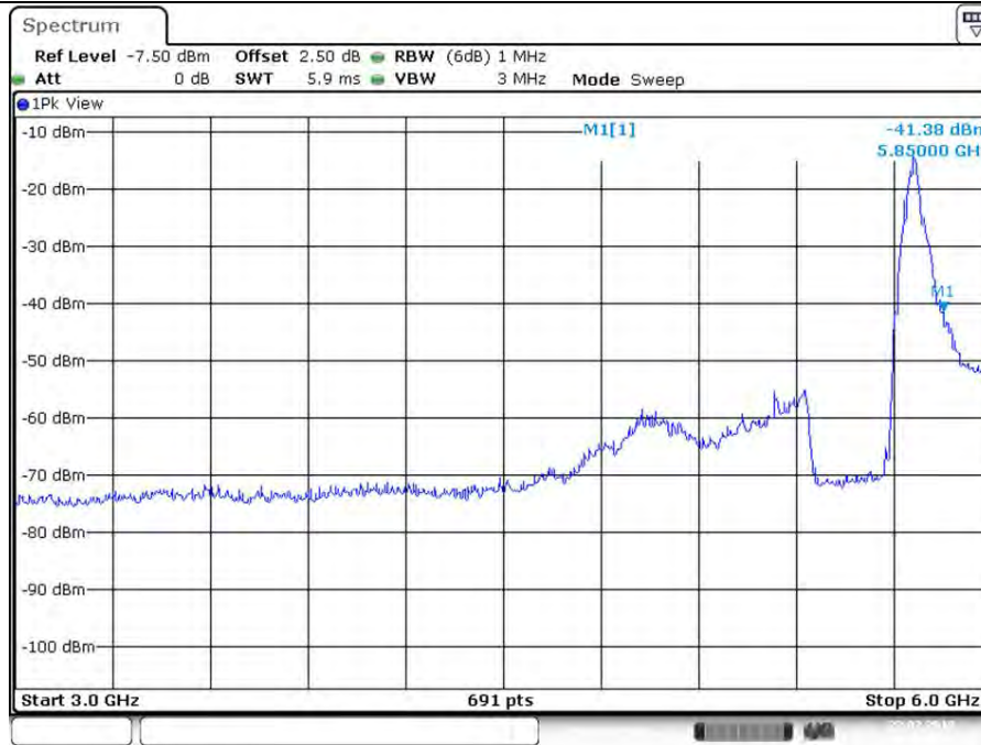
Plot on Configuration VHT20 / 5720 MHz / Peak / Port 1 / 3GHz~6GHz
