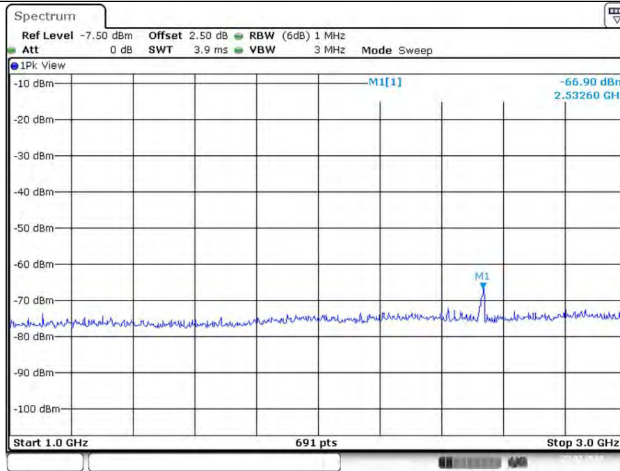
Plot on Configuration VHT20 / 5500 MHz / Peak / Port 1 / 1GHz~3GHz
