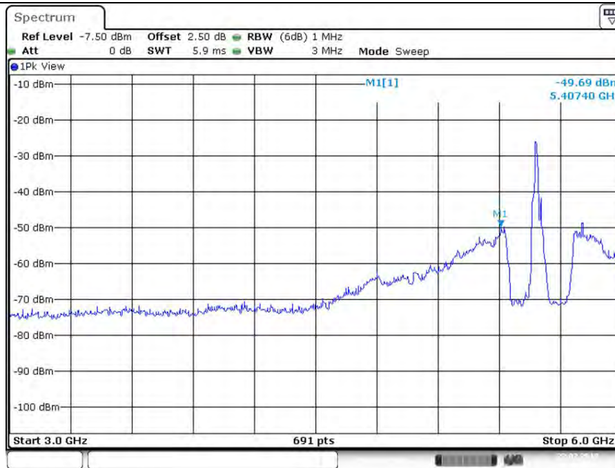
Plot on Configuration VHT20 / 5580 MHz / Peak / Port 2 / 3GHz~6GHz
