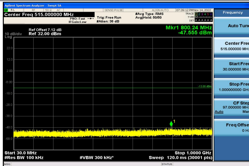
Band4-5MHz-16QAM-20175-1RB#0-30~1000MHz
