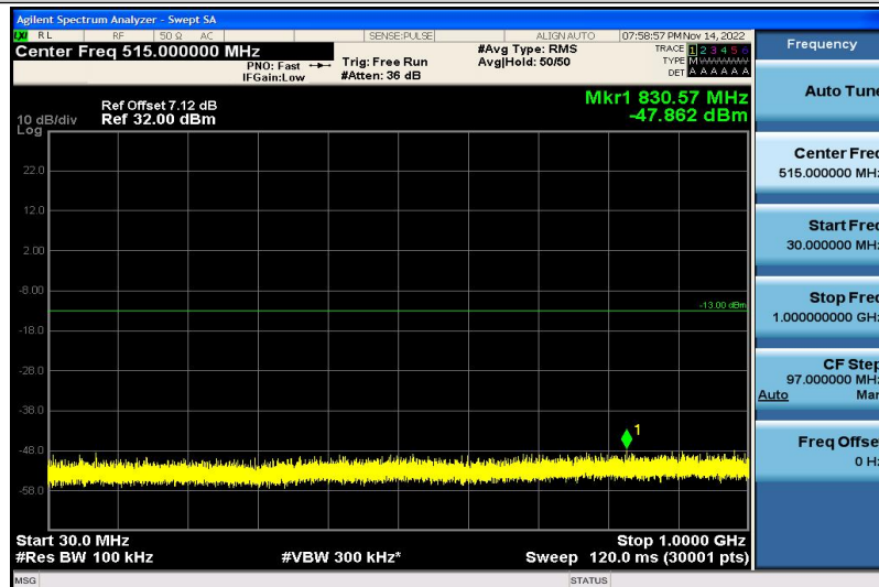
Band4-10MHz-QPSK-20175-1RB#0-30~1000MHz
