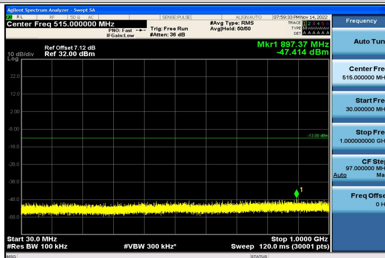
Band4-10MHz-16QAM-20175-1RB#0-30~1000MHz
