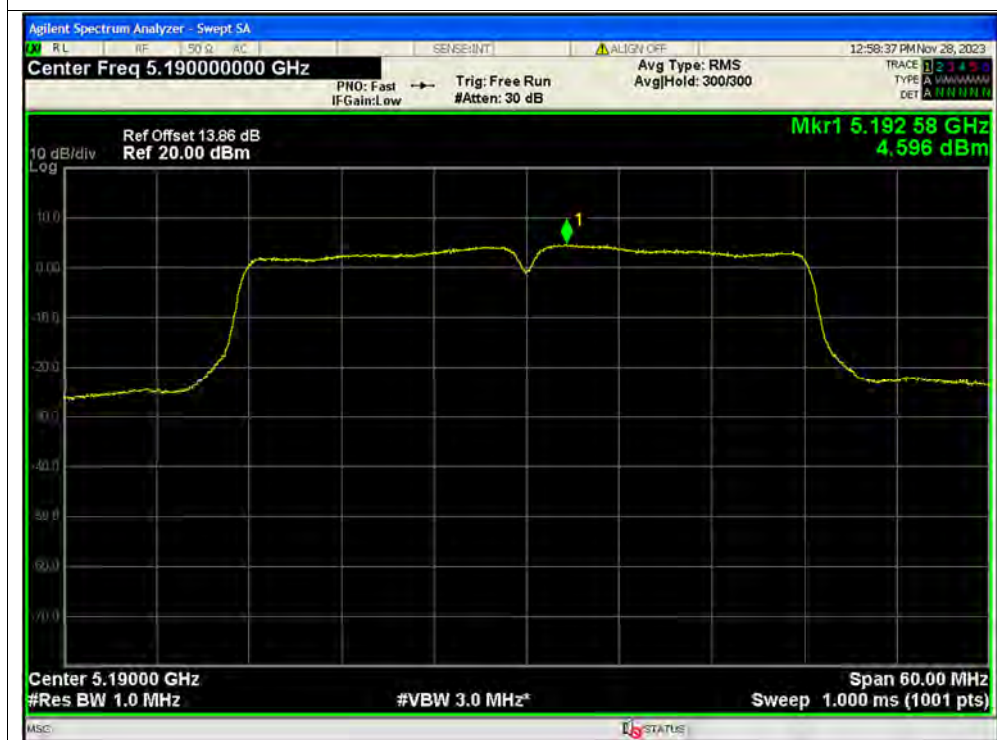
PSD NVNT n40 5190MHz Ant2 MIMO
