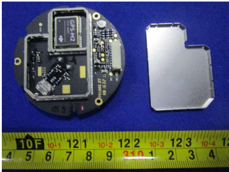
EUT –GPS Module Bottom Uncover View
