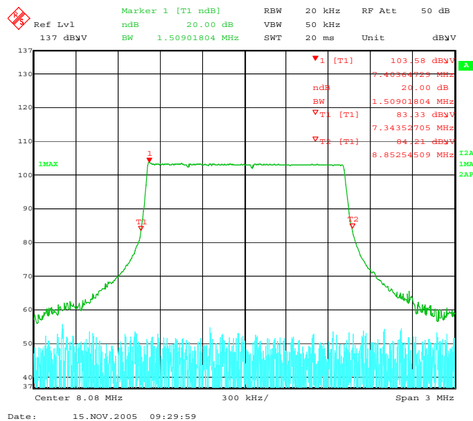
20 dB Bandwidth
